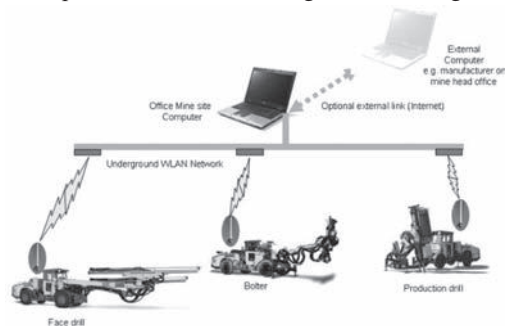
Figure 2. Rig remote access system (photo supplied by Atlas Copco).
