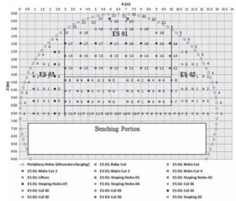
Figure 6. Design of the tunnel blast.
