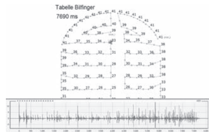
Figure 19. Using SHOTplus-T and the NCVIB system to compare the recorded waveform with the initiation sequence.
