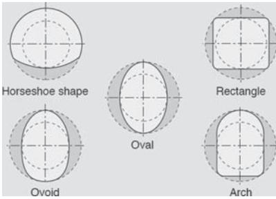
Figure 10. Typical tunnel cross-sections.
