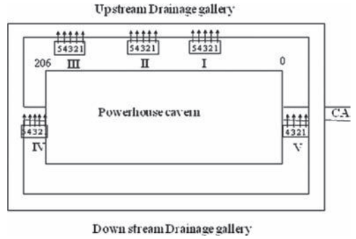
Figure 4. Location of vibration monitoring stations.
