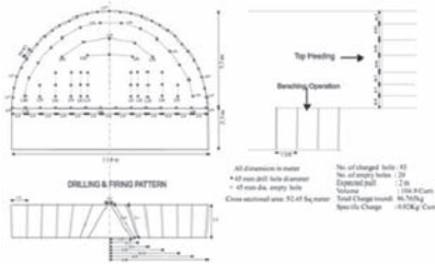
Figure 3. Drilling, charging & firing patterns of holes in heading, widening & benching portion.
