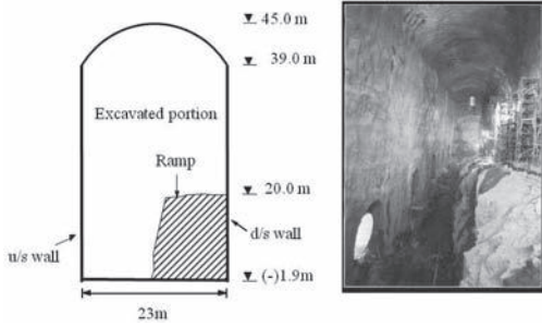
Figure 1. Position of the ramp and view of the underground power house cavern before excavation of the ramp.
