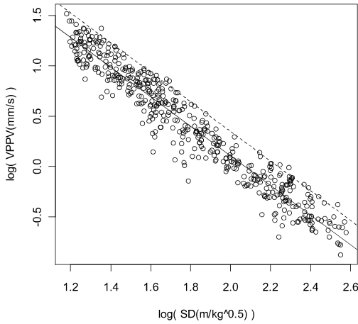
Figure 8. Combined vibration data with linear regression fit to transformed data plus a line estimated from the mean standard error of the residuals at a 95% confidence level.
