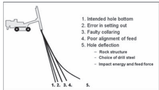
Figure 2. Factors that effects the drilling precision.
