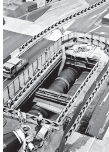
Figure 11. The twin storm water diversion pipes (aerial view).
