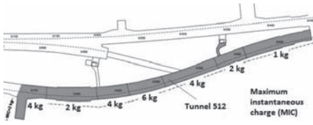
Figure 8. Instantaneous charge weight restrictions in tunnel 512.
