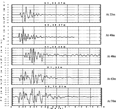
Figure 7. Waveform changes at different distance from a signature hole in the hard granite of the site.
