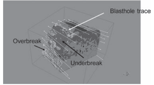
Figure 12. Boolean operation for as-drilled and as-blasted rounds (a) the as-drilled round formed by joining adjacent perimeter blastholes (b) overlay of the as-blasted round on the as-drilled round with some underbreak and overbreak areas indicated.
