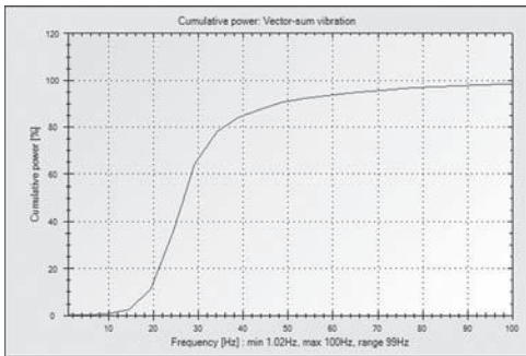
Figure 12. Percent cumulative power for the vibration recorded nearest a 1657 gram charge in Plunkett Street.
