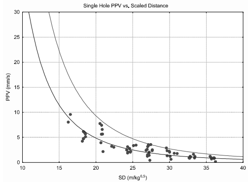
Figure 8. The regression of the cut hole vibration the parameters of which are input to MSW model.
