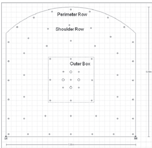
Figure 5. Face pattern showing areas of drilling.
