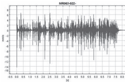
Figure 17. NCVIB: Example of blast vibration time history.
