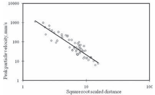
Figure 5. Peak particle velocity versus scaled distance.
