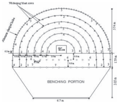
Figure 14. Sequences of excavation, drilling, firing and charging pattern of holes during hot temperature zone.
