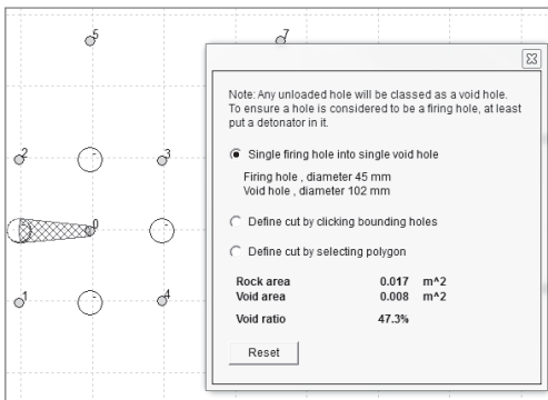
Figure 2. Burn cut design on 300 mm grid showing void ratio.
