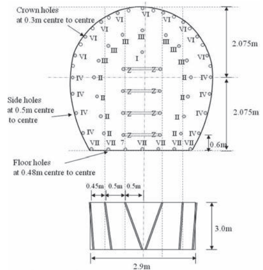
Figure Not to Scale Use long electric delay detonators Alternate holes in the perimeter only to be charged
