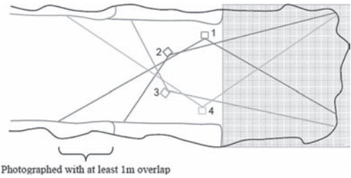
Figure 3. Four images are taken at each of the four numbered locations. These sixteen images are processed using the processing algorithm to produce the 3D point cloud (after Birch 2008).
