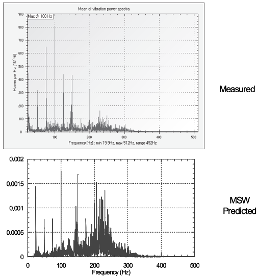
Figure 10. Comparison between the measured power spectrum and the predicted spectrum.
