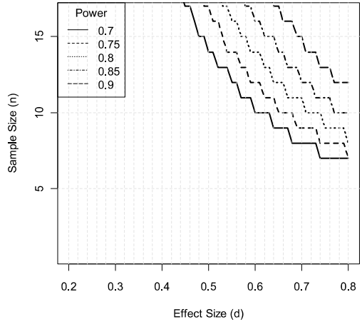
Figure A3. Sample size for significance level of 0.2.
