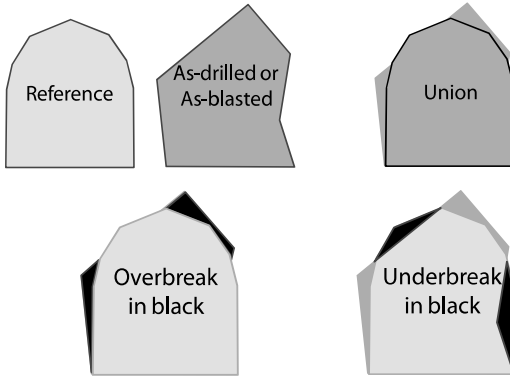
Figure 11. Boolean operations in 2D (a) approximate horseshoe profile is the reference object and the irregular polygon is the as-drilled round or as-blasted round. (b) Union of the reference object and the as-drilled or as-blasted object (c) Union minus the reference object gives the overbreak (in black) (d) Union minus the as-drilled or as-blasted object gives the underbreak (in black). Typically the reference object is either the as-designed round or the as-drilled round.
