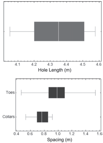
Figure 9. Drilling accuracy (a) Hole length box-whisker plot (b) Collar and toe spacing box-whisker plots (Spathis et al. 2009).
