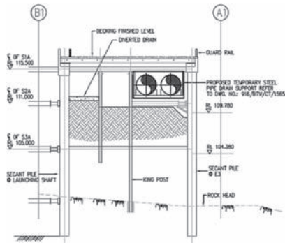
Figure 10. Section view of the shaft.
