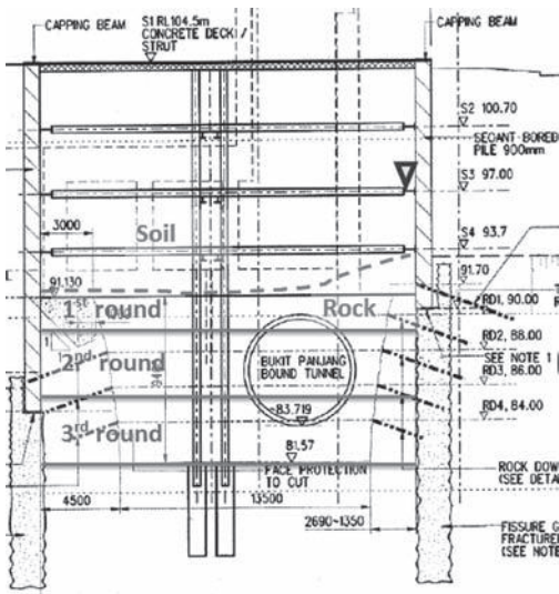
Figure 4. Section view of the shaft.
