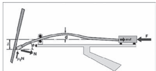
Figure 6. Drill hole deviation during drilling.
