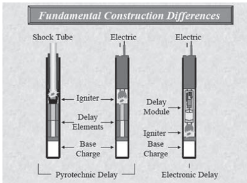
Figure 5. Construction of Electric, Shock-tube & Electronic Detonators © IME 2002.
