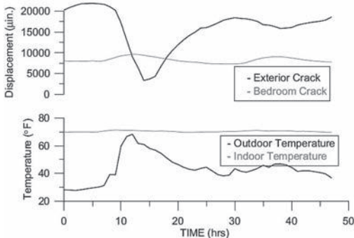
Figure 5. Response of crack with change in temperature (Dowding and McKenna, 2005).
