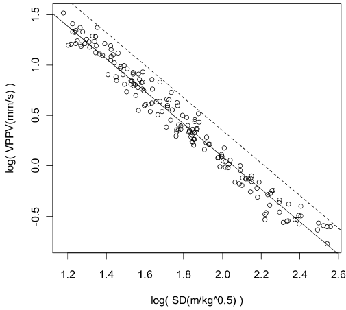
Figure 6. Plunkett Street vibration data with linear regression fit to transformed data plus a line estimated from the mean standard error of the residuals at a 95% confidence level.
