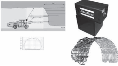
Figure 3. Tunnel Profiler (photo supplied by Atlas Copco).
