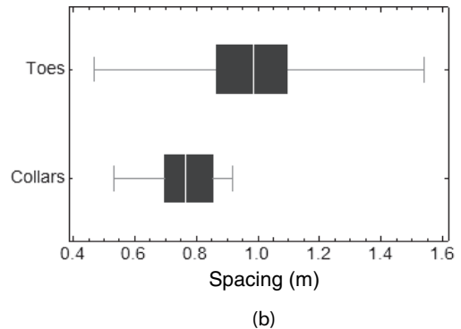
Figure 8. Drilling accuracy of collar and toe spacing box-whisker plots (Spathis et al. 2009).
