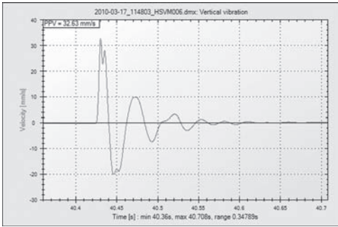
Figure 10. Vertical component of the vibration recorded at the nearest site to a 1657 gram charge fired in Plunkett Street.
