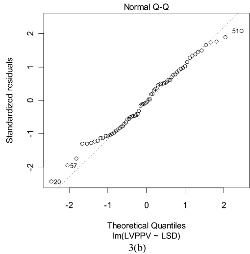
Figure 3. Thorpe Street (a) Plot of the residuals of the fit versus the fitted points (b) Probability plot for the regression fit.
