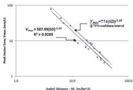
Figure 3. Vibration attenuation equation for the trial blasts.
