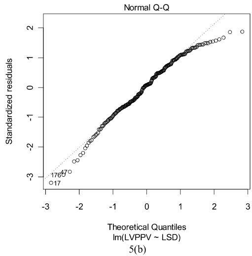
Figure 5. Hume Street (a) Plot of the residuals of the fit versus the fitted points (b) Probability plot for the regression fit.
