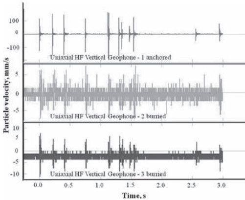
Figure 3. Signals obtained by different methods of coupling.
