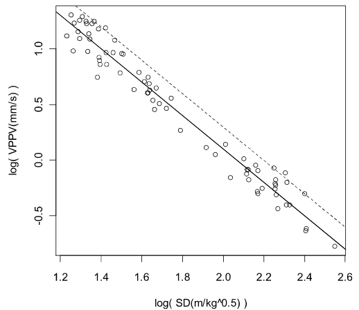
Figure 2. Thorpe Street vibration data with linear regression fit to transformed data. The dashed line is estimated from the mean standard error of the residuals at a 95% confidence level.
