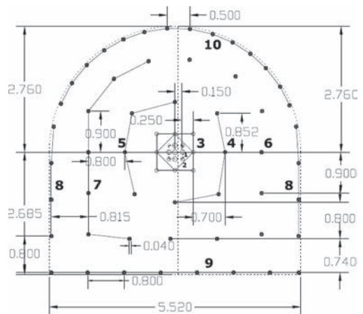
Figure 4. Blast design used in the excavation of HR tunnel.
