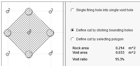
Figure 1. Burn cut showing meaningless void calculation.
