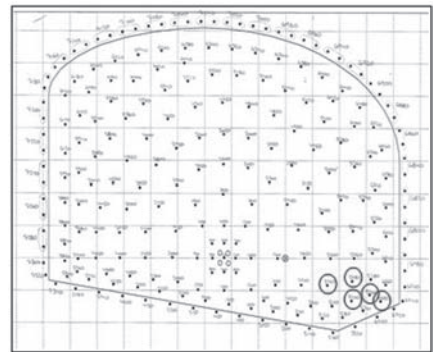
Figure 7. Correlating PPVs with shotholes the blast plan.
