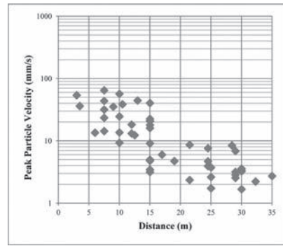
Figure 8. Recorded PPV values.
