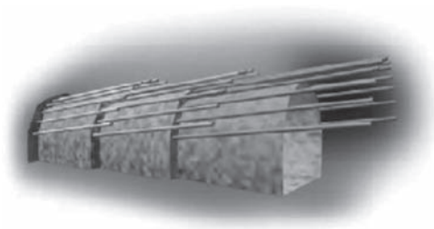
Figure 4. 3D view of pipe forepoling.
