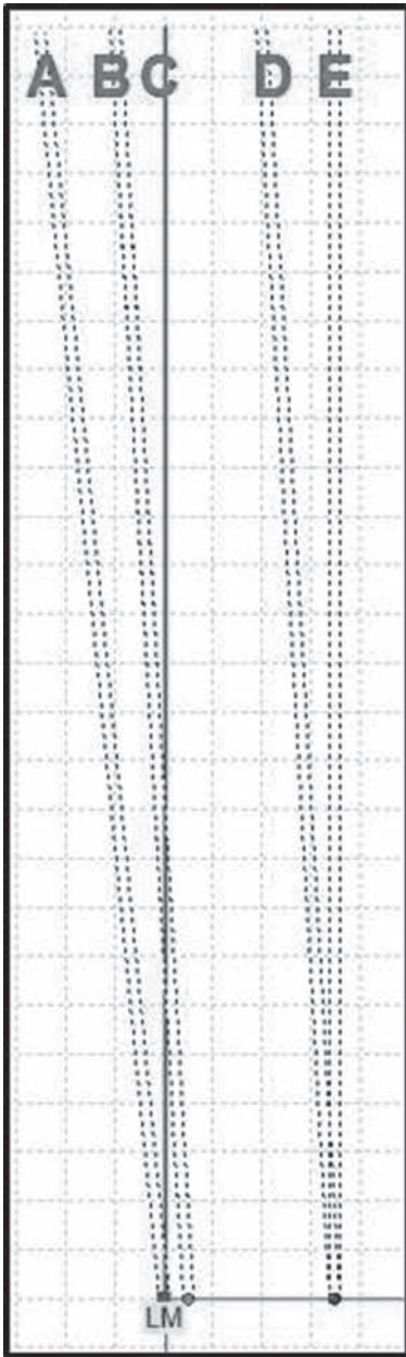
Figure 4. Plan of perimeter drill options on a 5.2 m round.
