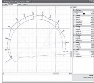
Figure 14. Section of scanned tunnel profile.
