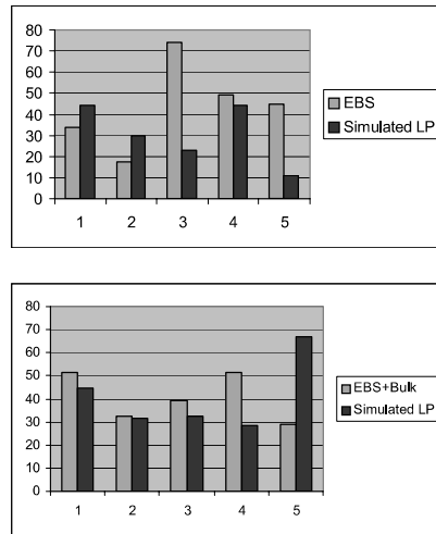
Figure 13. Randomised paired comparisons (a) effect of precise timing (b) effect of precise, faster timing and bulk emulsions (after Spathis et al. 2006).
