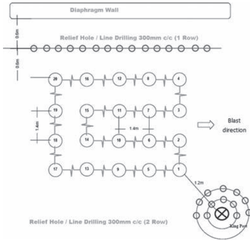
Figure 5. Typical blast design pattern.
