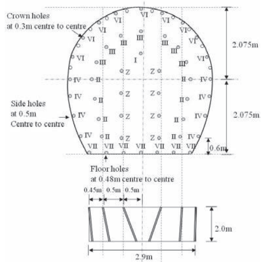
Figure Not to Scale Use long electric delay detonators. Alternate holes in the perimeter only to be charged. If the rock condition is very poor, one hole can be charged leaving two uncharged holes in the perimeter. If the rock condition is improved, the design suggested for face 1 can be followed for face 2 also.
