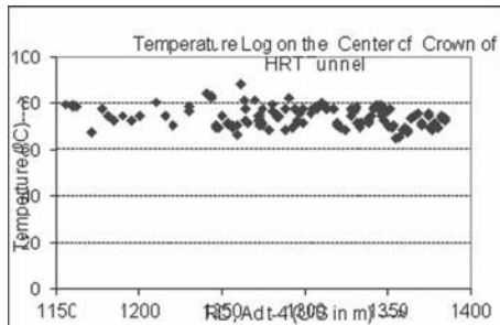
Figure 15. Temperature log recorded at different Reduced Distance (RD) in HRT, KWHEP.
