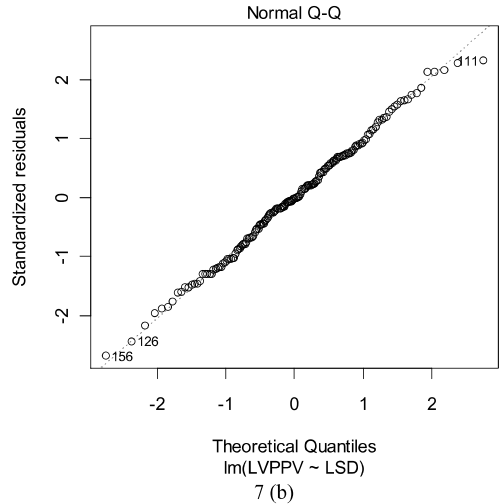
Figure 7. Plunkett Street (a) Plot of the residuals of the fit versus the fitted points (b) Probability plot for the regression fit.
