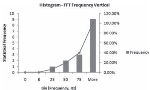
Figure 4. Dominant frequency of the vibrations.
