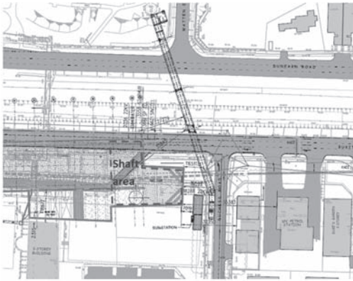
Figure 3. Plan view of Tan Tah Kee TBM launching shaft.
