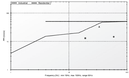
Figure 13. Plot of the component vibrations (□ transverse, ▲ vertical, ● radial) obtained for the largest vibration recorded nearest a 1657 gram charge in Plunkett Street. The threshold lines are those taken from the relevant British Standard and referred to in AS 2187-2006.
