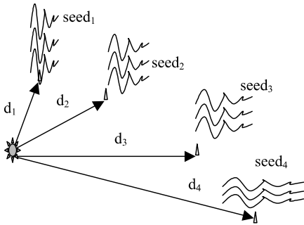
Figure 1. A sketch of multiple sets of seed waveforms measured at different distances from a signature hole.
