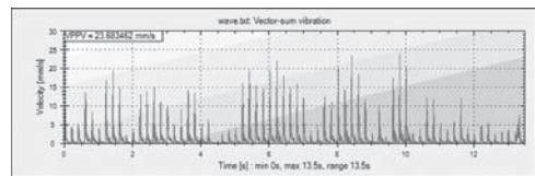
Figure 15. The first predicted waveform produced by the uncalibrated model for design 8 at Plunkett St. Minimal interference can be observed. 200 ms delay between production holes.
