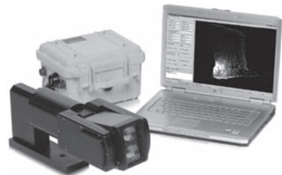
Figure 2. Optech laser scanning head (foreground).
