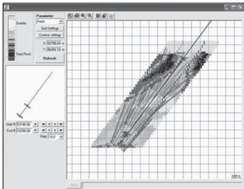
Figure 10. Tunnel mapping of a 50 m section in a subway tunneling project, including four injection.
