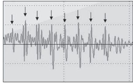
Figure 6. Waveform showing individual shotholes detonating.
