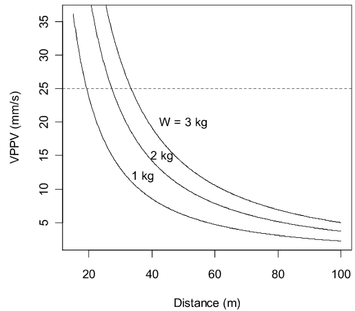
Figure 14. Vector peak particle velocity versus distance for a charge weight of 1, 2 and 3 kg. The plot is based on the 95% regression line for the combined data (Table 6). The AS 2187-2006 limit for human comfort for a component peak value is 25 mm/s (dashed line).
