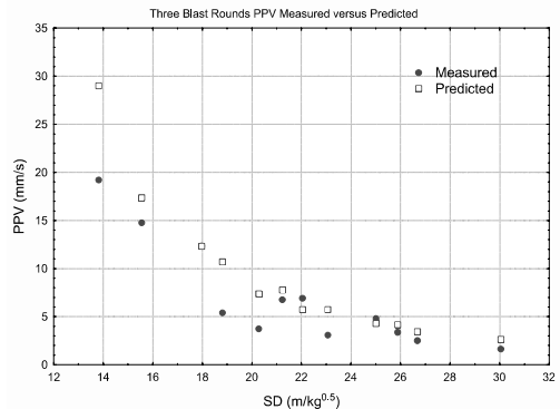
Figure 9. The modeled PPV comparing with the measured from the blast rounds.
