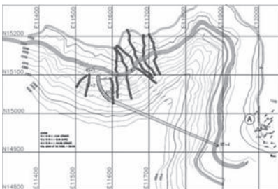
Figure 2. Tunnel alignment & existing road.
