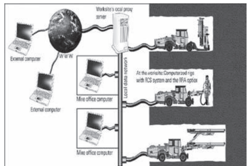
Figure 11. Communication system, for rigs with Atlas Copco’s RRA communication system.
