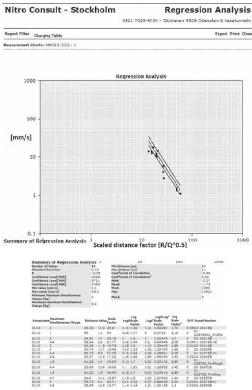
Figures 20–21. A regression analysis and summary enable rapid blast diagnosis and are used to calculate subsequent MICs.
