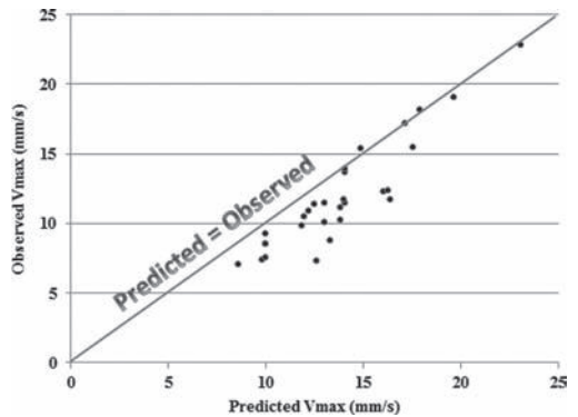
Figure 7. Validation of the blast vibration results.
