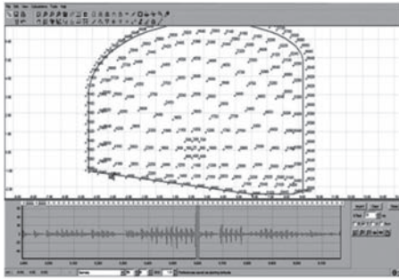
Figure 9. Using SHOTPlus-T and the NCVIB system to compare the recorded waveform with the initiation sequence.
