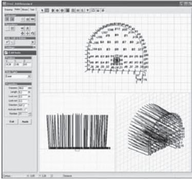
Figure 12. Design tool for drill plan generation.
