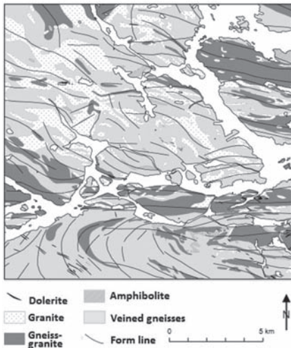
Figure 1. Main rock types in Stockholm bedrock, and structural trends (Persson 1998).
