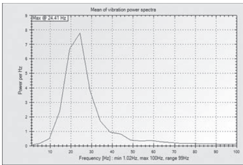
Figure 11. Mean vibration power spectrum for the vibration recorded nearest a 1657 gram charge in Plunkett Street.
