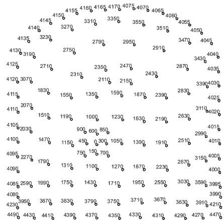
Figure 5. Blast holes and timing in a complete blast round.
