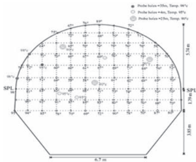
Figure 12. Temperature log of the face at Chainage 1068, Adit-4 (Upstream, HRT, KWHEP), dated 23/02/2009.
