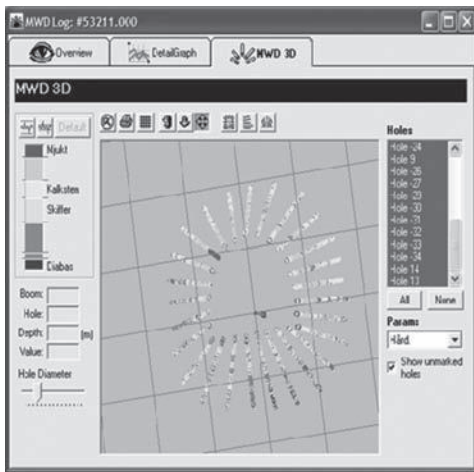
Figure 9. Three dimensional presentation of calibrated MWD data from an injection fan in a subway tunneling project.
