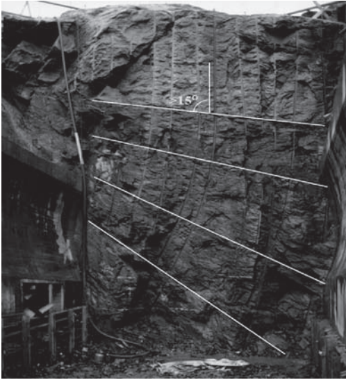
Figure 7. Hole deviation.
