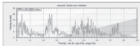
Figure 16. The first predicted waveform produced by the uncalibrated model for design 6 at Plunkett St. Waveform superposition is significant. 25 ms delay between production holes.
