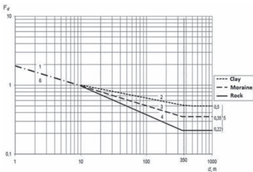
Figure 3. Uncorrected vertical PPV as a function of distance, d .
