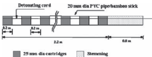
Figure 7. Prefabricated charge for perimeter holes.
