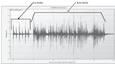
Figure 6. Vibration trace from a complete blast round.
