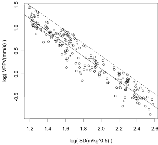
Figure 4. Hume Street vibration data with linear regression fit to transformed data plus a line estimated from the mean standard error of the residuals at a 95% confidence level.
