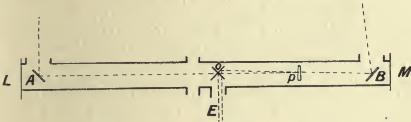
FIG. 134.—Barr and Stroud rangefinder.
