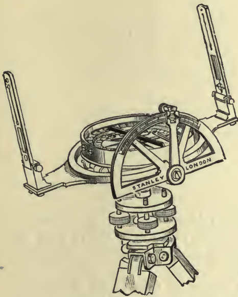
FIG. 45.—Hedley's dial.
