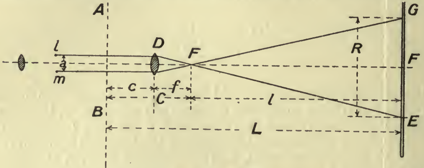
FIG. 121.—Theory of stadia measurements.
