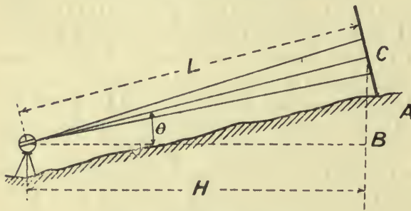
FIG. 123.—Staff inclined.
