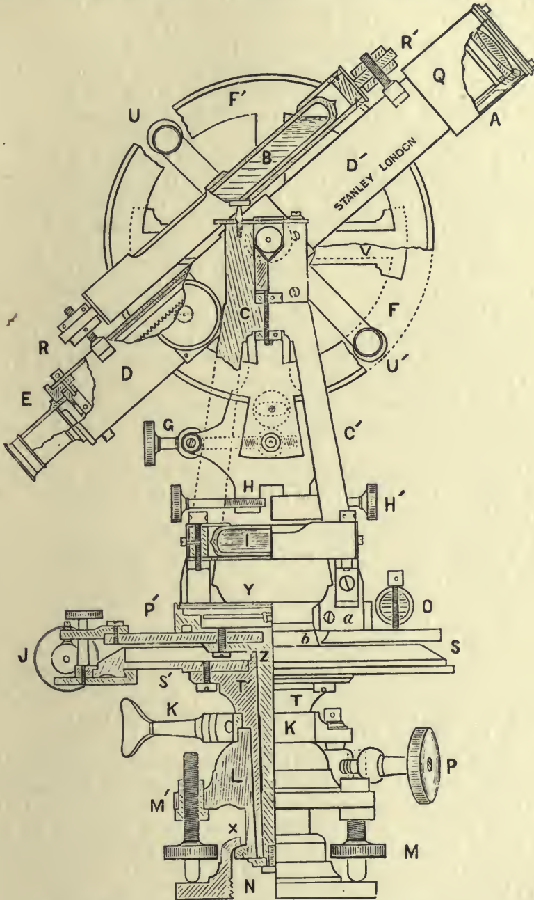
FIG. 78.—Details of 6-inch transit theodolite.
