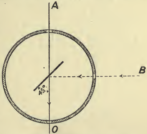
FIG. 14.—Optical square with one mirror.
