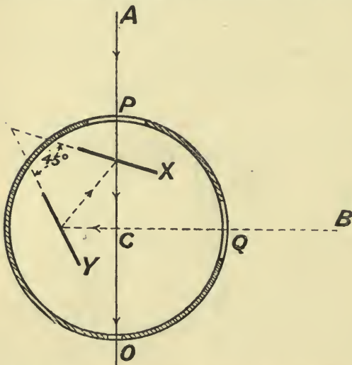
FIG. 12.—Optical square with two mirrors.
