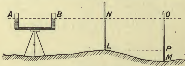
FIG. 102.—Water level.
