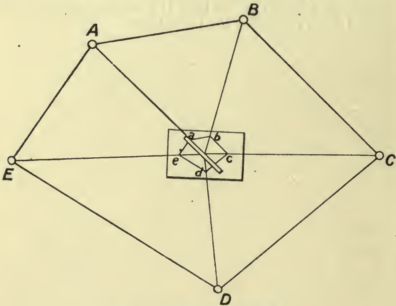
FIG. 55.—Plane table—Radiation.
