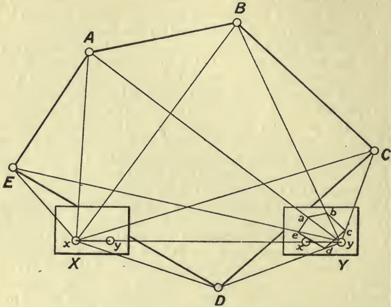
FIG. 56.—Plane table—Intersection.
