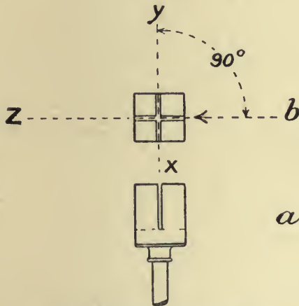
FIG. 8.—Simple cross-staff.
