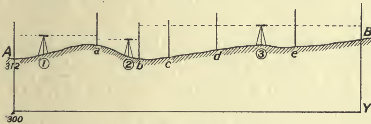
FIG. 112.—Series of levels.
