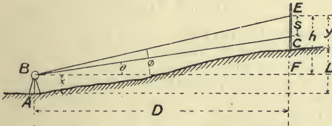
FIG. 126.—Surveying by vertical angles.
