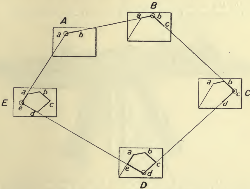
FIG. 58.—Plane table—Traversing.
