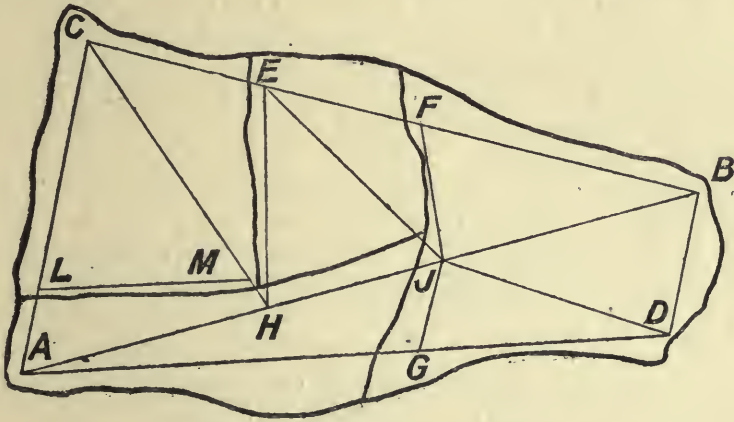
FIG. 17.—Several chain survey.
