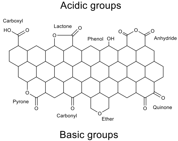
Fig. 1 Surface oxygen functional groups are commonly present in CBMs
