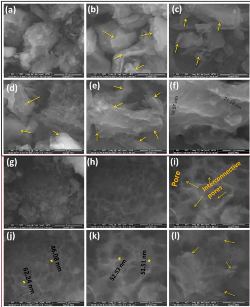
Fig. 6 SEM images of TFSSs after pyrolysis—CVD pure ACNSs a, b, c, d, e, and f and KOH treated TFSS after pyrolysis KACNSs g, h, i, j, k, and l both samples at different magnification. Adapted with permission from ref [63]
