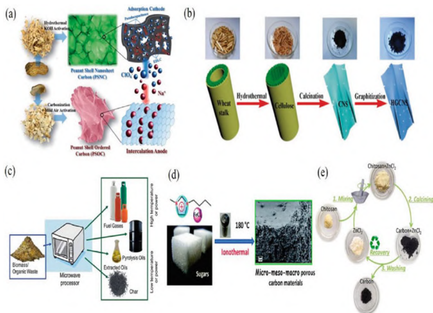
Fig. 3 Illustration of several synthesis techniques used to create biochars made from biomass. a Carbon from peanut shells was produced using a combination of hydrothermal carbonization and activation. Adapted with permission from ref [12]. b Carbon from wheat stalks was obtained by hydrothermal and calcination-graphitization processes. Adapted with permission from ref [13]. c Organic waste is pyrolyzed using a microwave. Adapted with permission from ref [14] d Porous carbon is produced by ionothermal means from sugars. Adapted with permission from ref [15] e Chitosan carbon was formed from molten salt. Adapted with permission from ref [16]
