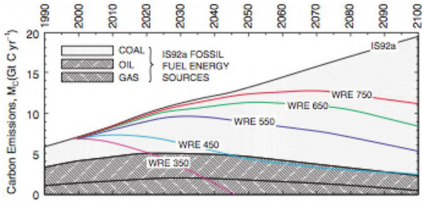
Fig. 1 The emission of CO_2 from fuel energy sources as compared to that present in the atmosphere [8]
