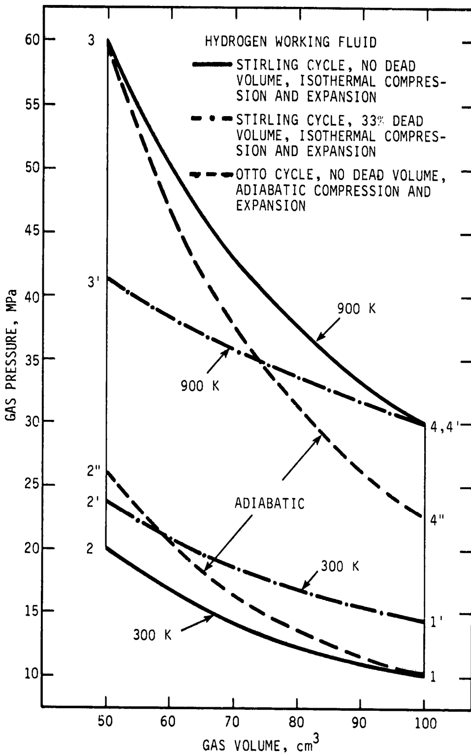
Figure 5-2. Theoretical Cycles.
