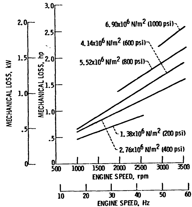
Figure 3-6 Mechanical Loss As a Function of Engine Speed for Helium Working Gas (Determined from experimental heat balance.)
