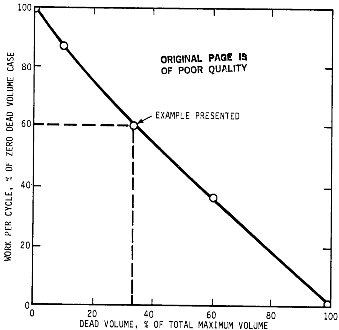
Figure 5-5. Effect of Dead Volume on Work Per Cycle for Isothermal Spaces and Constant Average Pressure.
