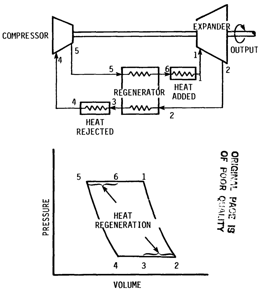
Figure 2-3. Example of Closed Cycle Gas Turbine Engine.
