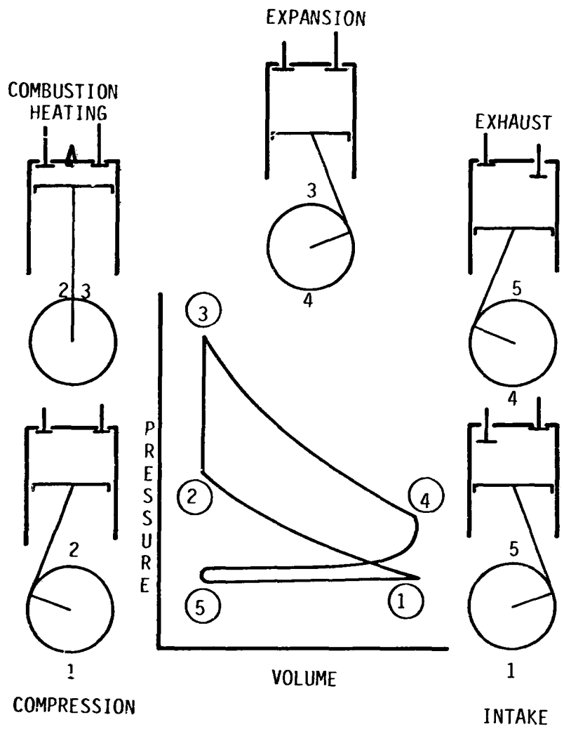
Figure 2-2. Example of Internal Combustion Engine.
