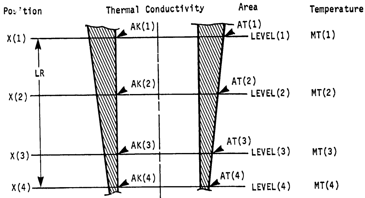
Figure 5-24. Computation of Tapered Cylinder Wall Conduction.
