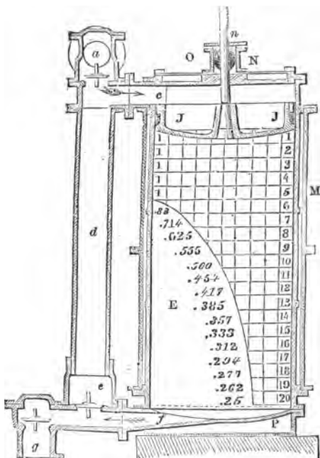
Diagram showing law of expansion of steam in a cylinder.
