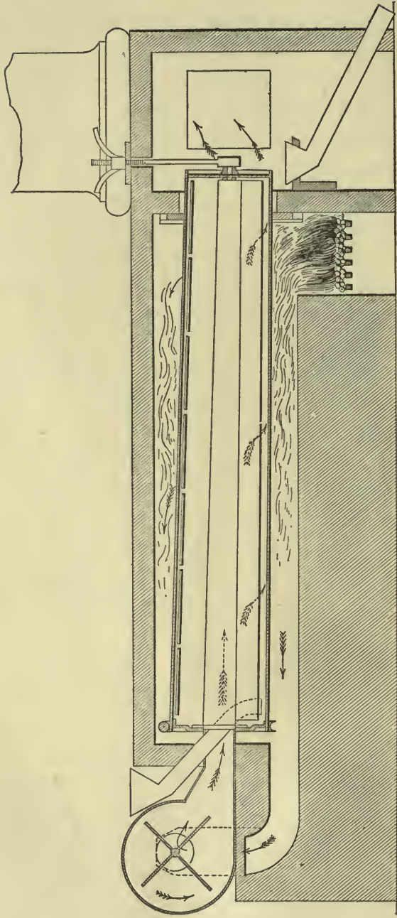
DRYING CYLINDER.
