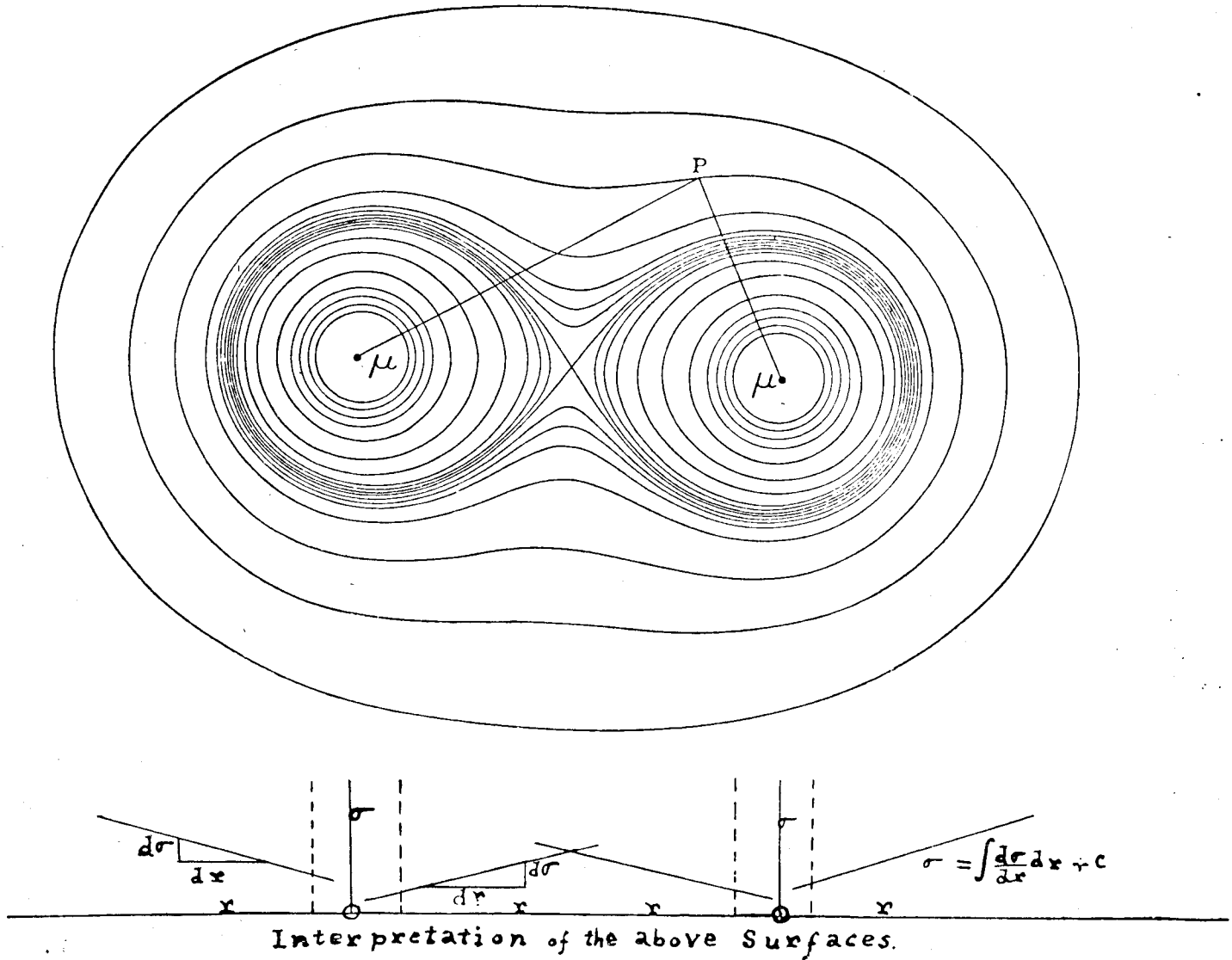
Fig. 15. Diagram of the equipotential surfaces about two equal masses, \mu and \mu , originally given in Thomson and Tail's Treatise on Natural Philosophy , 1st ed. 1873. Without regard to the cause involved this diagram represents the actual surfaces which exist under the potential of gravitation; and in the light of the new theory of the aether we now interpret the meaning of the distortions shown which were first published about half a century ago.
