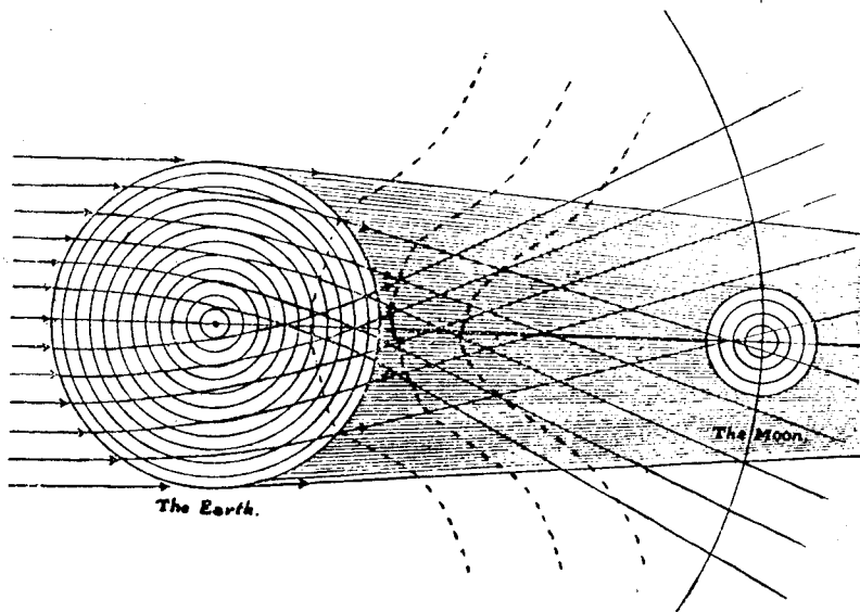
Fig. 13. Illustration of the refraction of the gravitational waves of the sun in passing through the globe of the earth, from the Electrodynamic wave-theory of physical forces, vol. 1, 1917, p. 88. The refracted wave-front is here indicated by pointed lines, to complete the analogy with sound, refracted around the balloon filled with CO_2 , and shown in Fig. 12, plate 7.
