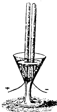
Fig. 1. Decomposition of water into oxygen and hydrogen by the action of an electric current.
