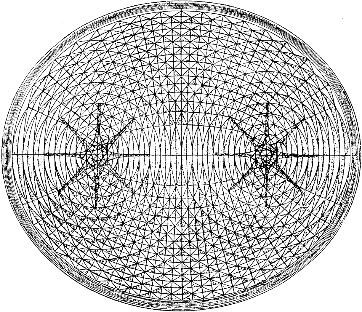
Fig. 19. Geometrical illustration of the wave-field about two equal stars. The wave-amplitudes increase asymptotically towards either body, which renders the aether of variable density \sigma = v/r , while the wave-motion in concentric spheres, when reflected from the surfaces of the confocal ellipsoids, yields stresses along the tangents to the hyperboloids, which intersect the ellipsoids at right angles and with them constitute the system of confocal conics.
