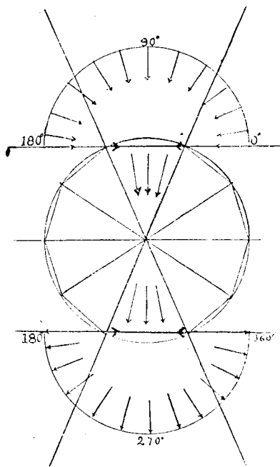
Fig. 6. Stresses in the aether at the boundary, owing to refraction and dispersion of waves by diamond.
