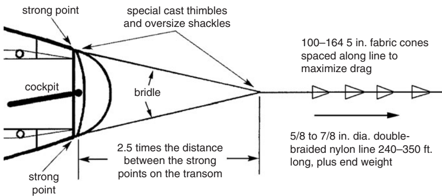
Details of the transom bridle and hookup of a series drogue to allow the boat to run downwind without steering.
