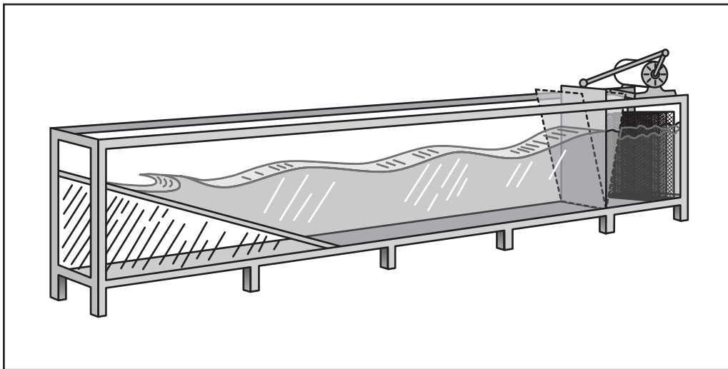
A glass-sided wave channel. A variable-speed motor with an adjustable yoke drives a paddle, hinged at the bottom, to generate waves with periods of 0.7 to 1.4 seconds and heights up to 1 foot. The waves on the backside of the generator are absorbed by special screens.
