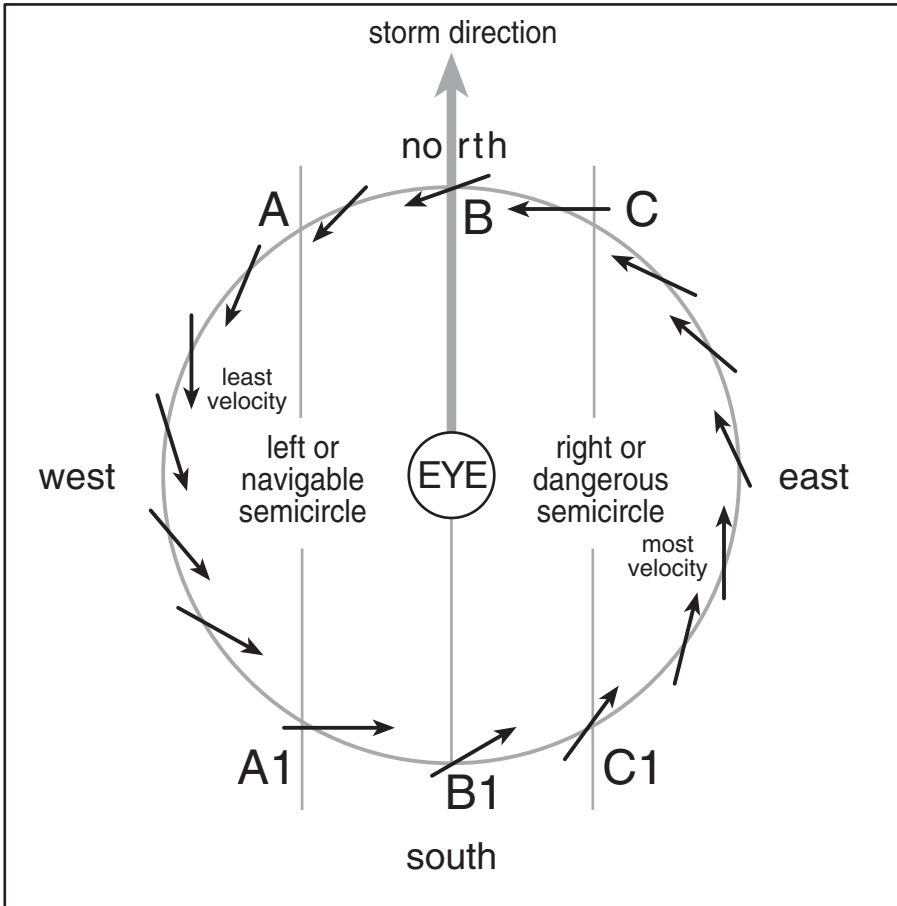
In this drawing the hurricane is headed north, but a revolving storm can travel in any direction.
