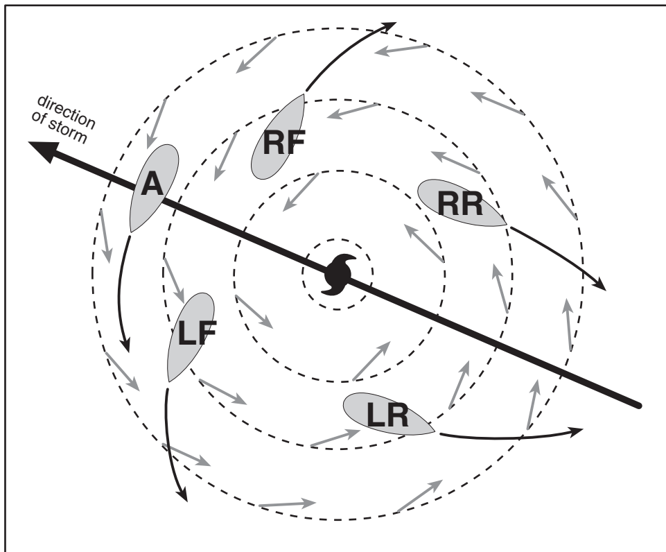
This hurricane is traveling west-northwest. The dangerous quadrant has the vessels RF and RR.
