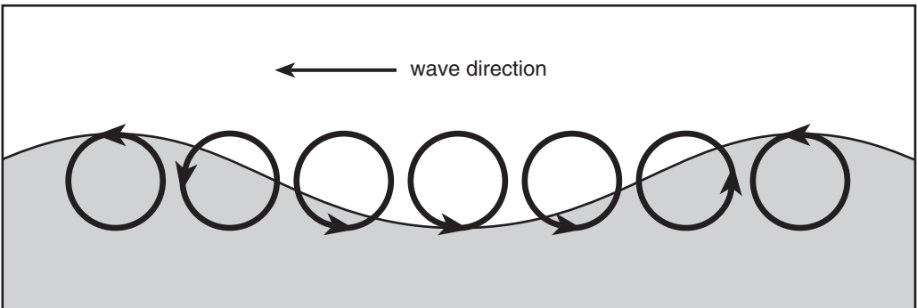
The diameter of the circle is the height of the wave. The period is the time required for the circle to make one revolution. Or said more simply, the particles in the top of the wave move forward; in the bottom of the wave, or the trough, the water particles move backward.
