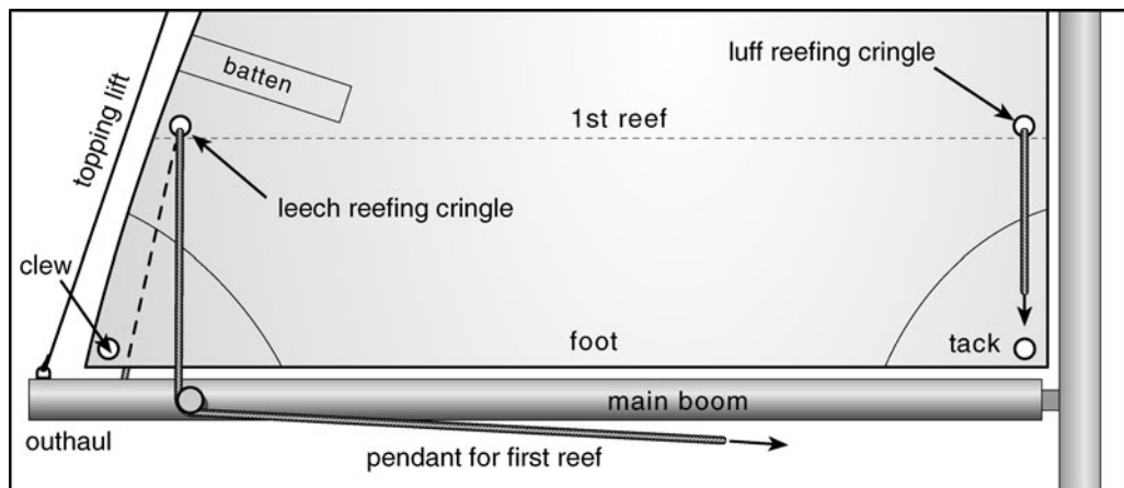
How slab reefs work.
