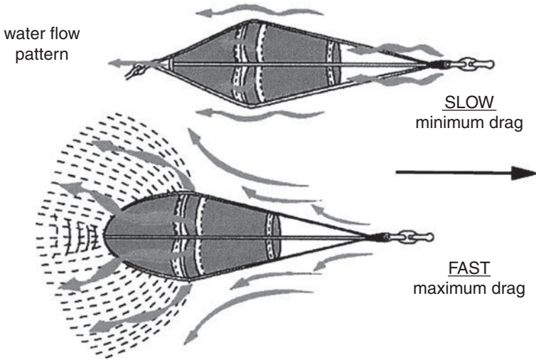
The water flow pattern of the Seabrake as drawn by the inventor.
