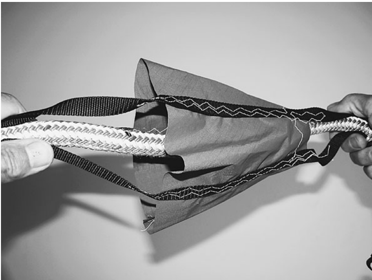
A 6-inch single cone is securely woven into a double-braided nylon line with three \frac{3}{4} -inch nylon tapes.
