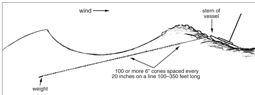
Jordan Series drogue stretched out behind a yacht in heavy going.
