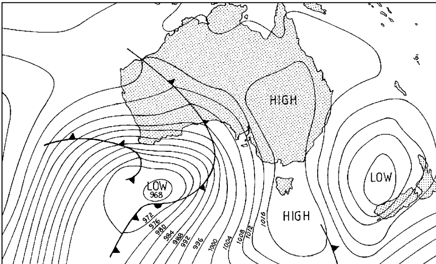
Australian weather chart for July 17, 1996.
