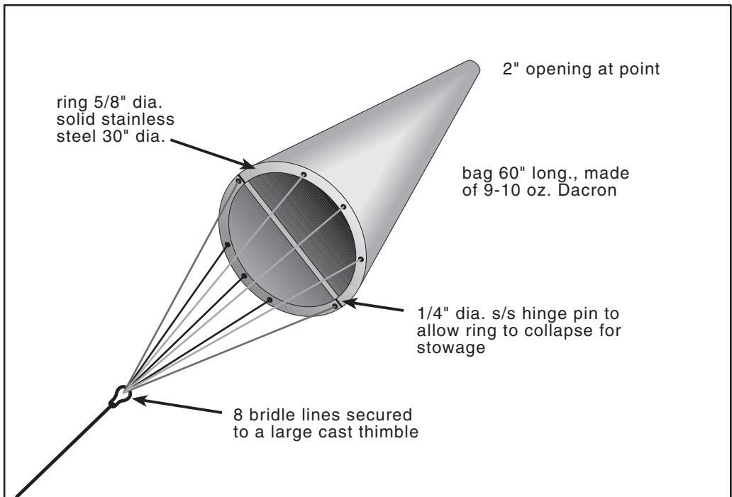
Voss-type fabric sea anchor with hinged metal ring that collapses for storage.
