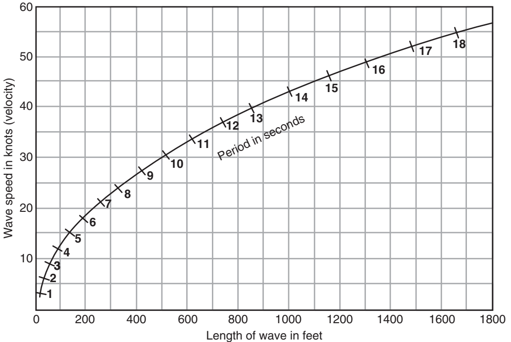
Relationships between speed, length, and period of waves in deep water, based on the theoretical connection between period and length.
