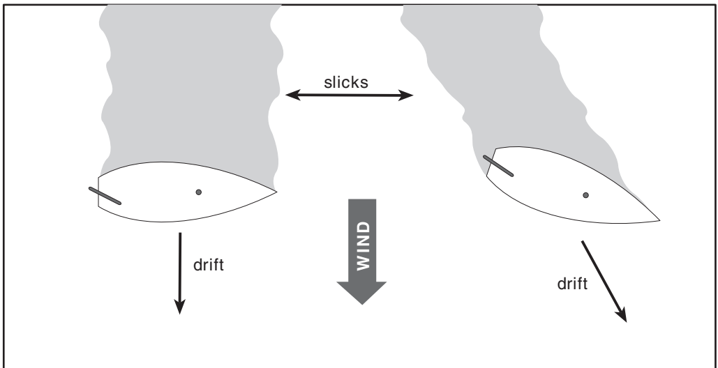
Yachts lying a-hull. The boat on the left is drifting directly downwind and creating a slick to windward. The sailboat on the right is positioned at an angle to the wind. Part of her smooth is wasted, and her port bow area is more exposed.
