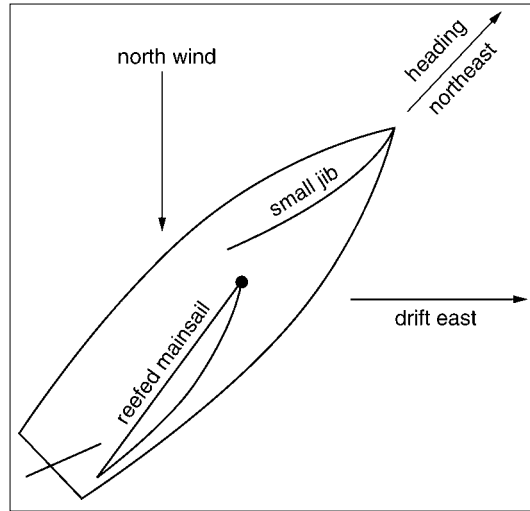
The forces involved when a sailing vessel is hove-to.
