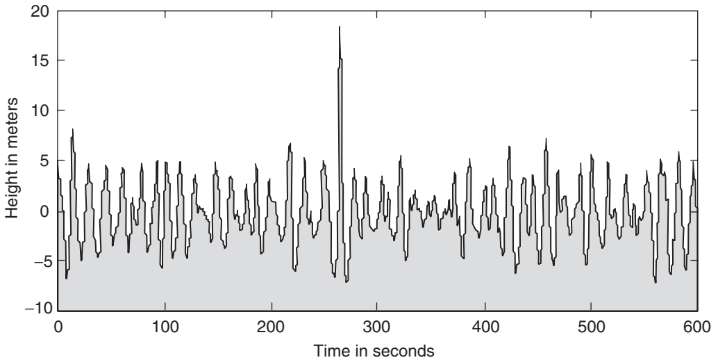
A trace of the Draupner oil rig platform “New Year’s Day wave” in the North Sea in 1995, which changed oceanographers’ perception of superwaves.
