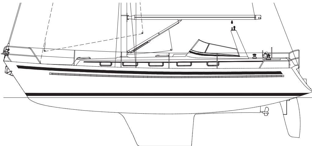
The 2006 Swedish Malö designed by Hans Leander. A typical modern design with three times the draft of Tilikum. With no sails up, this yacht will turn away from the wind, pivoting on her underbody because of the resistance of the mast and forward rigging.
