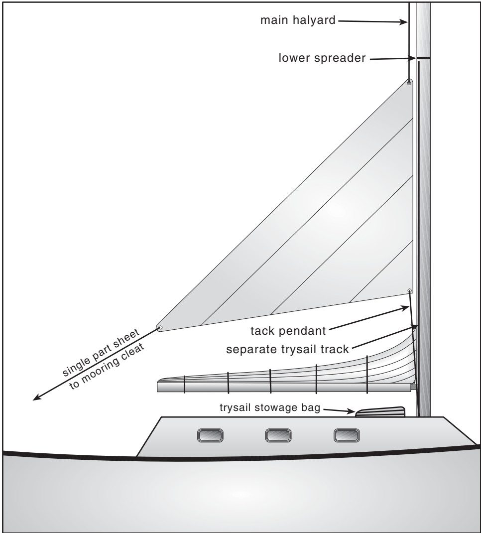
Details of a storm trysail.
