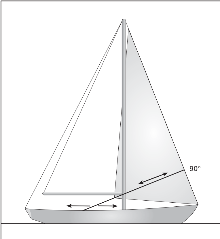
Ideal sheeting angles for furling headsails.
