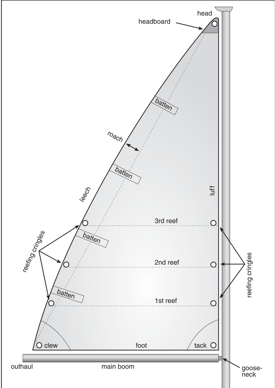
Parts of a Bermudian mainsail set up for slab reefing.
