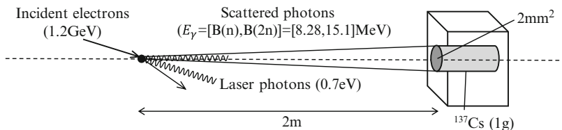
Fig. 1.4 Setup for calculation of transmutation of ^{137}\text{Cs}
