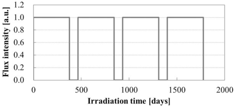
Fig. 20.1 Irradiation history
