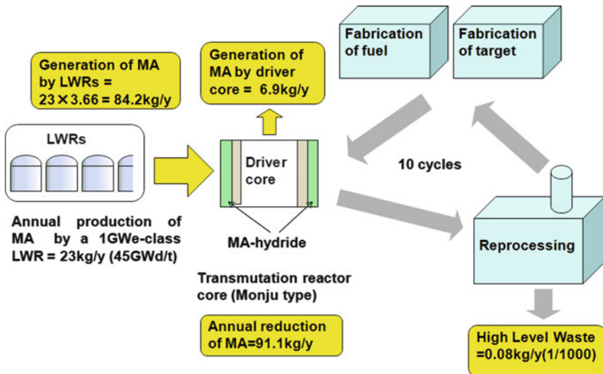
Fig. 16.8 Mass balance of MA in the system of LWRs and FBR with MA-hydride targets
