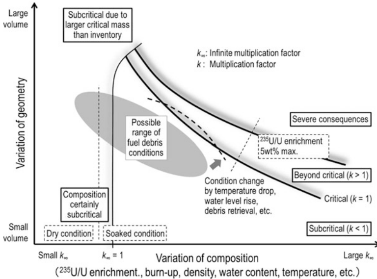
Fig. 21.2 Criticality map of fuel debris
