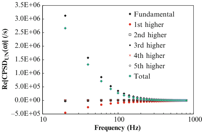
Fig. 12.7 Mode components of the uncorrelated component in the CPSD in the nearly critical system (real part)
