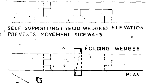
DOUBLE-TENONED SCARF with WEDGES
