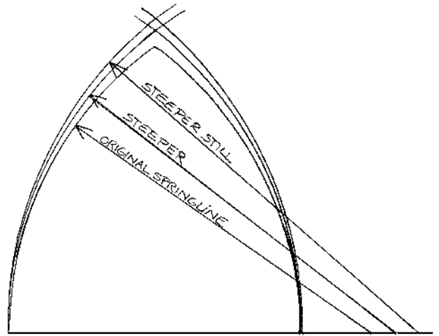
12.31(above): Steepen the profile by drawing several lines from a compass point further from the center of the diameter, and make new calculations from the steeper profile.
