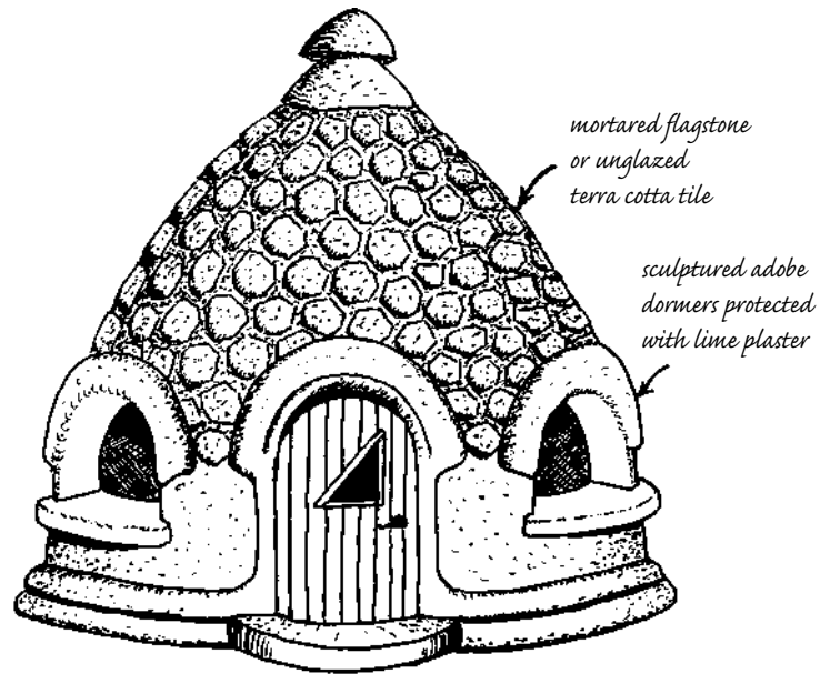
13.4: Low-fired clay tiles set in earthen mortar have been a traditional roof covering on domes in the Middle East for centuries. The mud mortar allows for transpiration, while the tiles inhibit erosion.
