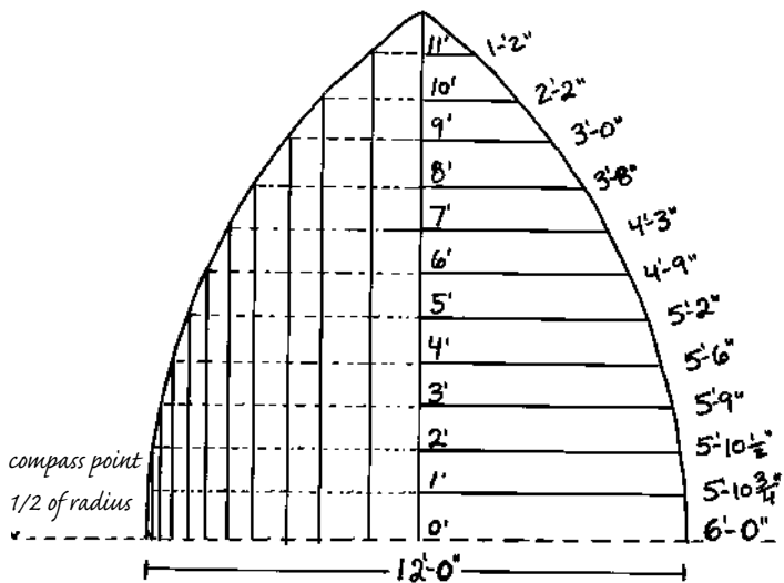
12.17: This diagram shows the approximate lengths to which the compass arm radius must be adjusted at every one foot of height. You can draw a larger diagram that includes measurements at every one inch (2 cm) or less for at-a-glance reference calculations during construction.
