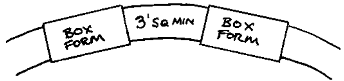
5.13: For a curved wall, take measurement from interior of wall surface to calculate three-square-feet of wall in between openings.
