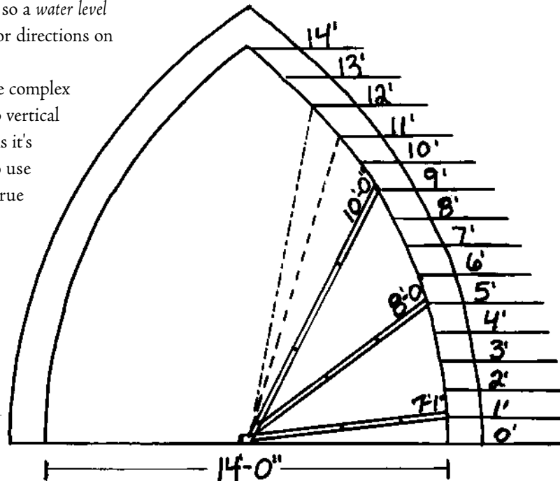
3.46: Expandable compass fixed to center of diameter at springline determines shape by lengthening of the arm at a diagonal.
