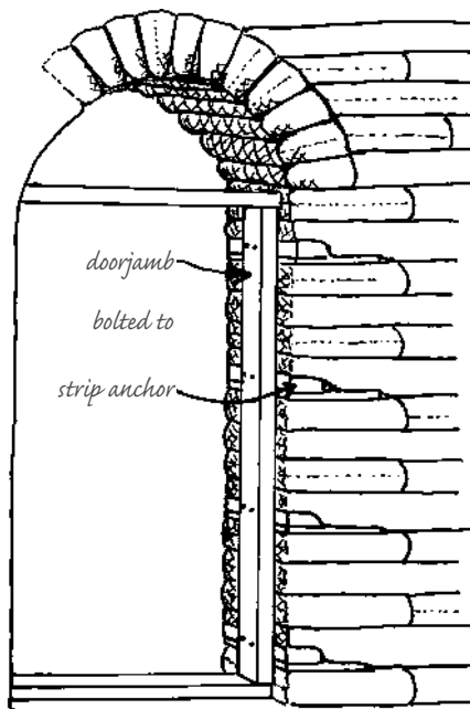
2.30: Most doorjambs can be bolted to an adequate attachment surface that is provided by an average of four strip anchors spaced every three to four rows.
