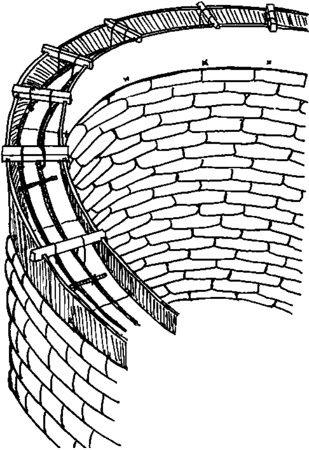
9.7: For curved walls, thin, flexible Masonite can be used as a form.
