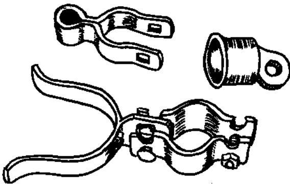
3.42: Common chain link fittings and parts used to build a compass with articulating arm. Clockwise from upper left: Gate-frame grip; rail-end cap; fork latch.
