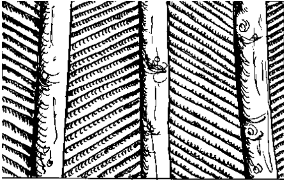
9.17 (above): Vigas set parallel to each other with latillas set in an alternating diagonal pattern.
