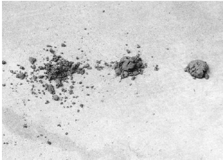
2.7: Three sample balls of soil dropped from shoulder height to the ground. The samples (left to right) show moisture contents varying from 10 to 20 percent.
