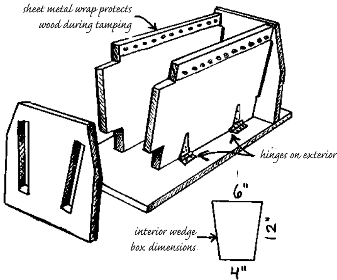
A.33: The Wedge Box
