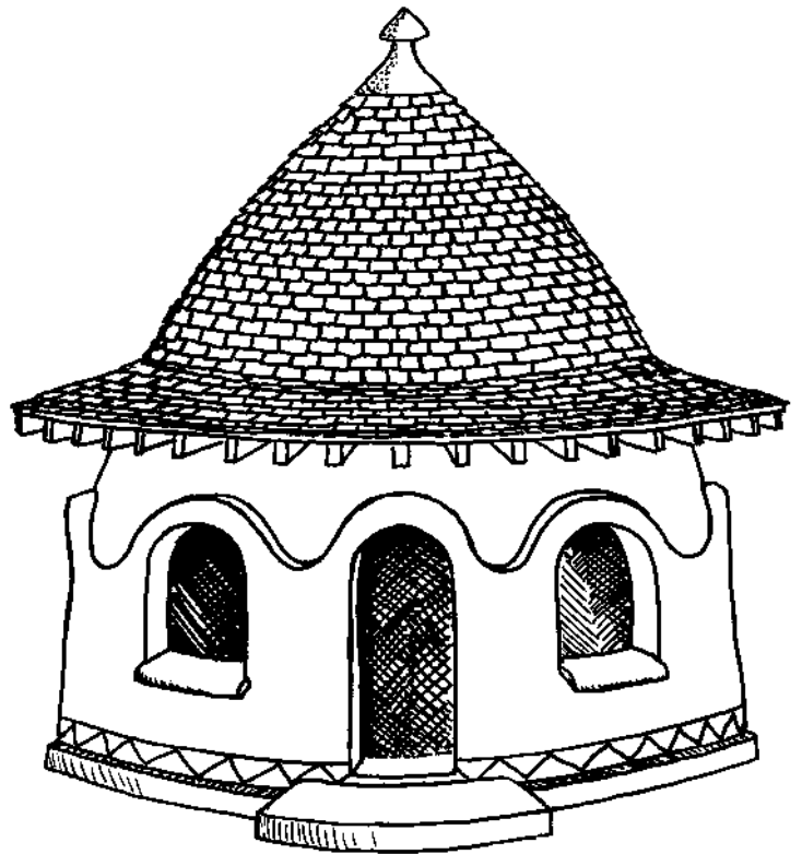
13.8: Shingles applied directly over an earthbag dome with built-in extended eaves to protect walls.
