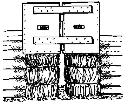
use straw bales to elevate box forms after walls have been compacted
