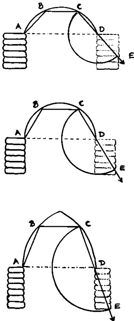
10.9: Point E (where the arrow exits the half-circle) determines how thick the wall buttressing needs to be to support this shape of arch.
