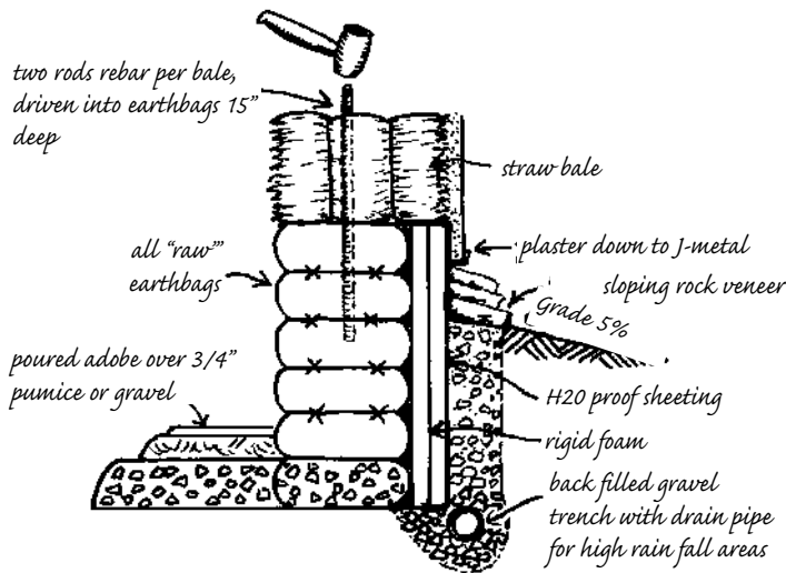
17.13: Insulated below grade level earthbag foundation for straw bale walls.
