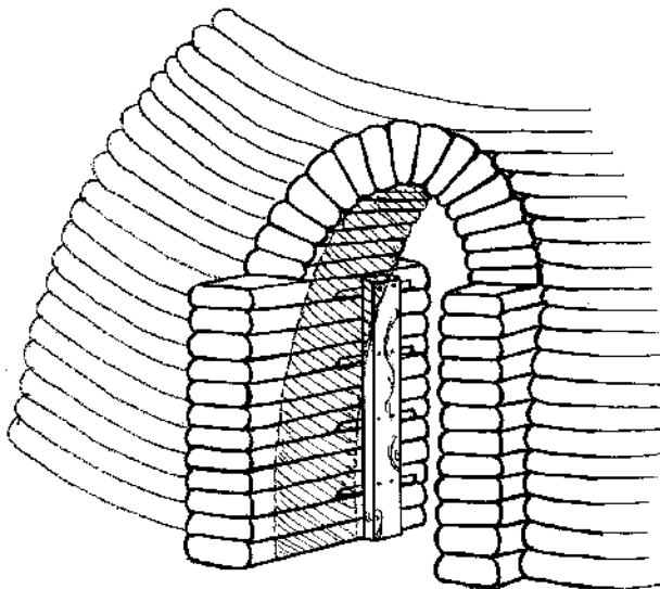
12.16 (left): Door buttressing can be built out of tubes or bags that extend into the interior, exterior, or both. The door opening is the weakest part of the wall in a dome. To ensure structural integrity, incorporate buttressing alongside the door forms. Buttressing provides extra wall width needed for installing a plumb doorjamb. (The shaded area indicates the contour of the corbelled wall.)
