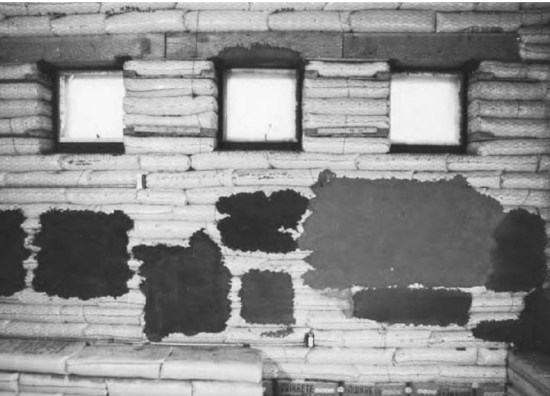
15.4: Plaster test patches on the wall at Sand Island Ranger Station.
