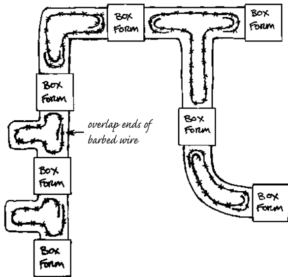
5.8: To maintain as much tensile strength as possible, continue barbed wire around corners, and integrate into buttresses and intersecting walls.
