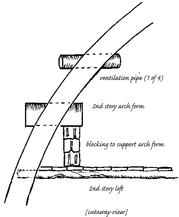
12.29: Providing support for the second-story arch forms may require extra bracing. Note the installation of upper ventilation pipes.
