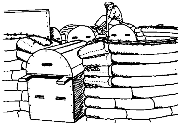
12.20: Incorporate the barbed wire from the wall in between every fan bag around the arch forms, as shown in the step-by-step illustrated guide, and integrate tubes with bags against the forms.
