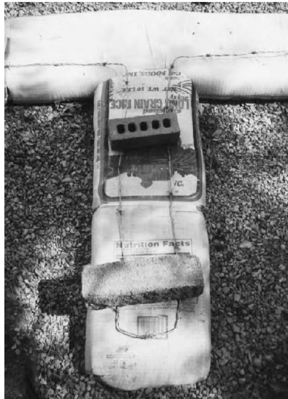
2.18: Use long enough weights to hold down two strands of barbed wire per row at two- to three-foot intervals along the wall.
