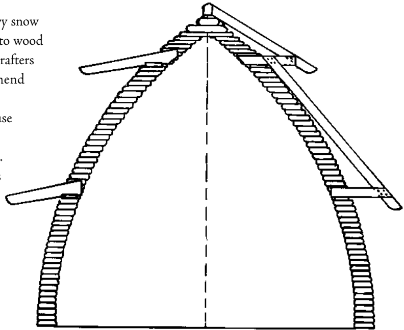
"Japanese bird cage" style light wood frame attached to extended eaves
