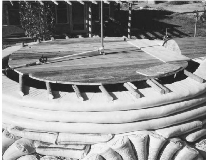
12.24: We used lodge poles for the joists of our loft. We ran them straight across and staked them into the wall with 12-inch (30 cm) spikes. A more sophisticated method could be any of the systems described for anchoring rafters or shelf brackets on top of Velcro plates, as described in Chapters 7 and 9.
