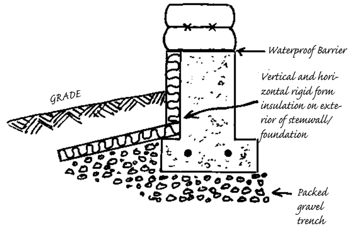
4.4: Shallow, frost-protected foundation.
