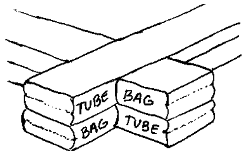
5.11: Alternate tubes with bags to extend beyond the wall to create buttressed corners.
