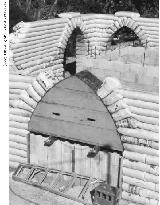
3.30: Tube work is integrated with the fan bags forming an arched opening, rather than taking the place of fan bags.
