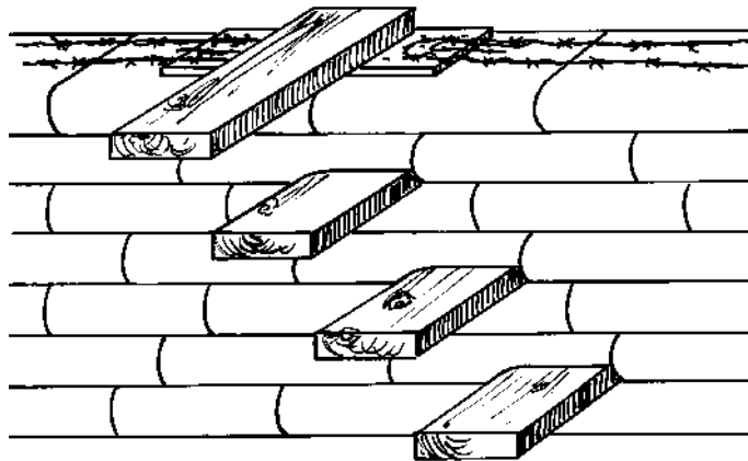
7.13: Stagger plank steps during construction, seated on Velcro plates.
