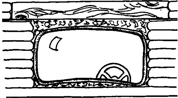
8.12: Car windshield sealed with a hose gasket, secured with adobe/cob under a wood lintel. What could be better than to view life through a Chevy?
