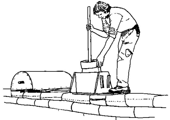
3.20: Using the wedge box to form fan bags.
