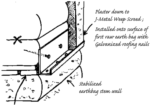
4.10b: J-Metal weep screed detail.
