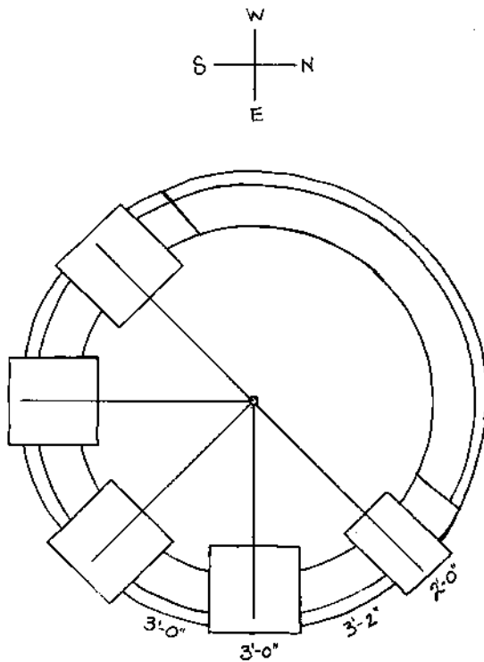
12.12: We made a top, or plan, view, drawing to delineate how we wanted the windows and door oriented by sighting the compass arm down the center of the box forms.
