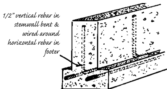
4.2: Cross-section view of a typical concrete foundation and stem wall.
