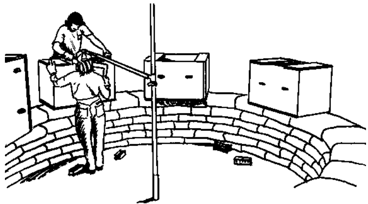
12.13: Use the compass to align box forms.
