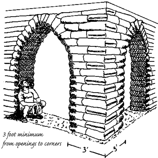
5.10: Alternate overlapping bags at corners mason-style for extra strength. To increase the mass where these two Egyptian-style arches are located, we built the entire corner using 20-inch wide 100-lb bags.
