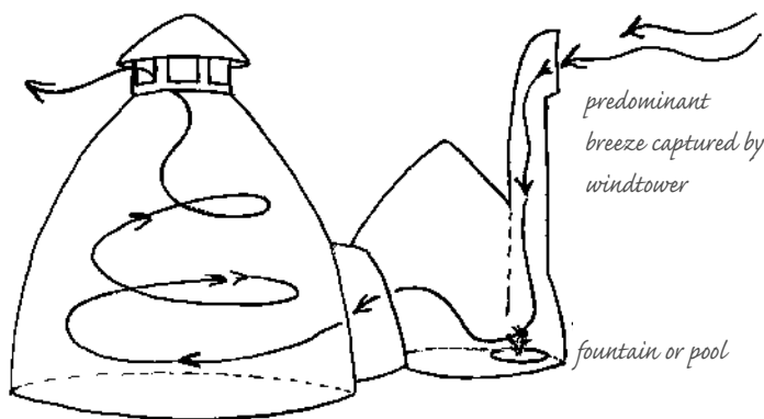
17.3: Wind-catchers.
