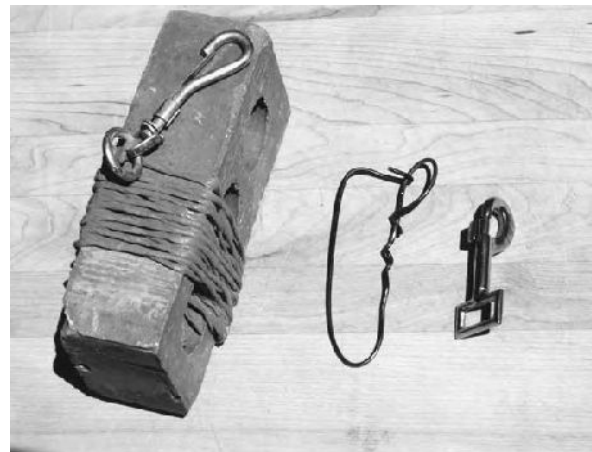
3.15: Left to right: Loaded suspended brick weight; home-made wire hanger clip; store-bought spring clip.
