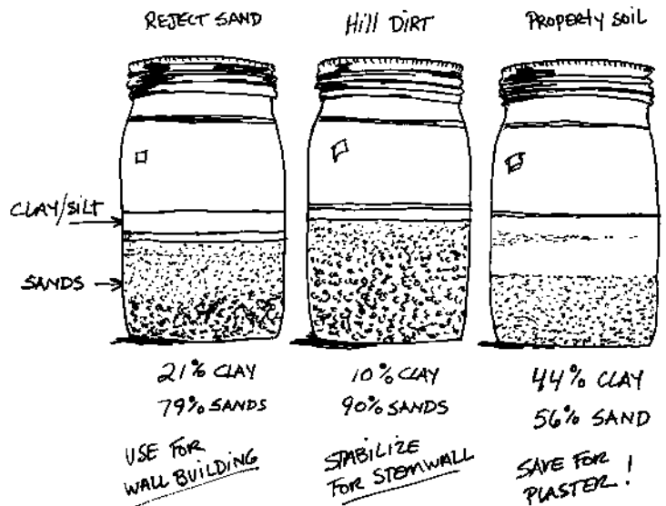
2.3: The Jar Test. Three sample soils and their appropriate uses.
