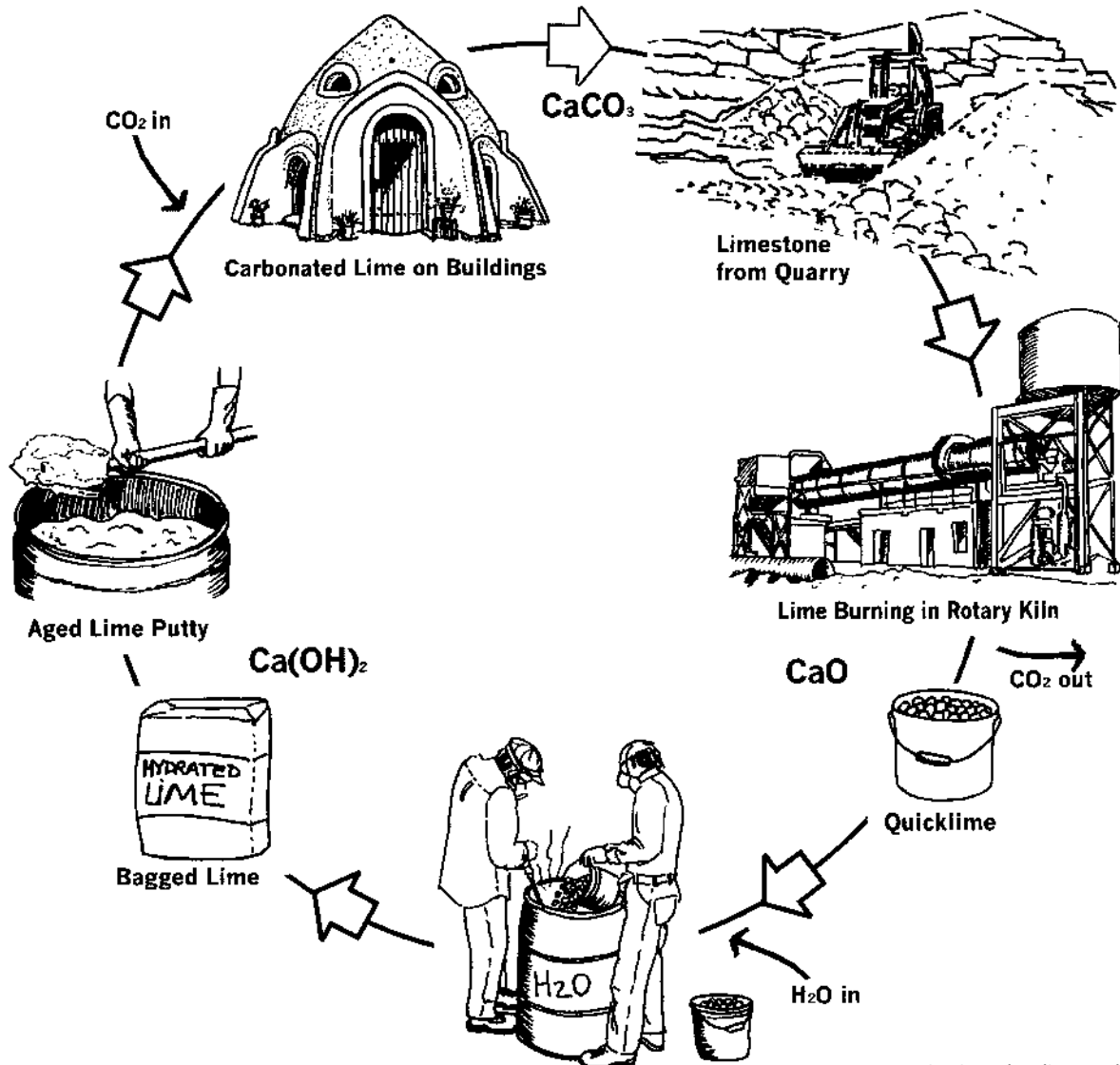
14.14: The lime cycle.
