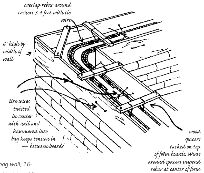
9.4: A minimum of two continuous #4 steel reinforcing bars are suspended in the form to provide tensile strength for the concrete.
