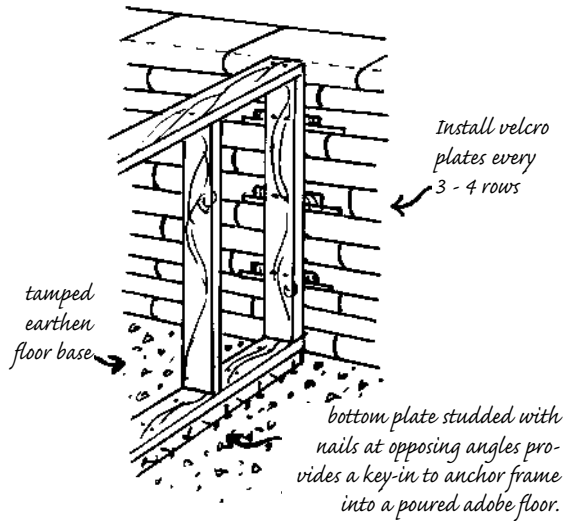
7.7: Intersecting stud frame wall lag-screwed to strip anchors.
