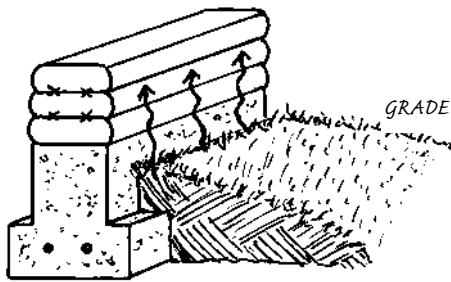
4.8: Capillary action: Without a capillary break, moisture in the ground is wicked up by the concrete and absorbed into the more porous earthen wall above.
