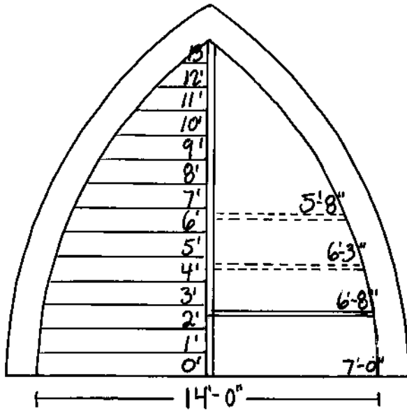
3.47: Pole compass with adjustable length horizontal arm is used to determine radius width by shortening the length of the arm.
