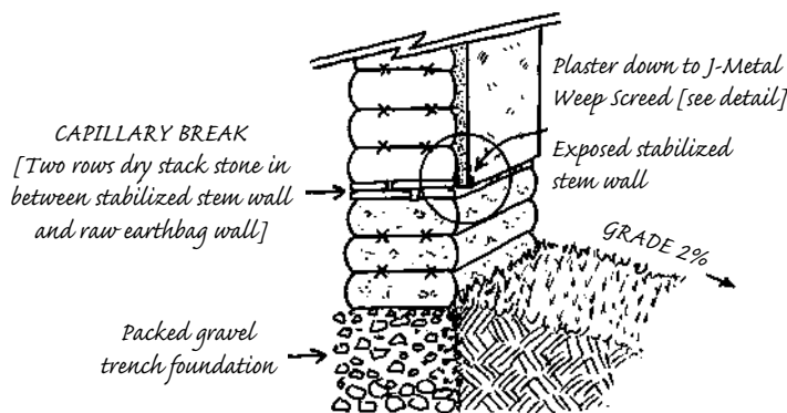
4.10a: Dry-stacked, flat rock capillary break. Weep screed between earth plaster and stabilized stem wall.
