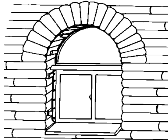
8.5: Manufactured vinyl window with homemade wood sill and a half-round glass protected with a hose gasket. Both windows are secured with shims until sealed with plaster.
