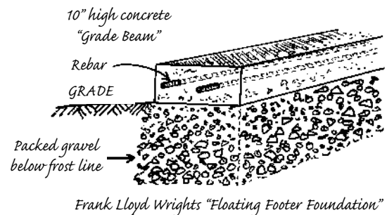
4.3: Floating footer on a rubble trench foundation.
