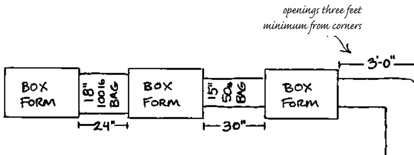
5.12: Two ways to create three-square-feet of wall in between openings using different size bags.
