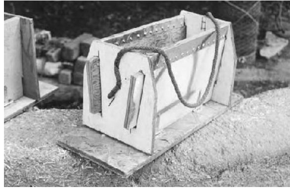
3.19: The wedge box is a form for creating uniform fan bags.
