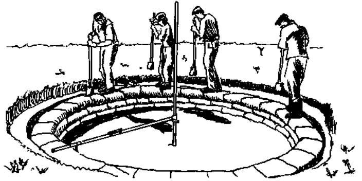
12.9: Continue the bag work until the bags are up to or just below grade. This is where the stem wall of the structure will begin.
