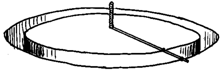
12.34: Use a string compass to designate interior and exterior of foundation trench. Trench style foundation for a grade-built dome, include trench work for any buttressing. Fill entire trench with rubble rock and gravel up to or just below grade.
