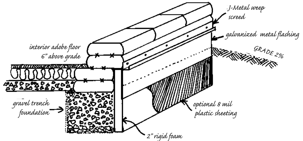
4.14: Insulated earthbag foundation.
