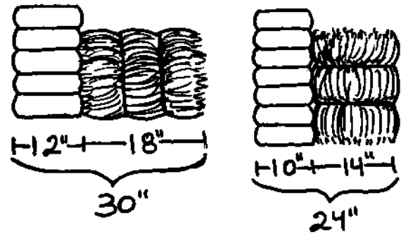
17.9: Alternate configurations of earthbags and straw bales used to achieve mass and insulation.
