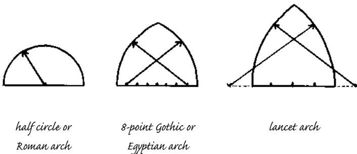
10.6: The placement of the compass point determines where the springline begins and defines the shape of the arch. The further the compass point is placed from the center of the baseline, the taller and steeper the profile becomes.
