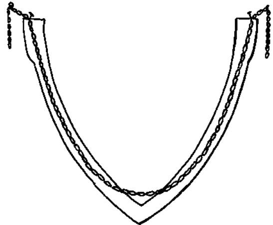
11.20: The suspended chain should hang within the center third of the roof and walls, and, where the chain exits the compass profile, is where buttressing is added.
