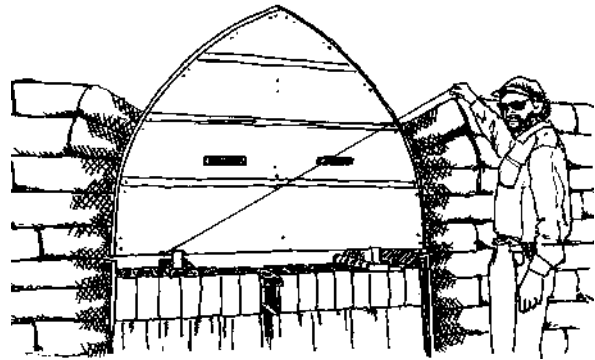
6.57: Eight-point Egyptian arch springline.
