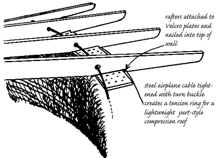
9.22: Light-wood, compression-style roof with extended eaves on earthbag walls.
