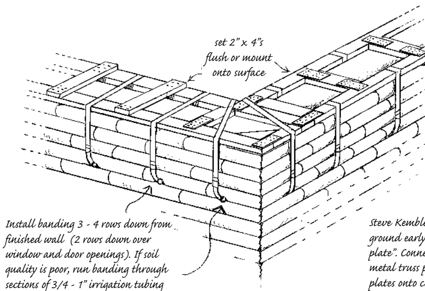
9.8: Light wood ladder roof plate cinched to wall with woven poly banding (strapping).
