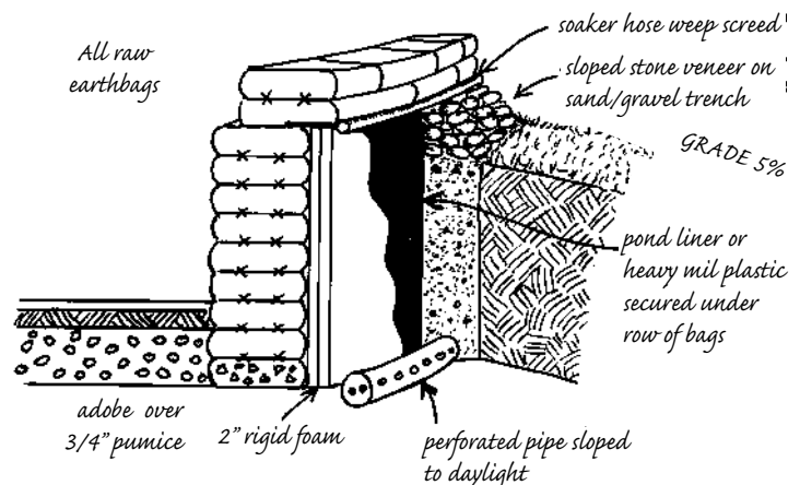
4.15: Curved, insulated foundation with interior sunken floor.
