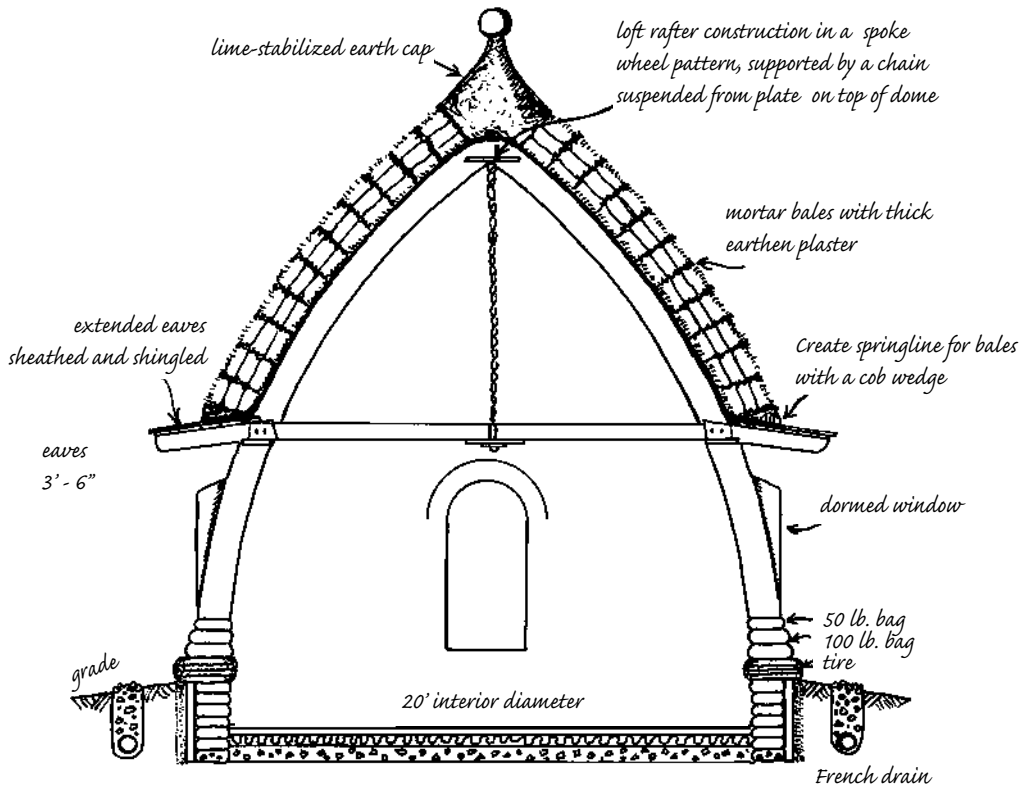
13.11: Scale model of a 20-foot (6 m) diameter earthbag dome with external straw-bale-insulated roof.
