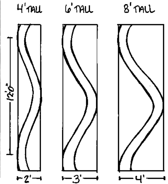
5.6: Examples of height to width ratios for curved, freestanding walls. (Bird's eye view).
