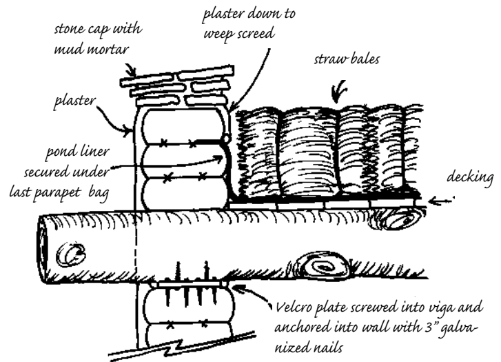
9.29: Detail of straw bale insulated, vaulted viga roof.
