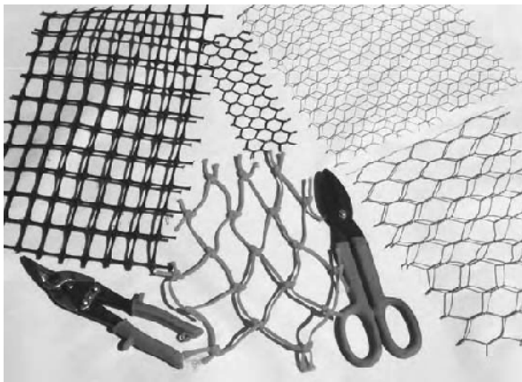
2.21: Examples of a variety of plaster lath, also referred to as stucco mesh.
