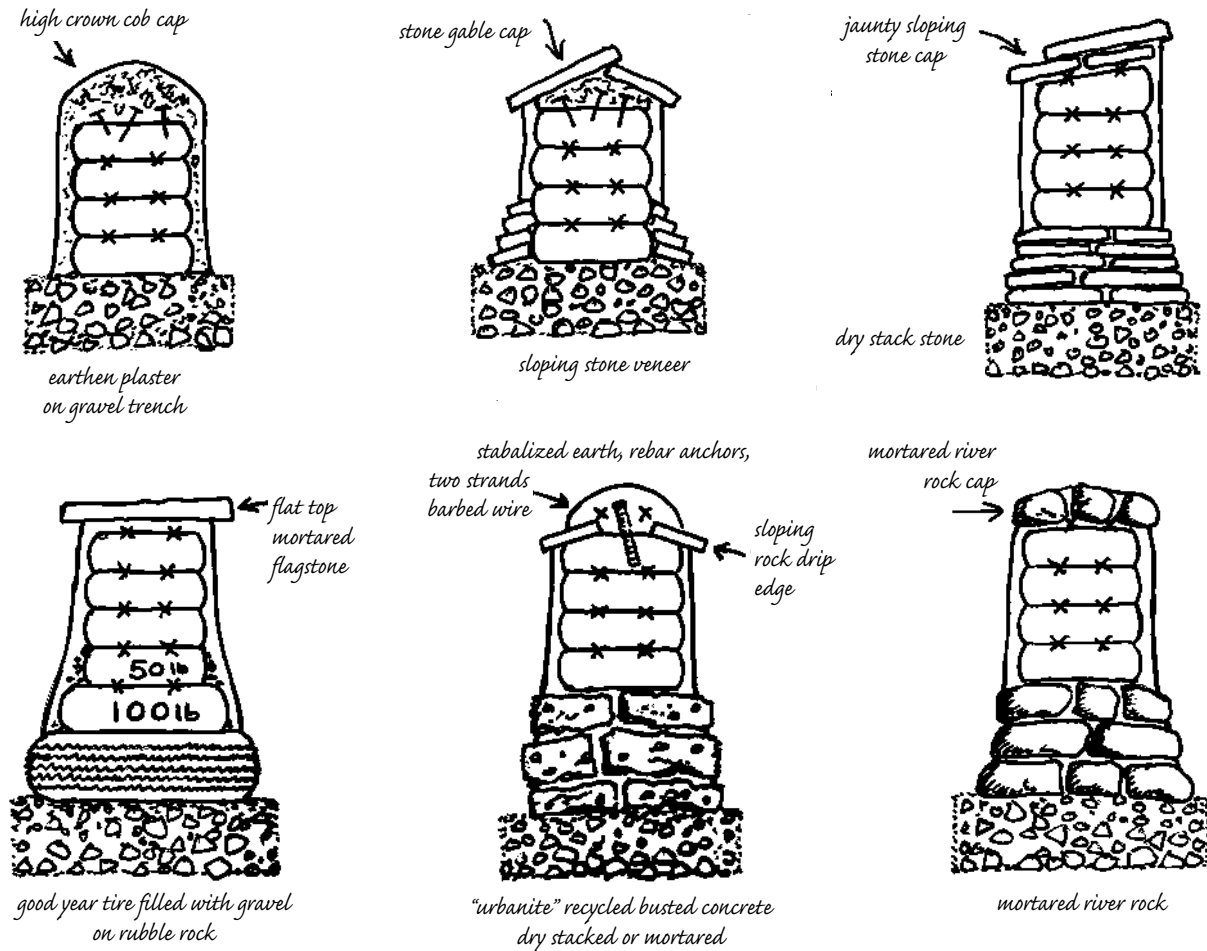
4.12 (below): Traditional and alternative foundation/stem walls.
