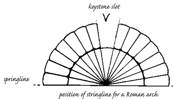
10.7: Examples of a Gothic and Roman arch with stringlines and keystone slots.
