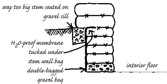
12.10: Honey House foundation detail.
