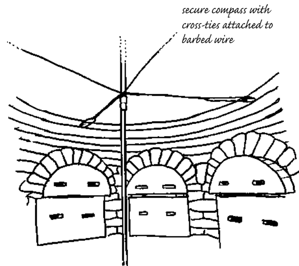
12.23: You will definitely need to shore up the compass pole with cross-ties if a coupling is used. Raise these cross-ties as the wall gets higher, to add more stability.
