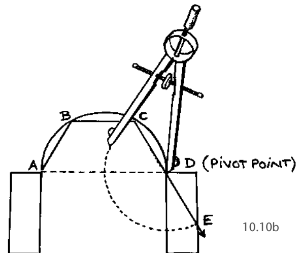
10.10a & b: After using the compass to locate the equidistant points of A, B, C, and D, create the arc between points C and E, using point D as the pivot point.
