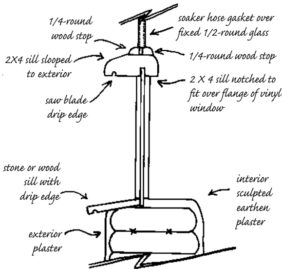
8.6: (Above) Side view detail of vinyl window installation. 8.7: (Right) Split a length of five-eighths-inch (1.56 cm) soaker hose as a gasket over a one-quarter-inch thick plate or thermopane glass that has been pre-cut in a half-round shape.
