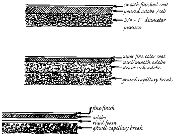
16.2: Three ways of insulating an adobe floor.
