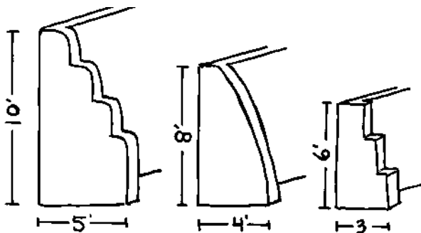
5.5: A ten-foot (3m) tall wall will need a buttress with a total depth of five feet (1.5 m), spaced at every 12 feet on center. An eight-foot (2.4 m) wall will need a buttress four feet (1.2 m) deep, and a six foot (1.8m) tall wall requires a buttress that is three feet (0.9 m) deep.
