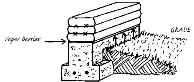
4.9: The waterproof membrane prevents capillary action, inhibiting water absorption by imposing a barrier.
