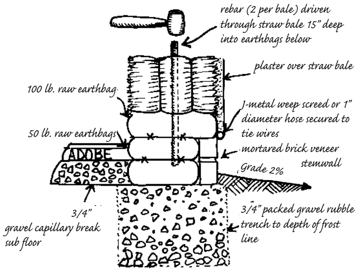
17.12: Grade level earthbag foundation for non-load bearing straw bale walls.
