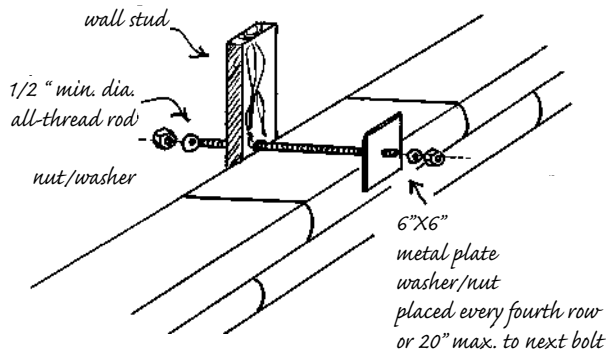
7.8: Stud frame wall attached with all-thread and bolted through an earthbag wall.
