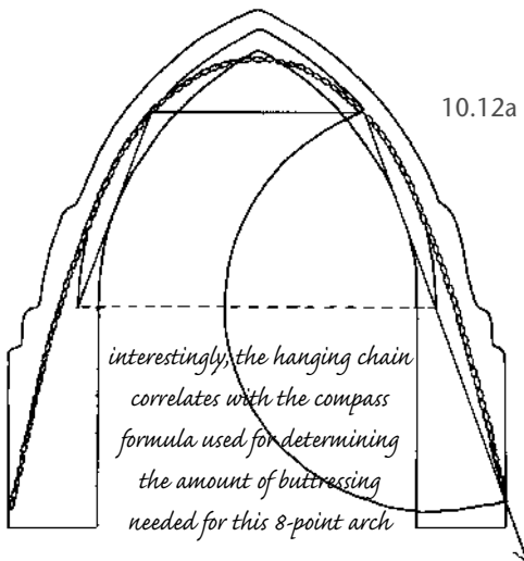
10.12a & b: Within the lines of force of every successful arch resides the imprint of the catenary curve. Every shape arch, whether it is tall and slim or shallow and thick-walled, is designed to contain within its core the natural equilibrium of the hanging chain.
