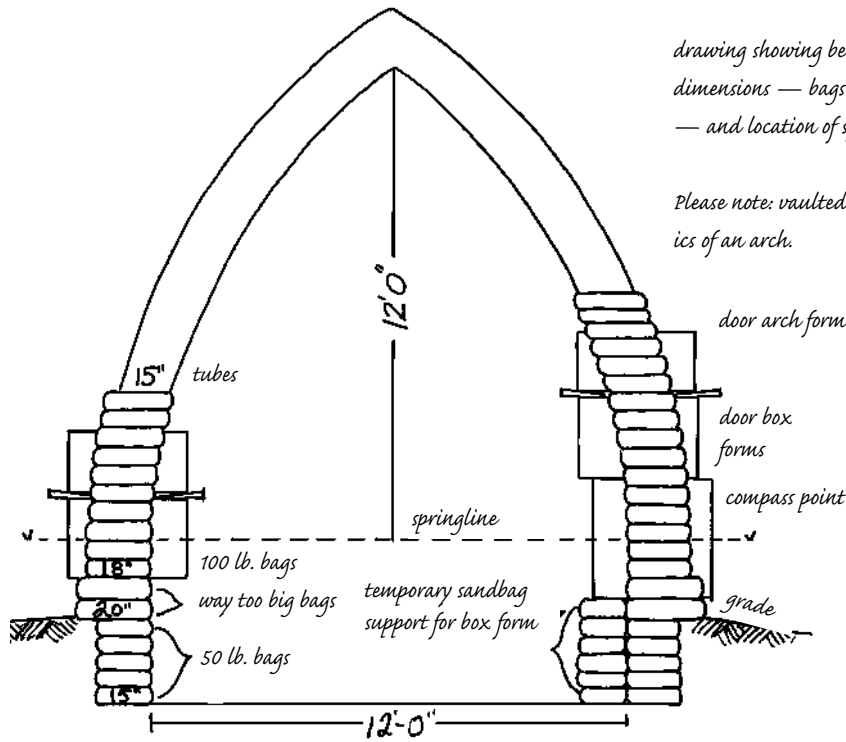
12.2: Elevation drawing depicts below-ground foundation, internal dimensions, and compass profile.
