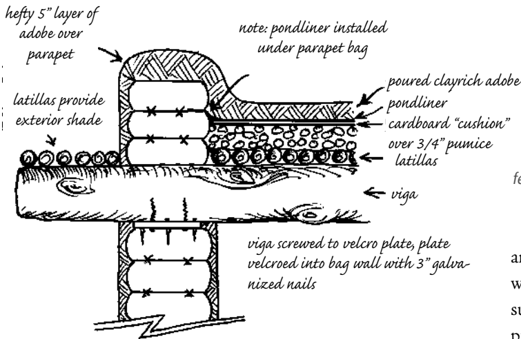
9.31: Exterior insulated, poured adobe roof for dry climates.
