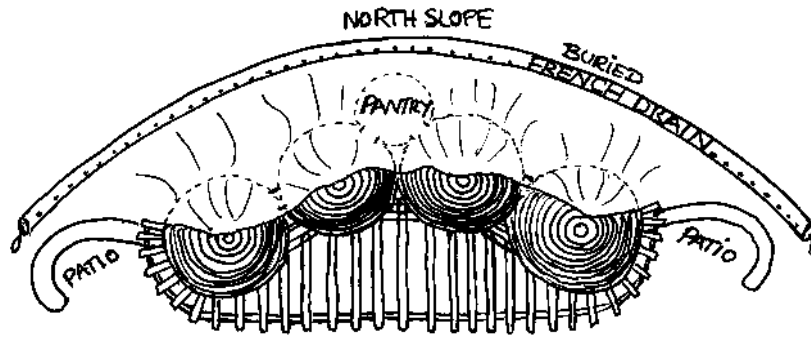
17.14: Four interconnected, bermed domes with buried dome pantry flanked by retaining walls — south face enclosed with attached sunroom in cold climates, or use as covered porch or trellis in hot climates.
