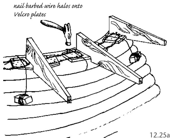
12.25a & b: (a) Extended eaves attached to plate and Velcroed into tamped bags. (b) Infill between eaves with the next row of bags and tamp snugly.
