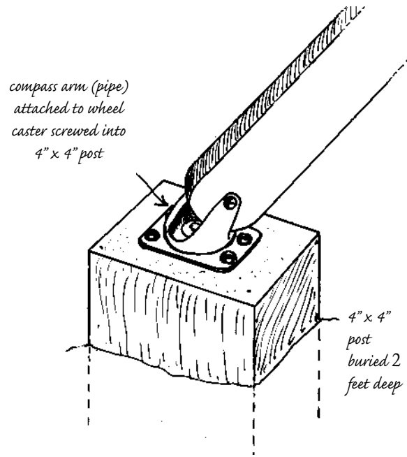
3.45: Detail for a caster wheel attachment.
