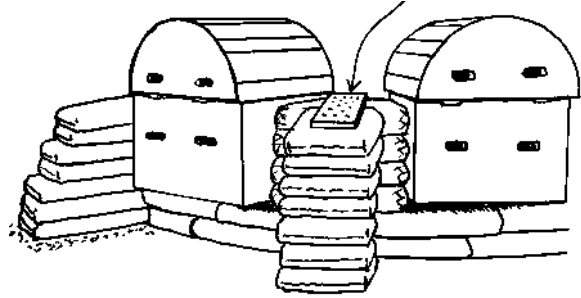
12.14: Incorporating buttresses is another way to increase the mass in between openings while keeping the openings relatively close together.
