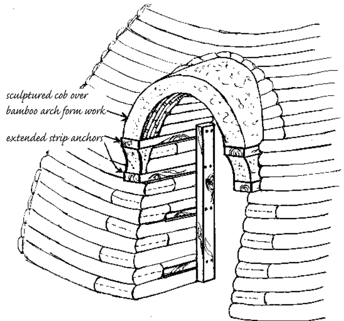
12.16 (left): Door buttressing can be built out of tubes or bags that extend into the interior, exterior, or both. The door opening is the weakest part of the wall in a dome. To ensure structural integrity, incorporate buttressing alongside the door forms. Buttressing provides extra wall width needed for installing a plumb doorjamb. (The shaded area indicates the contour of the corbelled wall.)
