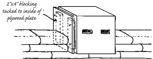
6.44: Doni suggests removing screws (or nails) from the plywood after a few rows of bags. Compression alone is enough to hold the side wedge board in place.
