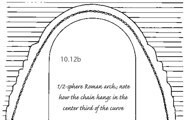
10.12a & b: Within the lines of force of every successful arch resides the imprint of the catenary curve. Every shape arch, whether it is tall and slim or shallow and thick-walled, is designed to contain within its core the natural equilibrium of the hanging chain.
