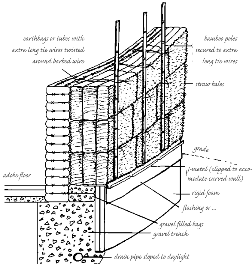
17.10: Earthbag wall with straw bale wrap.
