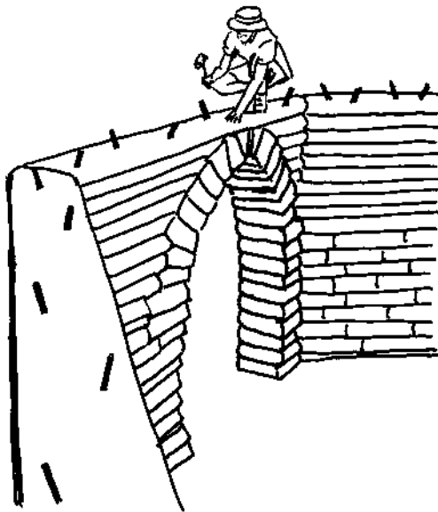
9.3: To anchor the bond beam to an earthbag wall, 16-inch (40 cm) long, #4 reinforcing bar (rebar) is driven 12 inches (30 cm) into the green (uncured), tamped earthbags at a maximum 20 degree angle, at least 4 inches (10 cm) in from the outer edge of the bag, and staggered at 24-inch (60 cm) intervals.
