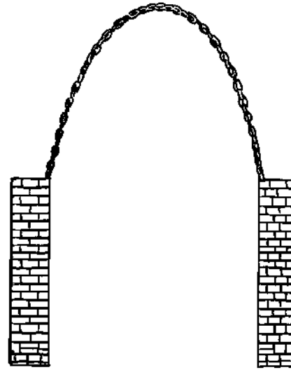
10.11b (right): When the catenary curve, in Figure 10.11a, is turned upside down, it creates an arc in complete compression.
