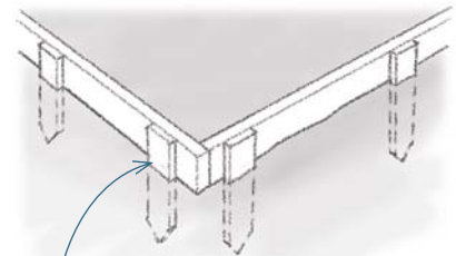
2x4s or 2x6s are nailed to small stakes driven into the ground every 4 ft.
