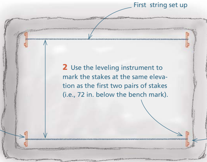
Plan view of excavation
