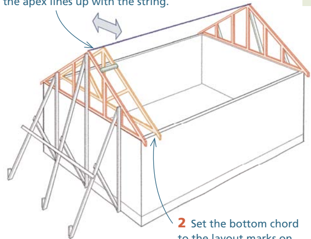
Lateral restraints
