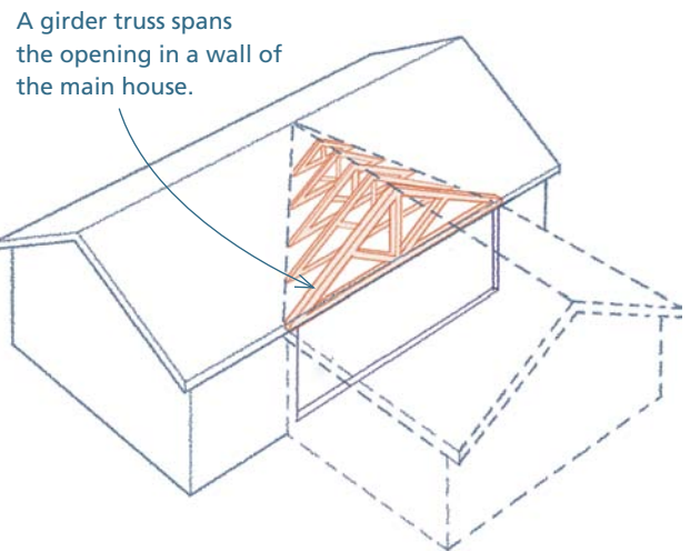
A girder truss supports both the main roof and the valley trusses in this area.
