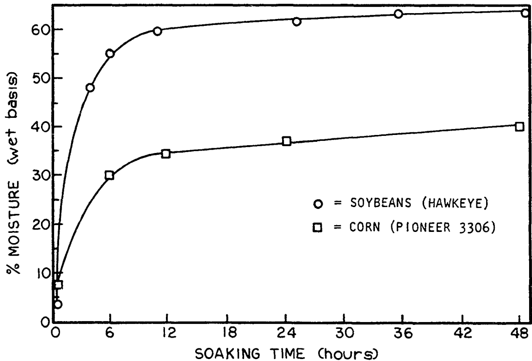
Figure 13. Moisture absorption curves at 85 degrees Fahrenheit for corn and soybean seeds immersed in tap water
