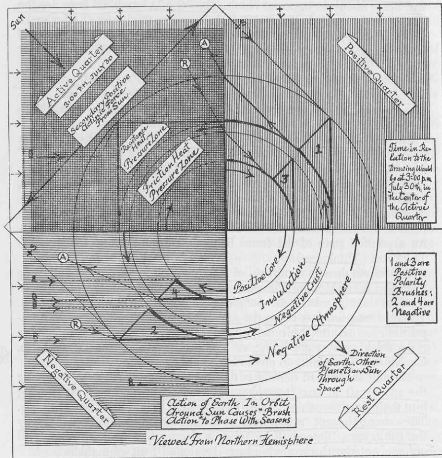
Rotation Principle Of The Earth
