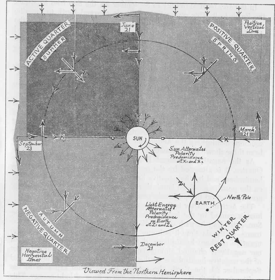
Orbit Principle Of The Earth
