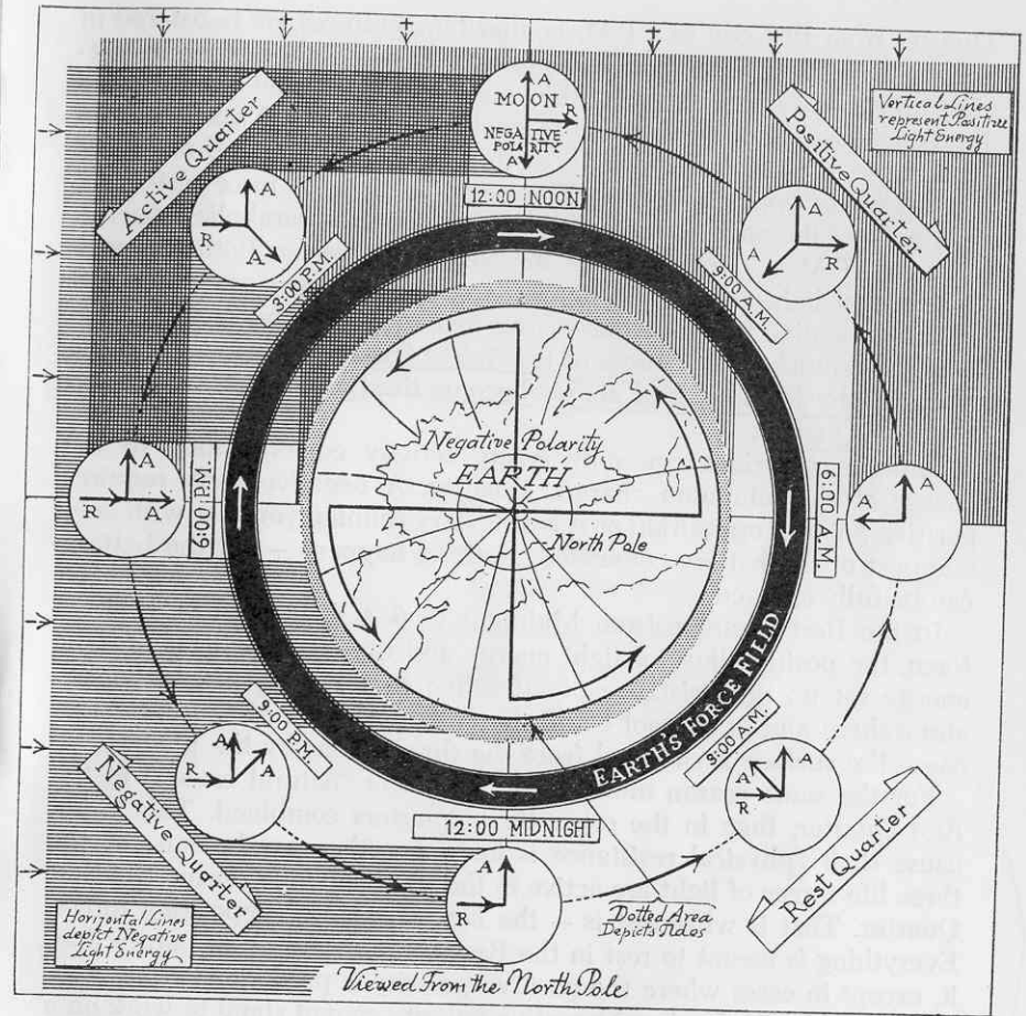
Orbit Principle Of The Moon
