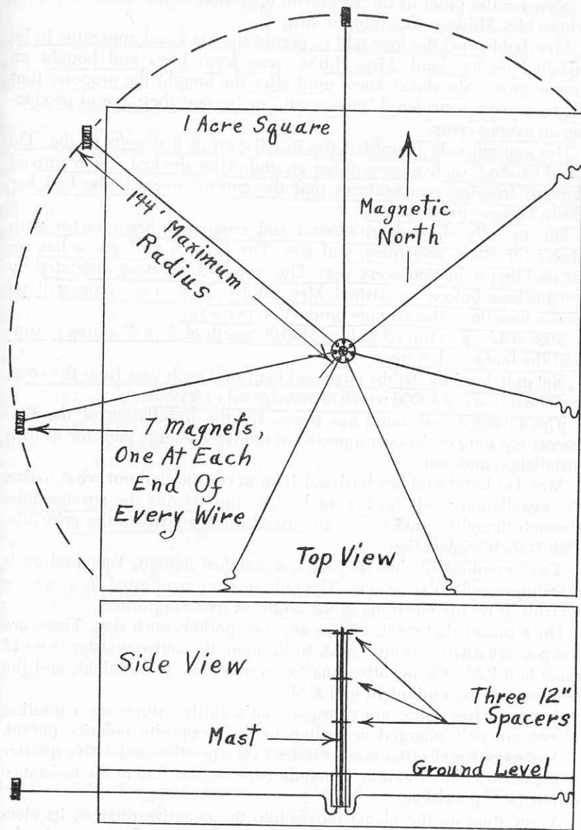
Figure 3 Anti Frost Control
