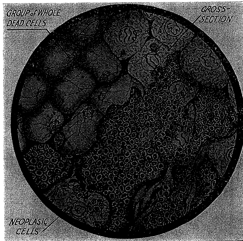
FIG. 3. — Diagram of a group of dead cells, not yet completely destroyed, in which neoplastic cells are forming. You will note, on the right, a region already completely transformed into neoplastic tissue.
