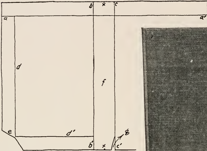
Fig. 17. Marking of cloth for Case Binding.
