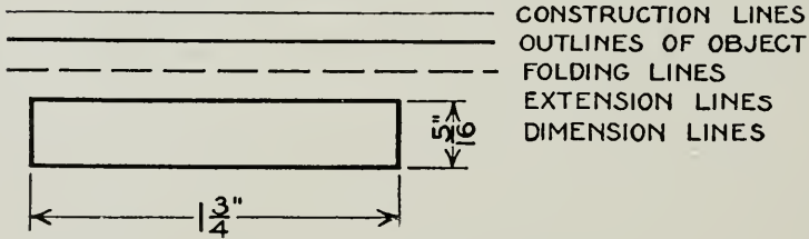
PLATE II. Line Conventions.
