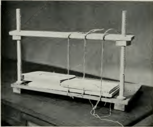
PLATE LVI. A sewing-frame in use.
