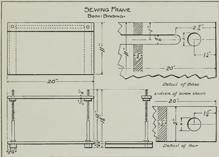
PLATE LV. Working drawing of sewing-frame.
