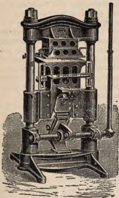
Fig. 64—Blocking press.
