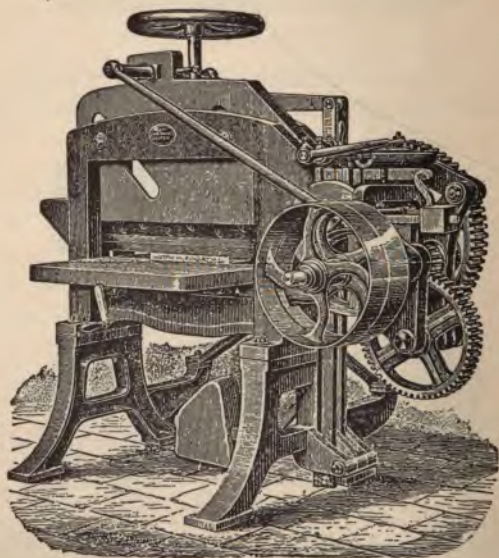
Fig. 35—Rotary guillotine.
