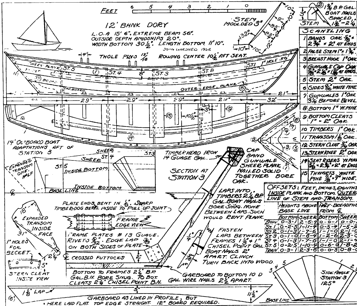
A 12-foot Bank dory.
