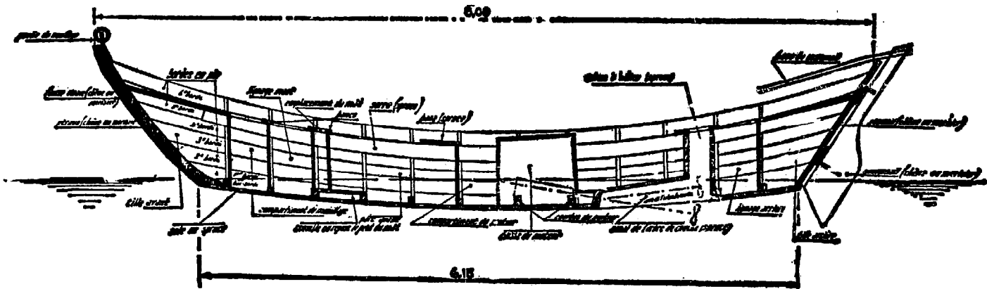
The original St. Pierre fishing dory.
