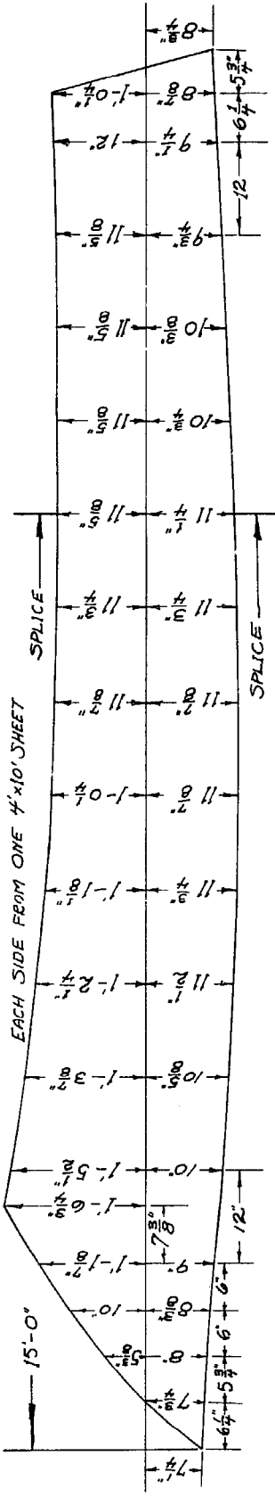
The plywood version of the 14' 4 1/2" outboard flatiron.
