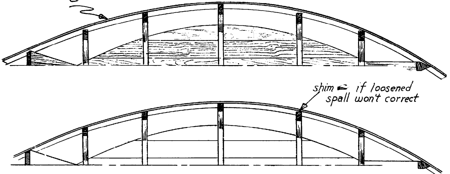
fairing batten
