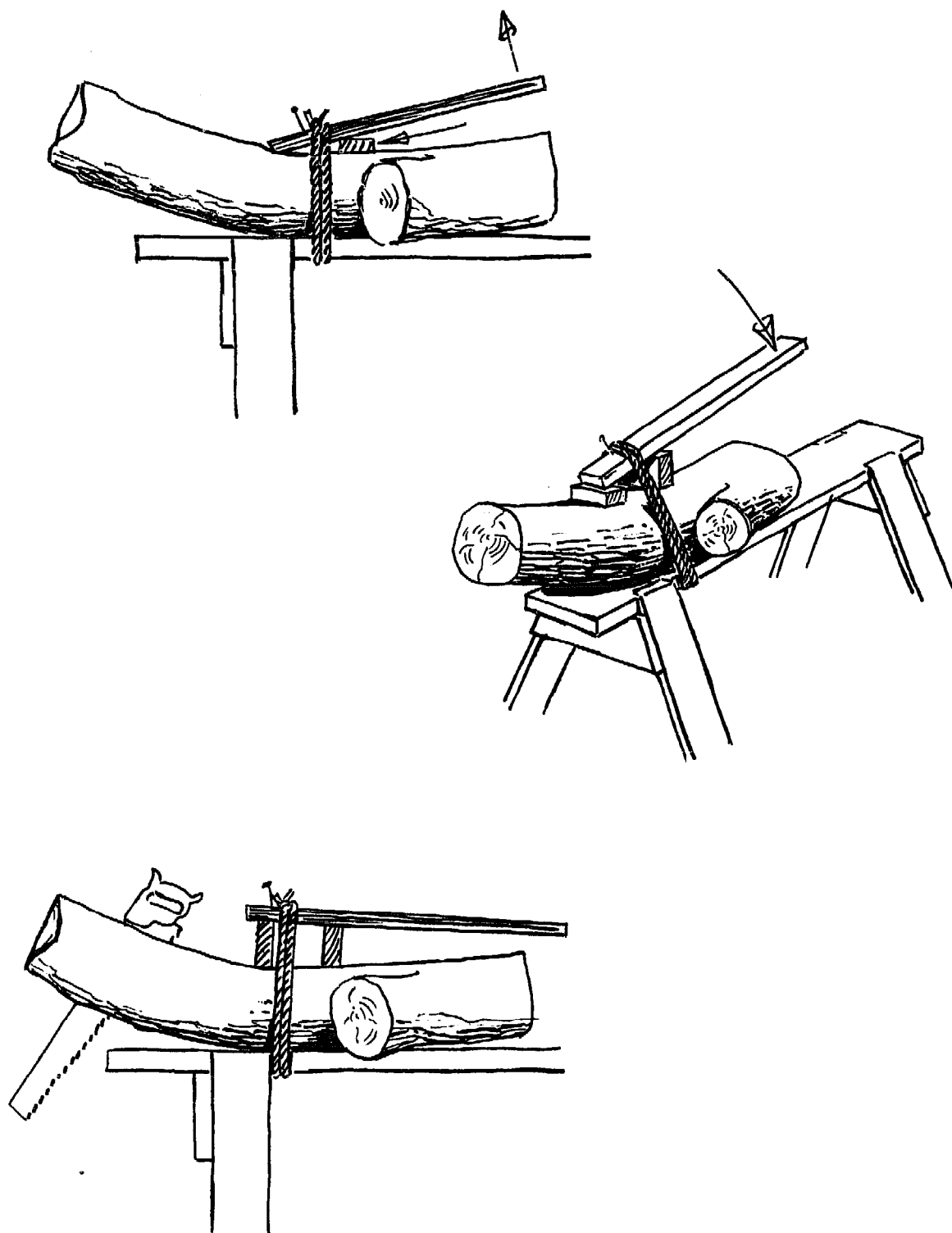
13. A "crusber" for clamping round or crooked wood. This works by levering up a fixed lashing of rope or chain while alternately increasing the size of the two fulcrums. This device exerts tremendous force, is stable under pressure, and can be quickly released.
