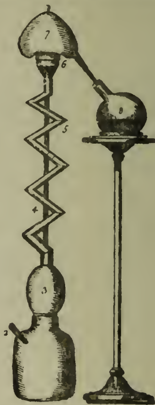
SERPENT CONDENSER Eighteenth century
