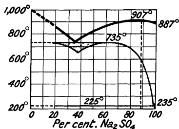
FIG. 117.—Freezing-point Curves of Mixtures of Sodium and Lead Sulphates.
