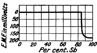
FIG. 23.—The Electromotive Force of Solution of Sb-Pb Alloys.
