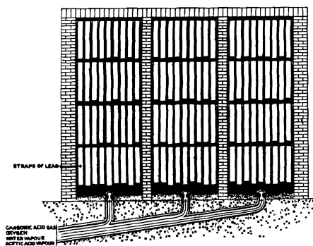
FIG. 124.—Arrangement of Lead for corrosion in the Chamber Process.
