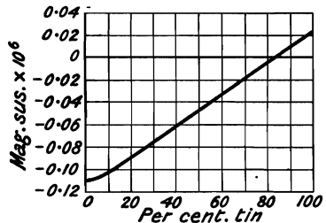
FIG. 61.—Magnetic Susceptibility of the Tin-Lead Alloys.
