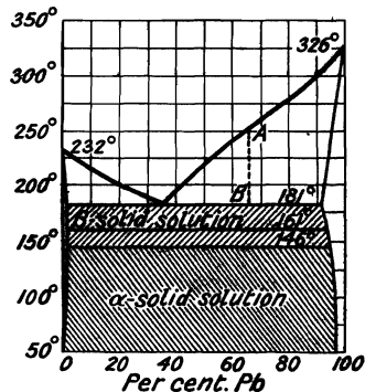
FIG. 55.—Freezing-point Curves of Lead-Tin Alloys.
