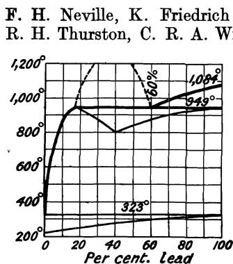
Fig. 33.—Freezing-point Curves of Lead-Copper Alloys.
