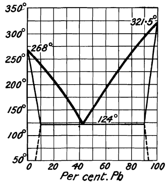
FIG. 26.—Freezing-point Curves of Bismuth-Lead Alloys.
