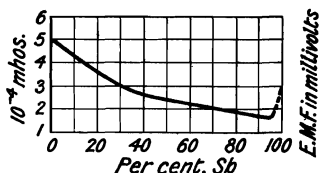
FIG. 22.—The Electrical Conductivity of the Sb-Pb Alloys.
