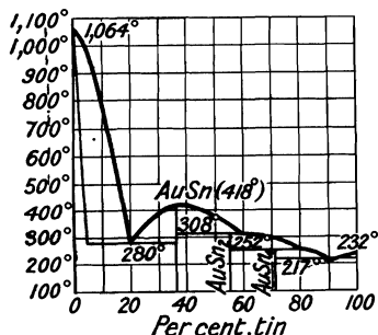
FIG. 46.—The Fusion Curves of the Sn-Au Alloys.
