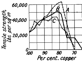
FIG. 35.—Tensile Strength of Bronzes.
