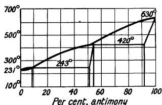
FIG. 20.—Fusion Curves of Binary Mixtures : Sn-Sb.
