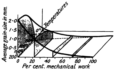
FIG. 7.—The Effect of Temperature and Mechanical Work on the Grain-size of Tin.
