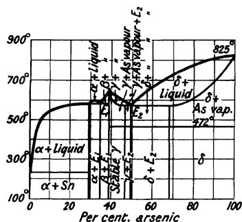
FIG. 18.—Fusion Curves of Binary Mixtures: As-Sn.
