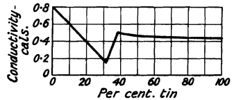
FIG. 37.—The Thermal Conductivity of Bronzes.
