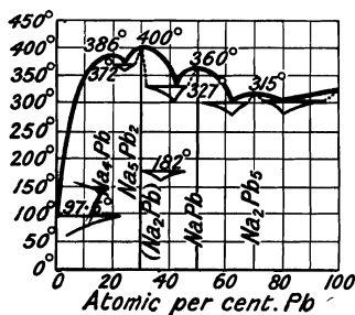
FIG. 31.—Freezing-point Curves of the Pb-Na Alloys.
