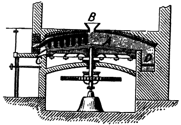
FIG. 2.—Roasting Furnace with Revolving Bed.
