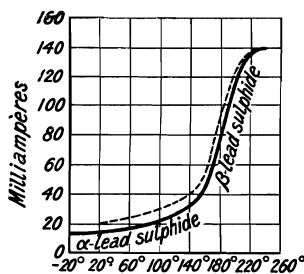
FIG. 105.—Electrical Conductivity of Galena Crystals.
