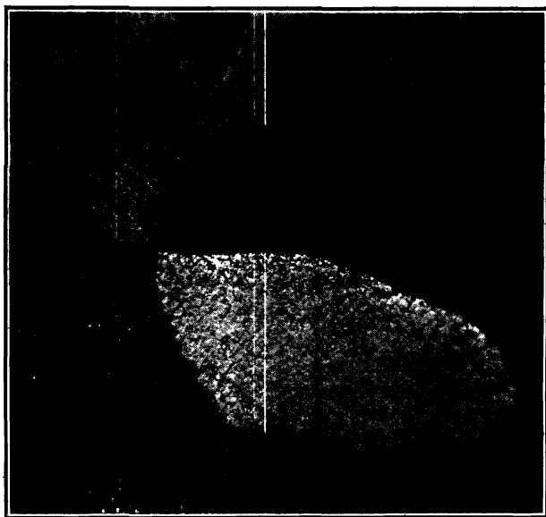
FIG. 8.—Lead etched with Acetic Acid ( \times 33 ).
