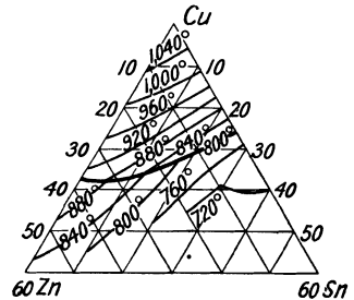
FIG. 43.—Melting-point Curves of Cu-Zn-Sn Alloys with over 60 per cent. of Copper.
