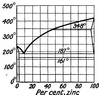
FIG. 50.—Fusion Curves of the Binary System: Sn-Zn.
