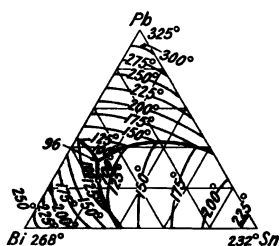
FIG. 62.—Fusion Curves of the Ternary System: Pb-Sn-Bi.
