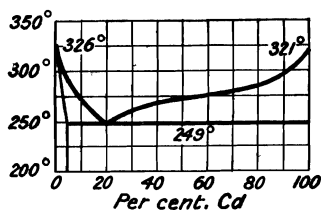
FIG. 43.—Freezing-point Curves of the Lead-Cadmium Alloys.
