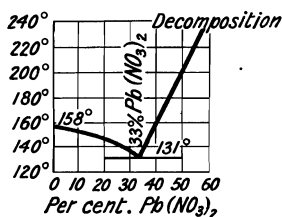
FIG. 128. — Freezing-point Curve of Lead and Ammonium Nitrates.
