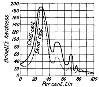
FIG. 34.—The Hardness of the Cu-Sn Alloys.
