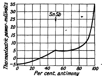
FIG. 24.—Thermoelectric Powers of the Sn-Sb Alloys.
