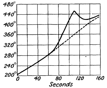
FIG. 3.—Heating Curve of Zirconium Oxide.
