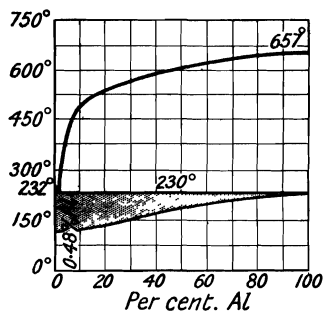
FIG. 59.—Fusion Curves of the Binary System: Al-Sn.
