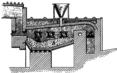
FIG. 4.—Flintshire Reverberatory Lead Furnace.
