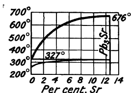
Fig. 38.—Freezing-point Curve of Mixtures of Lead and Strontium.
