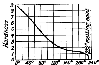
FIG. 13.—Hardness of Tin at Different Temperatures.
