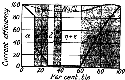
FIG. 42.—Electrolytic Corrosion of Bronzes by Aqueous Solutions of Sodium Sulphate and Chloride.
