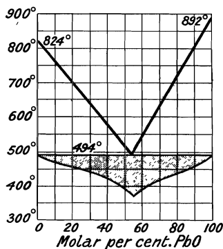
FIG. 68.—Freezing-point Curves of Mixtures of Lead Monoxide and Fluoride.
