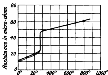
FIG. 17.—Electrical Resistance of Tin.
