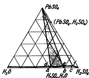
FIG. 111.—Equilibrium in the Ternary System: PbSO 4 –H 2 SO 4 –H 2 O at 0°.
