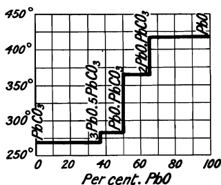
FIG. 121.—Equilibrium in the System \text{PbO-PbCO}_3\text{-H}_2\text{O} at Ordinary Temperatures.
