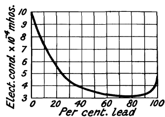
FIG. 51.—The Electrical Conductivity of Lead-Indium Alloys.
