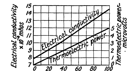
FIG. 54.—The Electrical Conductivity, and Thermoelectric Power of the Sn-Cd Alloys.
