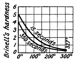
FIG. 11.—The Effect of Temperature on the Hardness of Lead.
