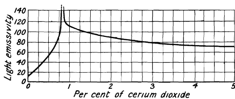
FIG. 5.—Effect of Cerium Dioxide on the Light Emissivity of Thoria.
