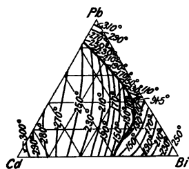
FIG. 45.—Freezing-point Curves of the Ternary System: Cd-Pb-Bi.
