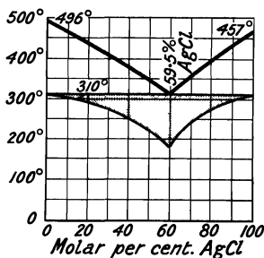
FIG. 83.—Freezing Points of Mixtures: \text{PbCl}_2\text{-AgCl} .
