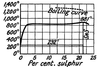
FIG. 78.—The Fusion Curve of Some Mixtures of Sulphur and Tin.
