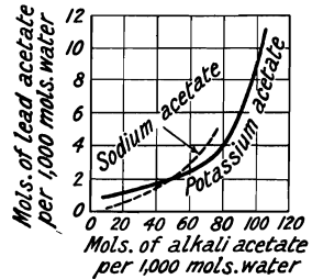
FIG. 112.—The Solubility of Lead Sulphate in Soln. of Potassium and Sodium Acetates.
