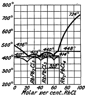
FIG. 82.—Freezing-point Curves of the Binary System: \text{PbCl}_2\text{-RbCl} .
