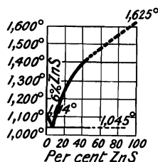
FIG. 109.—Freezing-point Curves of Lead and Zinc Sulphides.
