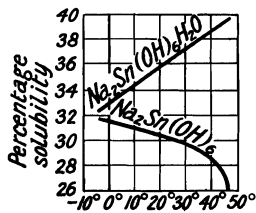
FIG. 65.—Solubility of Sodium Stannates.
