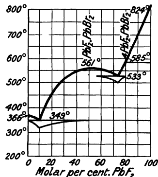
FIG. 94.—Freezing-point Curves of Mixtures of Lead Fluoride and Bromide.
