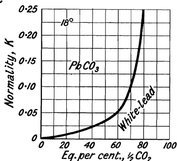
FIG. 126.—Equilibrium between Solutions of Potassium Carbonate and Lead Carbonate.
