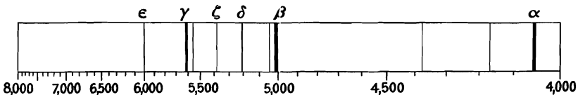
FIG. 12.—The Spark Spectrum of Lead.
