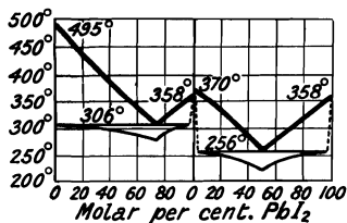
FIGS. 100 and 101.—Freezing-point Curves of Binary Mixtures of Lead Iodide with Lead Chloride and Bromide.
