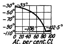
FIG. 73. — Freezing-point Curves of \text{Cl-SnCl}_4 Mixtures.
