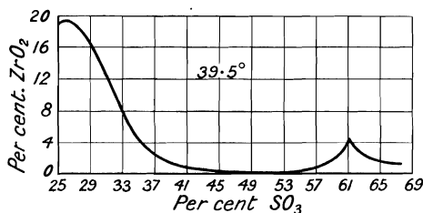
FIG. 6.—Solubility of Zirconium Oxide in Sulphuric Acid.
