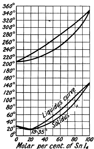
FIG. 77.—Freezing- and Boiling-point Curves of Mixtures of Stannic Iodide and Bromide.
