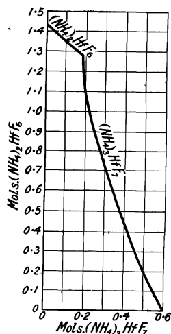
FIG. 3.—Mutual Solubilities of Ammonium Hexa- and Heptafluorhafnates.
