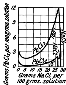
Figs. 75 and 76.—Phases in the Systems: \text{LiCl}-\text{PbCl}_2-\text{H}_2\text{O} , and \text{NaCl}-\text{PbCl}_2-\text{H}_2\text{O} .
