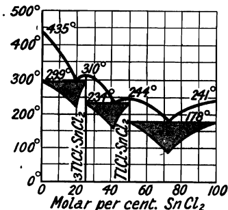
FIG. 72.—Freezing-point Curves of Mixtures of Thallos and Stannous Chlorides.
