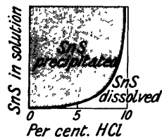
FIG. 79.—Effect of the Acidity of Solution on the Precipitation of Stannous Sulphide.
