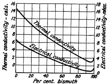
FIG. 26.—Thermal and Electrical Conductivities of the Tin-Bis- muth Alloys.
