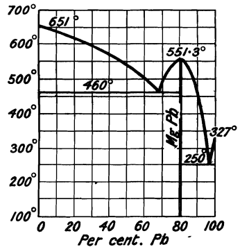
FIG. 40.—Freezing-point Curves of the Lead-Magnesium Alloys.
