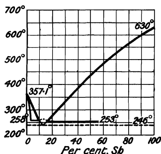
FIG. 21.—Freezing-point Curves of Mixtures of Antimony and Lead.
