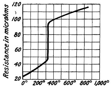
FIG. 13.—Electrical Resistance of Lead at Different Temperatures.
