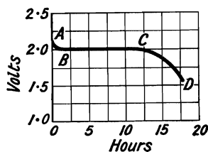
FIG. 14.—Voltage Drop of Accumulator.
