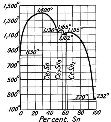
FIG. 63.—Freezing-point Curves of Tin-Cerium Alloys.
