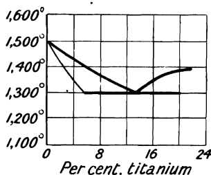
Fig. 5.—Freezing Points of the Iron-Titanium Alloys.
