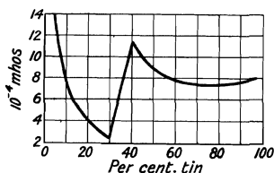
FIG. 38.—The Electrical Conductivity of Bronzes.
