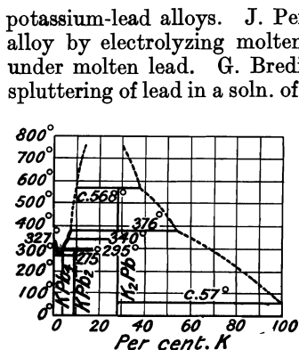
FIG. 32.—Freezing-point Curves of the Pb-K Alloys.
