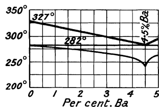
Fig. 39.—Freezing-point Curve of Some Barium-Lead Alloys.
