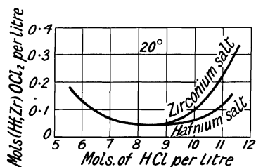
FIG. 4.—The Effect of Hydrochloric Acid on the Solubilities of Zirconium and Hafnium Oxochlorides.
