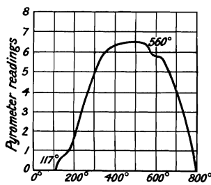
FIG. 1.—Heating and Cooling Curves of Germanium.
