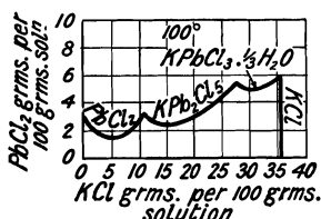
FIGS. 78 and 79.—Solubility of Lead Chloride in Solutions of Potassium Chloride at Different Concentrations.
