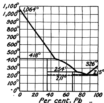
FIG. 36.—Freezing-point Curves of the Lead-Gold Alloys.
