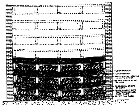
FIG. 122.—Diagrammatic Arrangements in the Stack Process.
