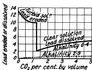
FIG. 15.—The Effect of Carbon Dioxide on the Corrosion of Lead.
