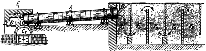
FIG. 3.—Roasting Furnace with Revolving Cylinder.
