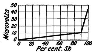
FIG. 24.—The Thermo-electric Force of Sb-Pb Alloys.
