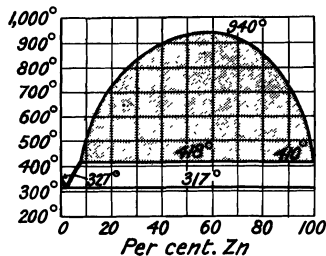
FIG. 42.—Freezing-point Curves of the Lead-Zinc Alloys.
