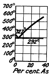
FIG. 20.—Fusion Curves of As-Pb Alloys.
