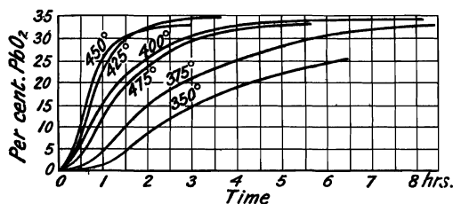
FIG. 66.—Speeds of Oxidation of Lead Monoxide (as PbO_2 ) at Different Temperatures.
