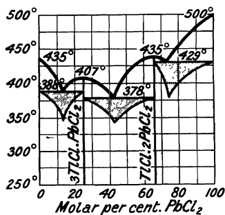
FIG. 90.—Freezing-point Curves of Mixtures of Thalious and Lead Chlorides.
