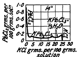
FIGS. 78 and 79.—Solubility of Lead Chloride in Solutions of Potassium Chloride at Different Concentrations.
