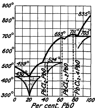
FIG. 93.—Freezing-point Curves of Mixtures of Lead Monoxide and Dichloride.
