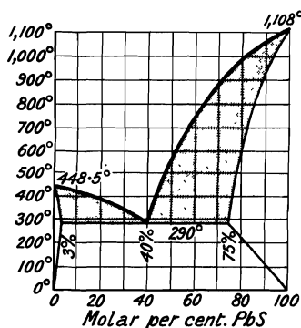
FIG. 110.—Equilibrium Diagram of Thallium and Lead Sulphides.
