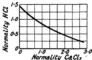
FIG. 30.—Concentration of Hydrochloric Acid required to prevent the Precipitation of Lead Sulphide.
