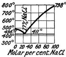
Figs. 73 and 74.—Freezing-point Curves of Mixtures of Lead Chloride with Lithium or Sodium Chloride.
