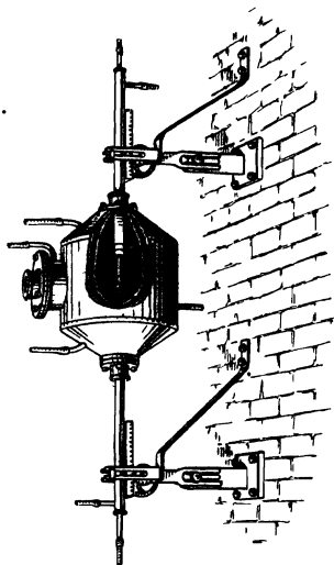
FIG. 1.—L. Weiss and E. Neumann's Vacuum Arc-Furnace.
