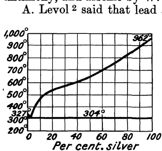
Fig. 34.—Freezing-point Curves of the Lead-Silver Alloys.
