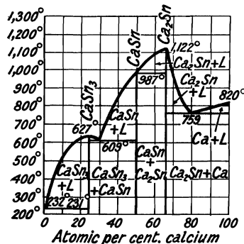
FIG. 47.—The Fusion Curves of the Ca-Sn Alloys.
