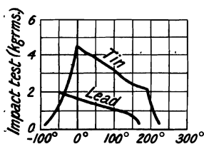
FIG. 14.—Impact Tests on Tin and Lead.
