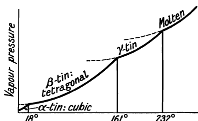
FIG. 11.—Equilibrium of the Allotropic Forms of Tin (Diagrammatic).†
