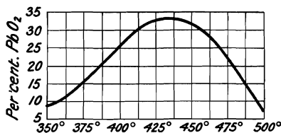
FIG. 67.—Proportion of Red-lead (as \text{PbO}_2 ) formed from Lead Monoxide at Different Temperatures.
