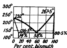
FIG. 25.— Fusion Curves of Bi- nary Mixtures Sn-Bi.
