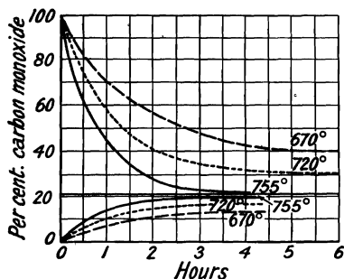
FIG. 64.—Equilibria in the Reaction \text{Sn} + 2\text{CO}_2 \rightleftharpoons \text{SnO}_2 + 2\text{CO} .
