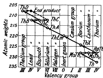
FIG. 4.—Arrangement of the Thorium Decay Products in the Periodic Table.
