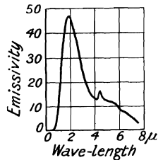
FIG. 4.— Ultra-red Emission Spectrum of Zirconia.
