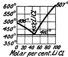
Figs. 73 and 74.—Freezing-point Curves of Mixtures of Lead Chloride with Lithium or Sodium Chloride.
