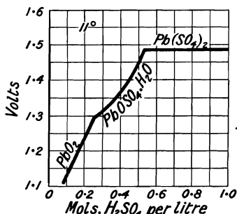
FIG. 119.—Electromotive Force of Solutions of \text{Pb}(\text{SO}_4)_2 in Sulphuric Acid at 11^\circ .
