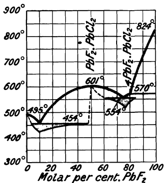
FIG. 92.—Freezing-point Curves of Mixtures of Lead Fluoride and Chloride.
