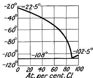
FIG. 9.—Freezing-point Curves of \text{Cl}_2 — \text{TiCl}_4 Mixtures.
