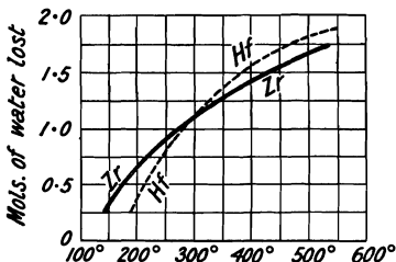
FIG. 7.—The Effect of Temperature on the Reaction: RO(H_2PO_4)_2 \rightarrow RO(PO_3)_2 .
