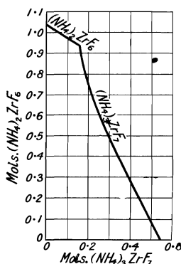
FIG. 5.—The Mutual Solubilities of Ammonium Hexa- and Hepta-fluozirconates.
