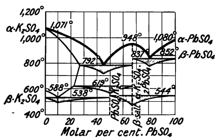
FIG. 115.—Freezing-point Curves of Lead and Potassium Sulphates.
