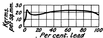
FIG. 53.—The Pressure of Flow of the Thallium-Lead Alloys.
