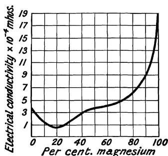
FIG. 41.—The Electrical Conductivity of Lead-Magnesium Alloys.
