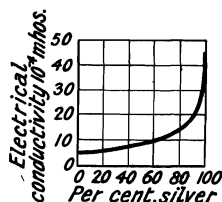
FIG. 35.—The Electrical Conductivity of Silver-Lead Alloys.
