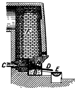
FIG. 5.—Ore Hearth.
