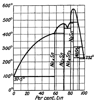
FIG. 30.—Equilibrium Curves of the Sodium-Tin Alloys.
