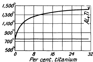
FIG. 4.—Freezing-point Curves of Aluminium-Titanium Alloys.
