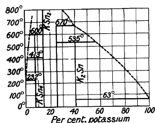
FIG. 29.—Equilibrium Curves of the Potassium-Tin Alloys.
