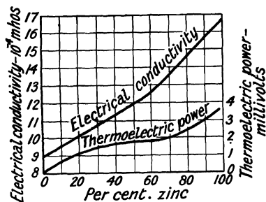
FIG. 52.—The Electrical Conductivity and Thermoelectric Power of the Sn-Zn Alloys.
