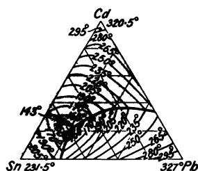
FIG. 63.—Fusion Curves of the Ternary System: Pb-Sn-Cd.
