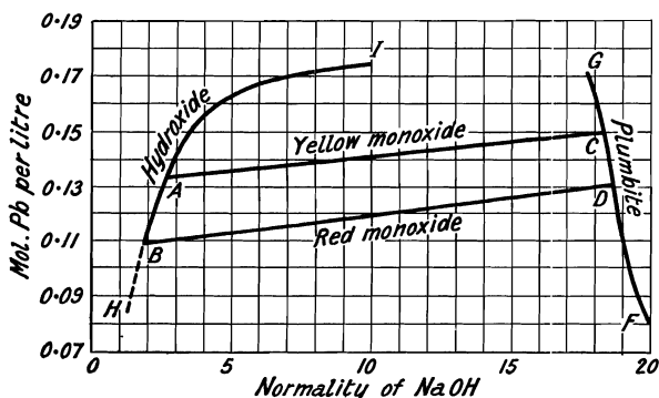
FIG. 64.—Equilibrium Diagram for the System PbO-H 2 O-NaOH.
