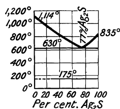
FIG. 108.—Freezing-point Curves of Mixtures of Lead and Silver Sulphides.
