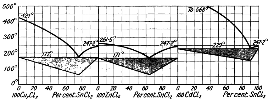
FIG. 69.—Fusion Curves of the System: Cu_2Cl_2-SnCl_2 .
