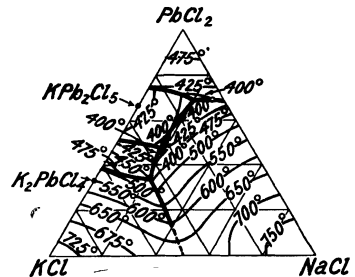
FIG. 81.—Fusion Curves in the Ternary System: \text{KCl}-\text{NaCl}-\text{PbCl}_2 .
