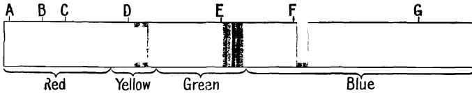
FIG. 1.—Absorption Spectrum of Monazite.
