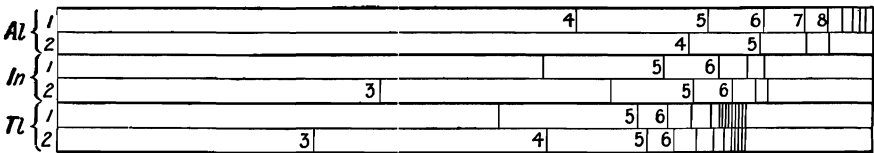
FIG. 27.—Series Spectra of Aluminium, Indium, and Thallium.
