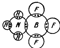
FIG. 5.—Electronic Structure of BF_3.NH_3 .
