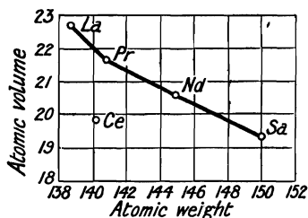
FIG. 7.—Atomic Volumes of the Cerium Metals.
