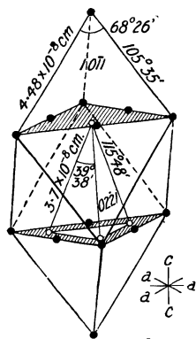
FIG. 13.—Space Lattice of Graphite (P. Debye and P. Scherrer).
