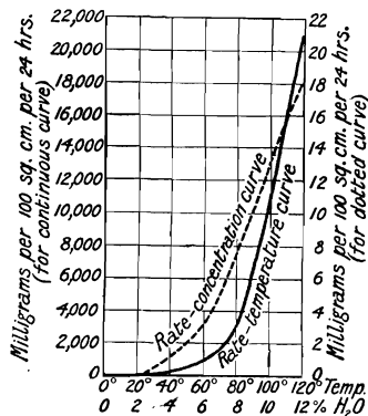
FIG. 29.—Effect of Temperature and Concentration on the Rate of Dissolution of Aluminium in Nitric Acid.
