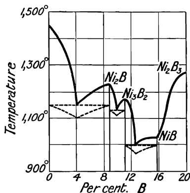
Fig. 7.—Freezing-point Curve of Mixtures of Nickel with up to 20 per cent. of Boron.
