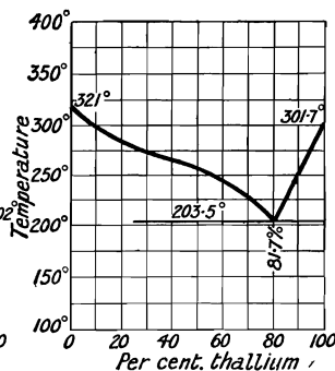
FIG. 13.—Freezing-point Curve of Alloys of Cadmium and Thallium.
