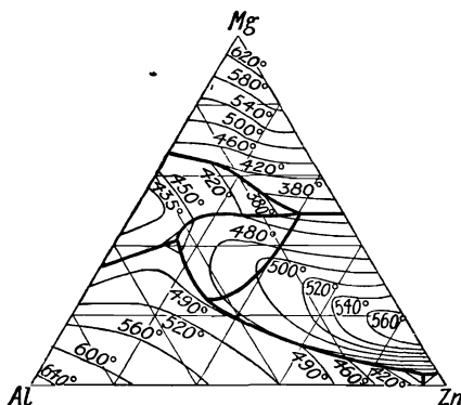
FIG. 44.—Isothermal Lines in the Equilibrium Diagram of the Ternary System, Zn—Mg—Al.
