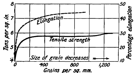
FIG. 21.—Effect of Grain-size on the Tensile Properties of Aluminium.
