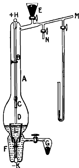
FIG. 1.—E. Weintraub's Mercury Arc Furnace.
