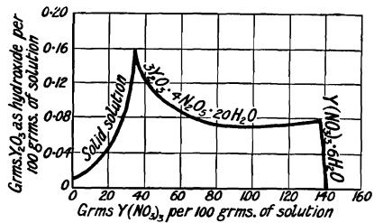
FIG. 26.—The Ternary System, \text{Y}_2\text{O}_3 - \text{N}_2\text{O}_5 - \text{H}_2\text{O} , at 25°.
