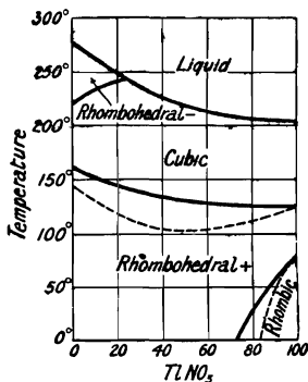
FIG. 30.—Transformations with Thallous and Rubidium or Caesium Nitrates.
