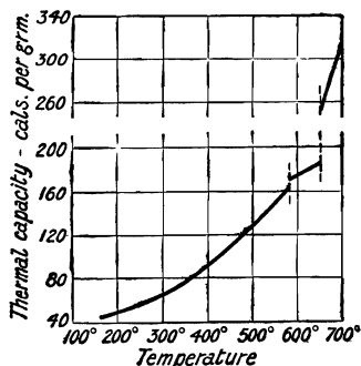
FIG. 23.—Thermal Capacity of Aluminium at Different Temperatures.
