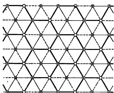
FIG. 14.—Arrangement of Atoms in Graphite.
