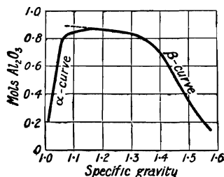
FIG. 48.—Precipitation of Alumina from Solution in Sodium Hydroxide.
