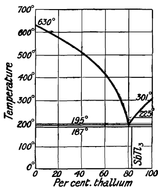
FIG. 3.—Freezing-point Curve of Thallium-Antimony Alloys.
