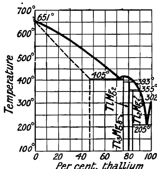
FIG. 11.—Freezing-point Curve of Alloys of Magnesium and Thallium.
