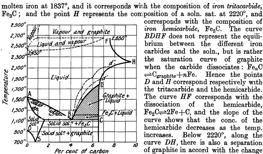
FIG. 31.—The Solubility of Carbon in Iron.
