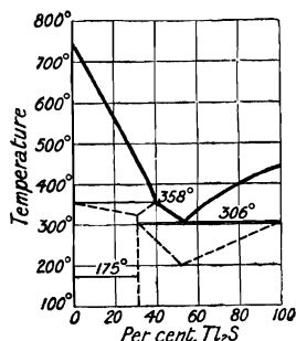
Fig. 25.—Equilibrium Diagram of the Binary System, \text{Ag}_2\text{S}-\text{Tl}_2\text{S} .
