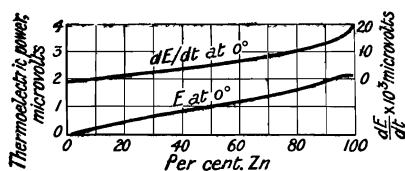
FIG. 42.—Thermoelectric Power, E , at 0° of Zinc-Aluminium Alloys.
