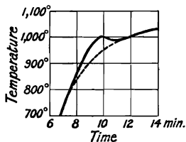
FIG. 51.—Portion of Heating Curve of Alumina showing Exothermal Change starting about 850°.
