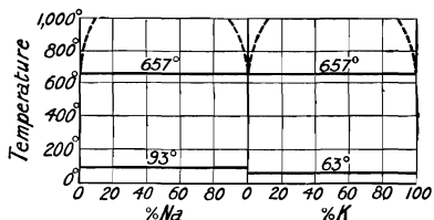
FIGS. 30 and 31.—Freezing-point Curves of Binary Mixtures of Aluminium with Sodium and Potassium.
