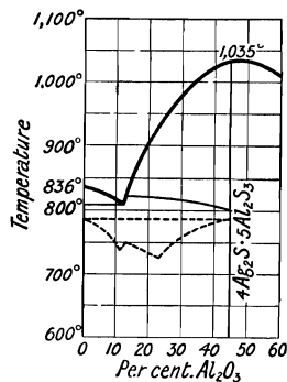
FIG. 62.—Freezing-point Curves of Silver and Aluminium Sulphides.
