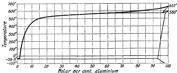
Fig. 46.—Freezing-point Curve of Mixtures of Mercury and Aluminium.
