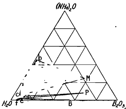
FIG. 22.—Equilibrium in the Ternary System, (NH_4)_2O-B_2O_3-H_2O , at 30^\circ .
