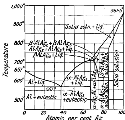
FIG. 33.—Freezing-point Curve of Mixtures of Silver and Aluminium.
