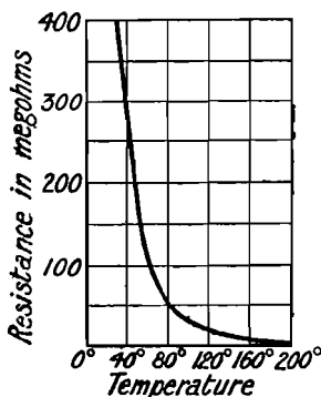
FIG. 3.—The Electrical Resistance of Boron.
