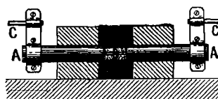
FIG. 10.—W. Borchers' Resistance Furnace
