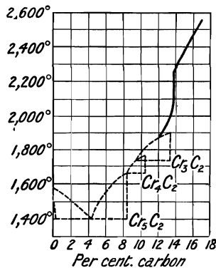
FIG. 29.—Part of Freezing-point Curve of the Chromium-Carbon System.
