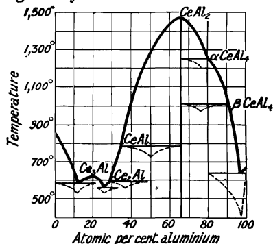
FIG. 15.—Freezing-point Curve of Aluminium-Cerium Alloys.
