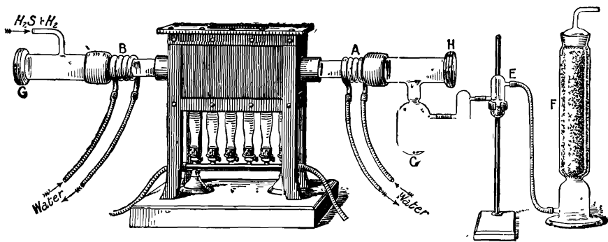
FIG. 33.—The Preparation of Boron Trisulphide.
