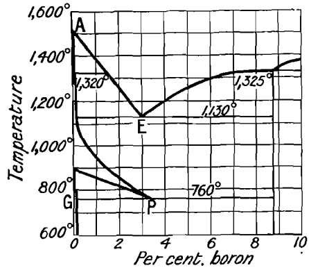
Fig. 6.—Freezing-point Curve of Mixtures of Iron and Boron.
