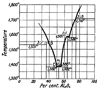
FIG. 54.—Freezing-point Curve of the Binary System, \text{CaO}-\text{Al}_2\text{O}_3 .
