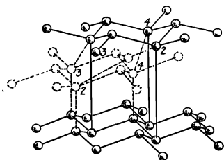
FIG. 15.—Lattices of Graphite (continuous lines), and of Diamond (lower continuous and middle dotted lines).
