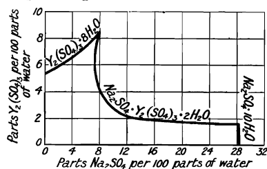
FIG. 25.—The Ternary System, Y_2(SO_4)_3 - Na_2SO_4 - H_2O , at 25°.
