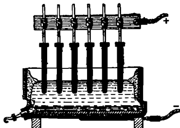
FIG. 2.—Cell for the Electrolysis of a Solution of Alumina in Fused Cryolite (Diagrammatic).
