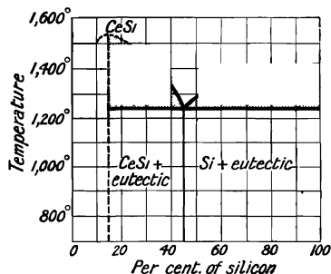
FIG. 12.—Freezing-point Curve of Alloys of Silicon and Cerium.
