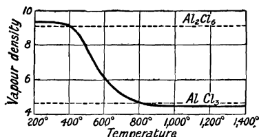
Fig. 60.—Effect of Temperature on the Vapour Density of Aluminium Chloride.
