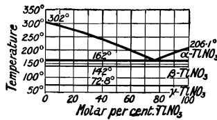
FIG. 28.—Freezing-point Curve of Mixtures of Thallous and Sodium Nitrates.
