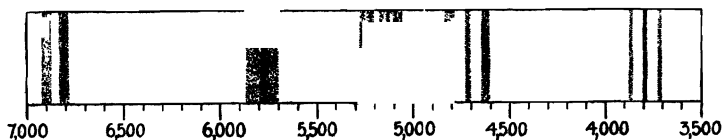
FIG. 9.—The Absorption Spectrum of Aqueous Solutions of Neodymium Chloride.
