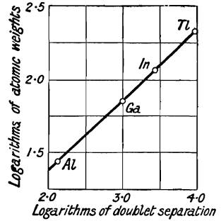
FIG. 26.—Relationship between the Spectral Lines and the Atomic Weights of Al, Ga, In, Tl.
