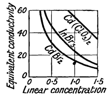
FIG. 2.—Equivalent Conductivity and Linear Concentration of Solutions of Indium and Cadmium Bromides.
