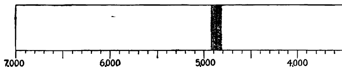
FIG. 28.—Absorption Spectrum of Terbium Nitrate Solution.
