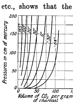
FIG. 18. — Equilibrium Pressures of Carbon Dioxide adsorbed by Charcoal.
