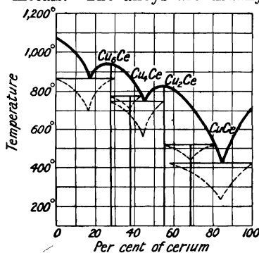
FIG. 13.—Freezing-point Curve of Copper-Cerium Alloys.
