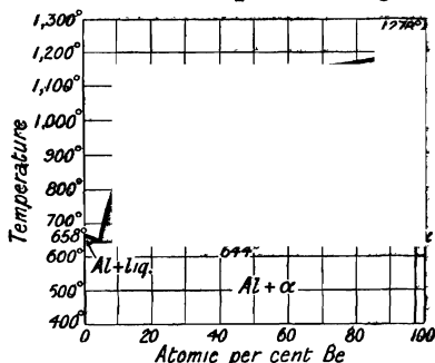
FIG. 36.—Freezing-point Curve of Mixtures of Beryllium and Aluminium.
