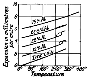
FIG. 40.—Thermal Expansion of Zn-Al Alloys.
