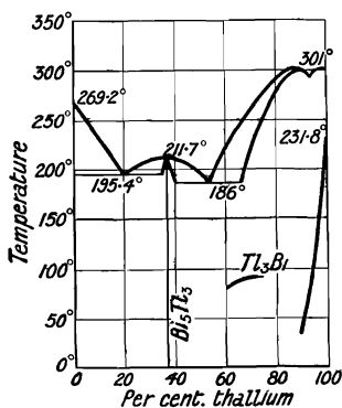
FIG. 4.—Freezing-point Curve of Thallium-Bismuth Alloys.
