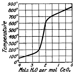
FIG. 18.—Dehydration Curve of Ceric Hydroxide.
