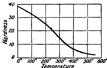
FIG. 17.—The Variation of the Hardness of Aluminium with Temperature.
