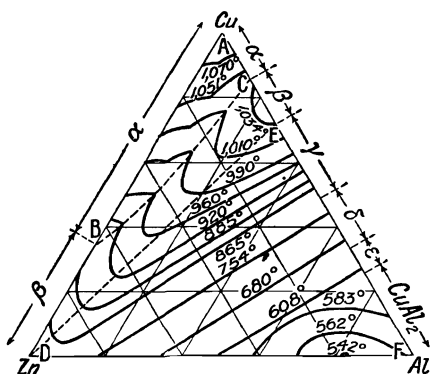
FIG. 43.—Isothermal Lines in the Equilibrium Liquidus Diagram of the Ternary System, Cu—Zn—Al.
