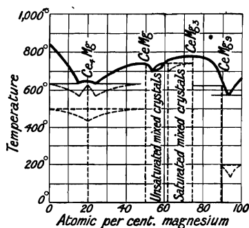
FIG. 14.—Freezing-point Curve of Magnesium-Cerium Alloys.
