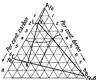
FIG. 32.—Ternary System Fe—C—B.
