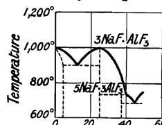
Fig. 57.—Freezing Curves of Mixtures of Aluminium and Sodium Fluorides.
