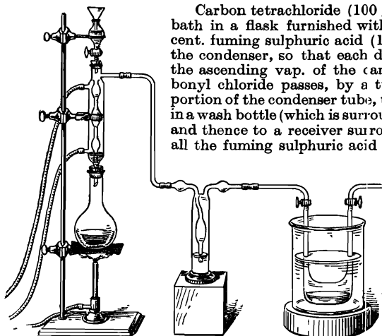
FIG. 40.—H. Erdmann's Process for Preparing Phosgene.
