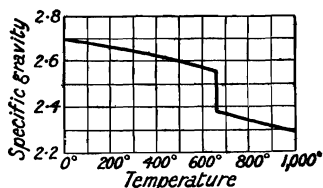
FIG. 16.—Specific Gravity of Aluminium at Different Temperatures.
