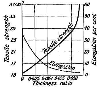
FIG. 18.—Effect of Cold-working on the Tensile Properties of Aluminium.
