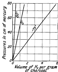
FIG. 17. — Equilibrium Pressures of Hydrogen adsorbed by Charcoal.
