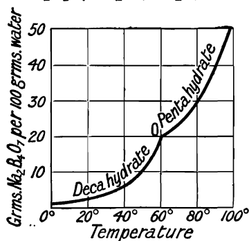
FIG. 16.—Solubility Curve of Borax in Water.
