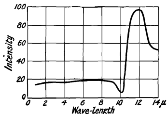
FIG. 26.—Ultra-red Absorption Spectrum of Carborundum.
