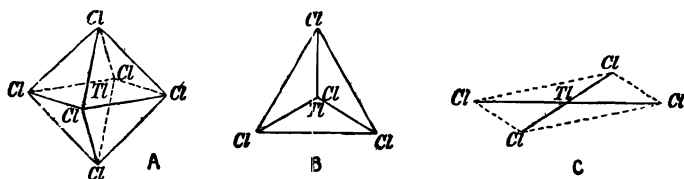
FIGS. 16-18.—A. Werner's Nuclei for [\text{TI} \text{Cl}_6] \text{TI}_3' and [\text{TI} \text{Cl}_4] \text{TI}' .
