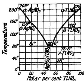
FIG. 31.—Freezing-point Curves of Mixtures of Thallous and Silver Nitrates.
