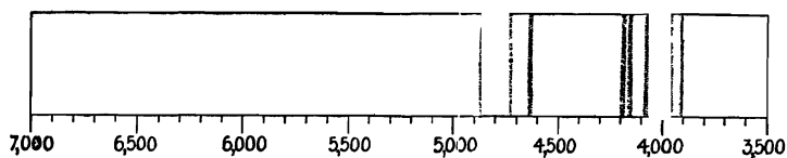
FIG. 10.—Absorption Spectrum of Samarium Chloride.
