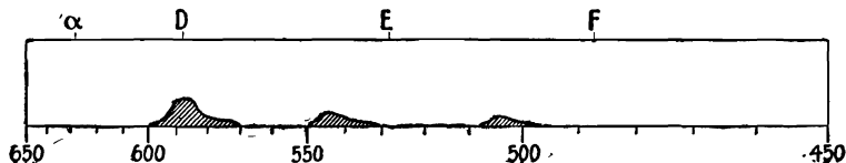
FIG. 25.—Absorption Spectrum of Alkanna and Aluminium Chloride.
