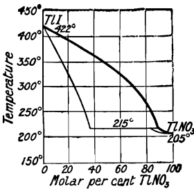
FIG. 27.—Freezing-point Curve of Thallous Iodide and Nitrate.
