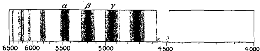
FIG. 2.—Spectrum of Boric Acid.
