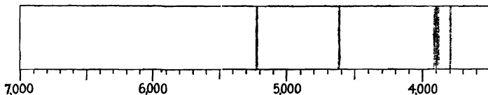
FIG. 27.—Absorption Spectrum of Europium Nitrate Solution.
