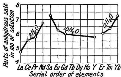
FIG. 5.—Solubilities of the Rare Earth Bromonitrobenzenesulphonates.
