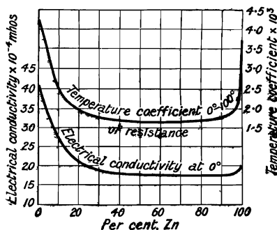
FIG. 41.—Electrical Conductivity, and Temperature Coefficient of Resistance of Zinc Aluminium Alloys.
