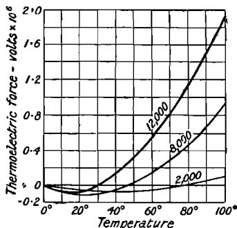
Fig. 28.—Thermo-electric Force of a Couple composed of Compressed and Uncompressed Aluminium.
