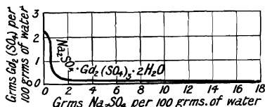
FIG. 29.—Solubility of Gadolinium Sulphate in Solutions of Sodium Sulphate.
