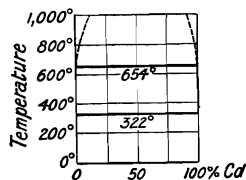
Fig. 45.—Freezing-point Curves of Cadmium-Aluminium Alloys.
