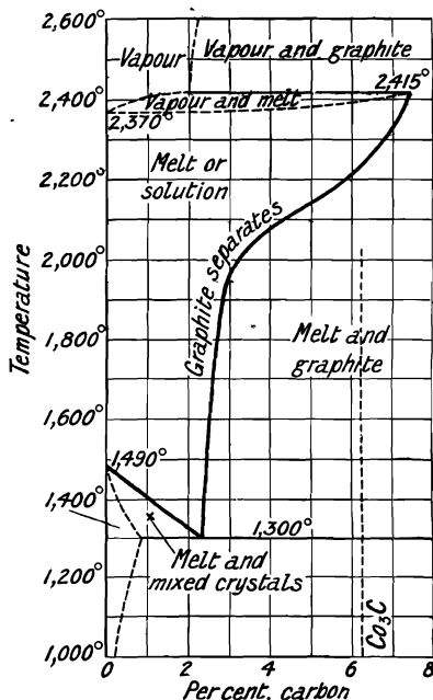
FIG. 34.—The Solubility of Carbon in Cobalt.
