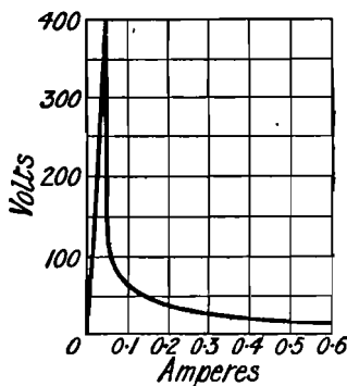
FIG. 4.—Volt-Ampere Curve of Boron in Air.
