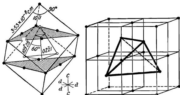
FIGS. 11-12.—Space Lattice of Diamond (P. Debye and P. Scherrer).
