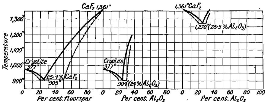
FIG. 3.—Melting Points of Mixtures of Cryolite and Fluorspar. FIG. 4.—Melting Points of Mixtures of Alumina and Cryolite. FIG. 5.—Melting Points of Mixtures of Alumina and Fluorspar.
