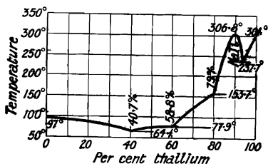
FIG. 5.—Freezing Points of Alloys of Thallium and Sodium.
