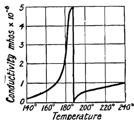
Fig. 61.—Electrical Conductivity of Aluminium Chloride.
