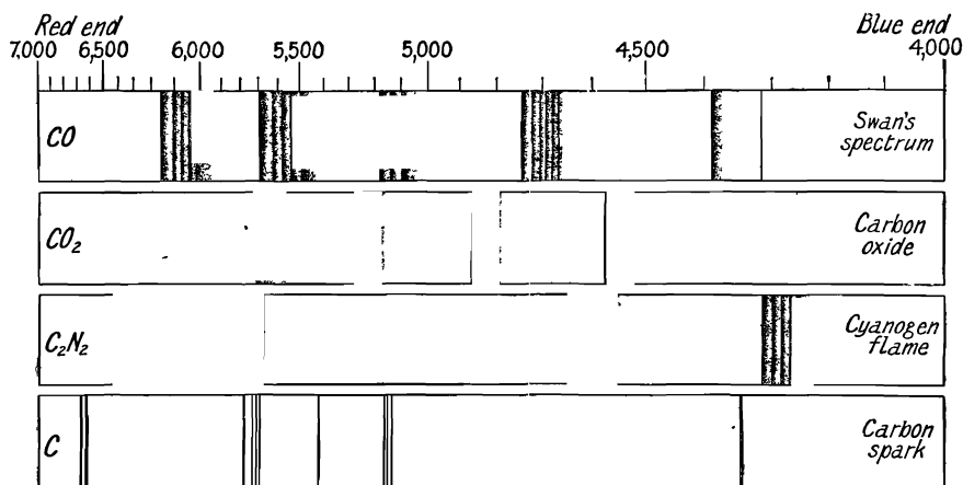
FIG. 16.— Spectra of Carbon and its Oxides, and of Cyanogen.
