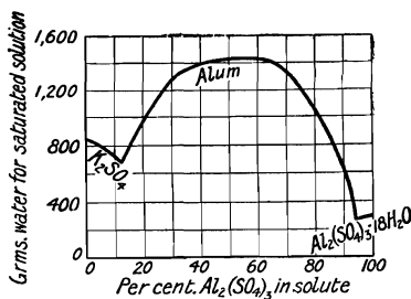
FIG. 67.—The Ternary System, K_2SO_4 - Al_2(SO_4)_3 - H_2O , at 25°.
