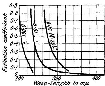
FIG. 106.—Effect of Wave-length on the Extinction Coefficient of Solutions of Potassium Persulphate.
