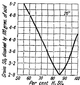
FIG. 51.—The Solubility of Sulphur Dioxide in Sulphuric Acid.
