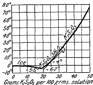
FIG. 72.—Solubility of Potassium Pyrosulphite.
