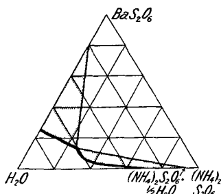
FIG. 132.—Ternary System (NH 4 ) 2 S 2 O 6 –BaS 2 O 6 –H 2 O, at 30°.
