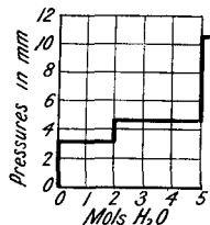
Fig. 115.—Vapour Pressure of Hydrated Sodium Thiosulphate.
