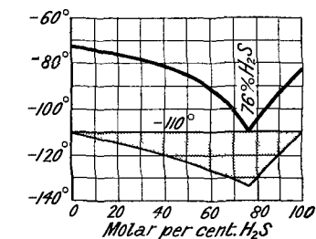
FIG. 37.—Freezing-point Curve of the System: \text{SO}_2\text{-H}_2\text{S} .
