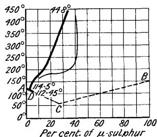
FIG. 10.—The Effect of Temperature on the Equilibrium Proportions of S_\lambda and S_\mu .
