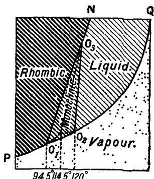
FIG. 6.—Vapour Pressure of Sulphur (Diagrammatic).
