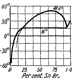
FIG. 54.—The Binary System : \text{SO}_2\text{-SnBr}_4 .
