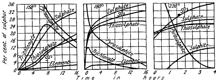
FIGS. 69, 70, and 71.—Percentage of Different Forms of Combined Sulphur present at Different Temperatures.
