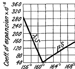
FIG. 21.—The Thermal Expansion of Viscid Sulphur.
