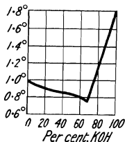
FIG. 50.—Effect of N -KOH on the Lowering of the Freezing Point of 2 N - \text{H}_2\text{SeO}_3 .
