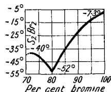
Fig. 140.—Portion of Melting-point Curve of Bromine and Sulphur.
