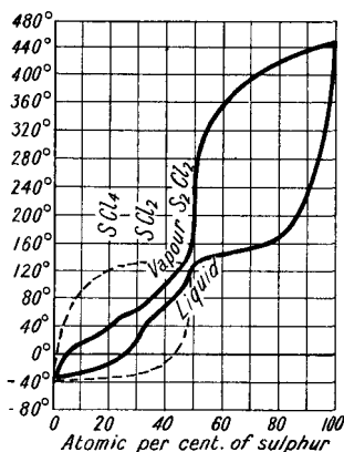
FIG. 138.—The Composition of Binary Mixtures of Sulphur and Chlorine—Liquid and Vapour—at the Boiling Point.
