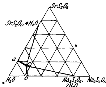
FIG. 131.—Ternary System : Na 2 S 2 O 6 –SrS 2 O 6 –H 2 O, at 30°.
