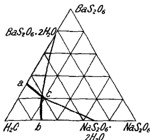
FIG. 133.—Ternary System : \text{Na}_2\text{S}_2\text{O}_6 - \text{BaS}_2\text{O}_6 - \text{H}_2\text{O} , at 30°.
