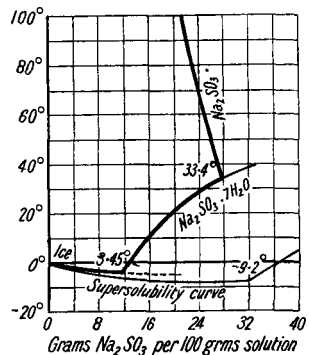
FIG. 61.—Solubility Curves of Sodium Sulphite.
