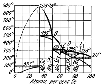
FIG. 33.—Freezing-point Curve of the Binary System: Sodium-Selenium.
