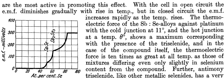
FIG. 44.—Electromotive Force of the \text{Sb} \mid \text{SbCl}_3 \mid \text{SbSe}_n -cell.
