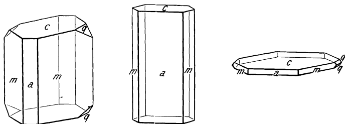
FIG. 7.—Crystals of \beta -monoclinic Selenium.
