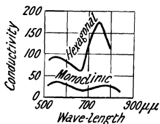
FIG. 23. — Effect of Light of Different Wave-length on the Conductivity of Selenium Crystals.
