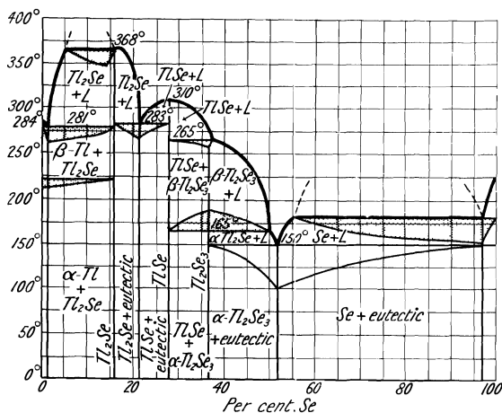
FIG. 40.—Melting-point Curve of the Binary System: Selenium-Thallium.
