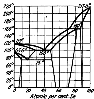
FIG. 64.—Melting Points of Mixtures of Selenium and Sulphur.
