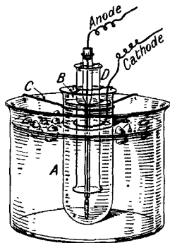
FIG. 104.—The Preparation of Potassium Persulphate.
