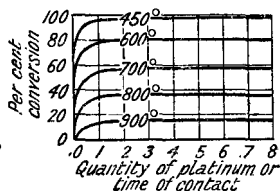
FIG. 74.—Relation between Conversion and Times of Reaction at various Temperatures.
