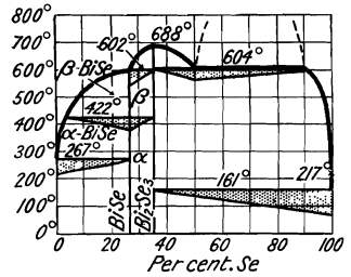
FIG. 45.—Freezing-point Curves of the Binary System: Bi-Se.
