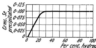
FIG. 1.—Influence of Acidity of Solution on the Precipitation of Selenium.
