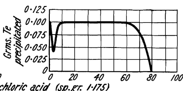
FIG. 2.—Influence of Acidity of Solution on the Precipitation of Tellurium.
