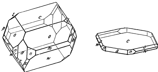
FIG. 6.—Crystals of \alpha -monoclinic Selenium.
