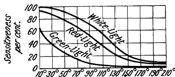
FIG. 20.—The Effect of Temperature on the Sensitiveness of Selenium to White, Red, and Green Light.
