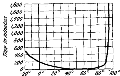
FIG. 5.—The Effect of Temperature on the Rate of Transformation of \beta - to \alpha -Sulphur.
