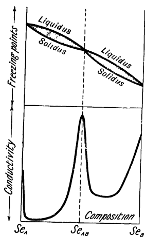
FIG. 5.—Freezing-point, and Electrical Conductivity Curves of Selenium quenched from Different Temperatures.
