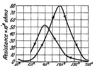
FIG. 12.—Electrical Resistance on a Rising and a Falling Temperature.
