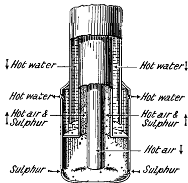
FIG. 4.—H. Frasch's Sulphur Pump.
