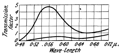
FIG. 9.—Spectral Transmission of Selenium-coloured Glass.
