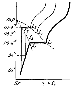
FIG. 8.—Effect of S_\mu on the Melting Point of S_r .
