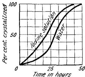
FIG. 9.—Speed of Crystallization of Plastic Sulphur, under Water, and under a \frac{1}{10} N-solution of Iodine.
