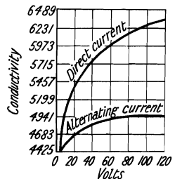
FIG. 26.—The Effect of Impressed Electromotive Force on the Resistance of Selenium.
