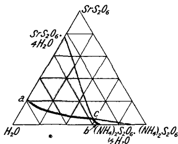
Fig. 130.—Ternary System : (\text{NH}_4)_2\text{S}_2\text{O}_6 — \text{SrS}_2\text{O}_6 — \text{H}_2\text{O} at 30^\circ .
