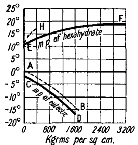
FIG. 48.—The Effect of Pressure on the Melting Point of Hexahydrated Sulphur Dioxide.
