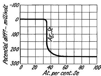
FIG. 36.—Potential Difference in the Cell: \text{Ag} | \frac{1}{2} \text{N-AgNO}_3 | \text{Ag}_2\text{Se} .
