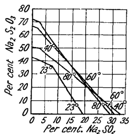
FIG. 117.—Mutual Solubilities of Sodium Sulphate and Thiosulphate.
