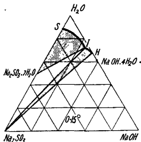
FIG. 62.—Equilibrium in the Ternary System: Na 2 SO 3 -NaOH-H 2 O at 0.15^\circ .
