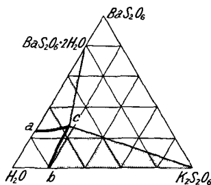
FIG. 134.—Ternary System : \text{K}_2\text{S}_2\text{O}_6 - \text{BaS}_2\text{O}_6 - \text{H}_2\text{O} , at 30°.
