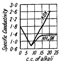
FIG. 58.—The Effect of the Progressive Addition of Alkali on the Conductivity of Sulphurous Acid.
