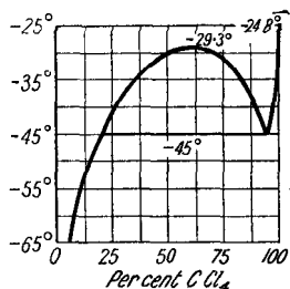
FIG. 52.—The Binary System : \text{SO}_2\text{-CCl}_4 .
