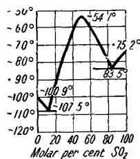
FIG. 146.—Freezing-point Curve of the System: \text{Cl}_2 - \text{SO}_2 (with catalyst).
