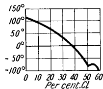
FIG. 139.—Solubility of Sulphur in Sulphur Monochloride.
