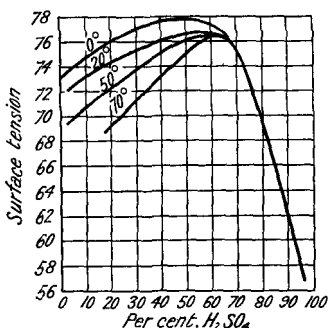
FIG. 86.—The Surface Tension of Sulphuric Acid.
