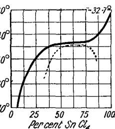
FIG. 53.—The Binary System : \text{SO}_2\text{-SnCl}_4 .
