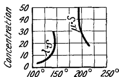
FIG. 7.—Solubility of \lambda - and \mu -Sulphur in Triphenylmethane.
