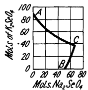
FIG. 56.—Mutual Solubilities of Sodium and Potassium Selenates.
