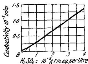
FIG. 98.—Conductivity of Dilute Sulphuric Acid.
