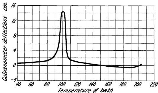
FIG. 4.—Showing the Temperature of Selenium when Heated in a Bath at Different Temperatures.
