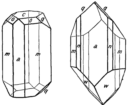
FIG. 13.—Forms of Crystals of Monoclinic or \beta -Sulphur.
