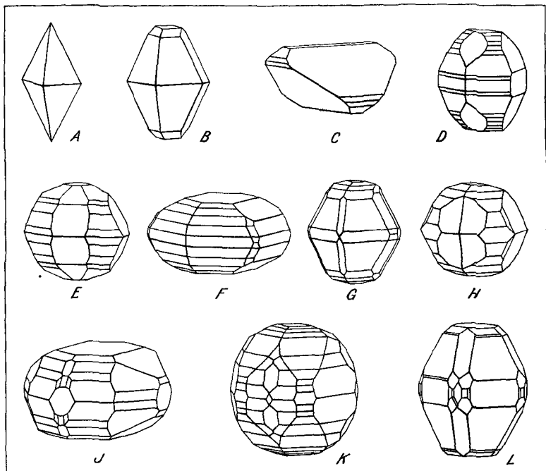
FIG. 11.—Forms of Crystals of Rhombic or \alpha -Sulphur.
