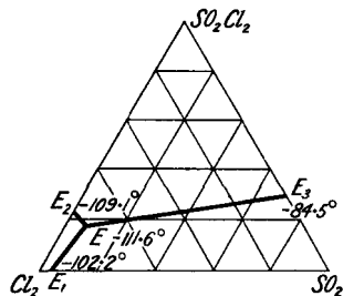
FIG. 149.—Freezing Points of the Ternary System: \text{SO}_2\text{Cl}_2 - \text{Cl}_2 - \text{SO}_2 .
