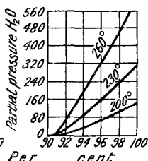
FIG. 92.—Partial Pressure of Water Vapour over Sulphuric Acid.
