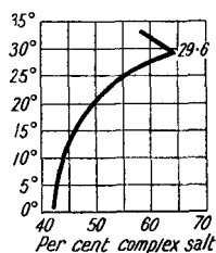
FIG. 127.—Solubility of \text{Na}_2\text{Ca}(\text{S}_2\text{O}_3)_2(\text{NO}_3) .
