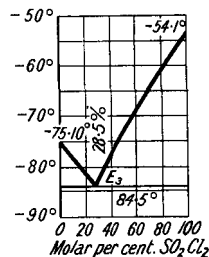
FIG. 148.—Freezing-point Curve of the System: \text{SO}_2 - \text{SO}_2\text{Cl}_2 .
