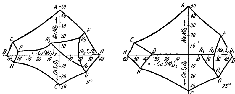
Figs. 125 and 126.—Equilibria in the System: \text{CaS}_2\text{O}_3 + 2\text{NaNO}_3 \rightleftharpoons \text{Na}_2\text{S}_2\text{O}_3 + \text{Ca}(\text{NO}_3)_2 , at 9^\circ and 25^\circ .
