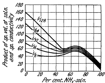
FIG. 49.—Progressive Addition of Ammonia to Solutions of Selenious Acid.
