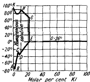
FIG. 151.—The Binary System: \text{KI}-\text{SO}_2 .
