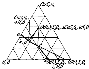
FIG. 128.—The Ternary System: \text{CuS}_2\text{O}_6\text{-(NH}_4)_2\text{S}_2\text{O}_6\text{-H}_2\text{O} , at 30^\circ (Diagrammatic).
