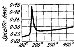
FIG. 22.—Specific Heat of Liquid Sulphur.
