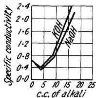
FIG. 51.—Effect of the Progressive Addition of Solution of Alkali on the Specific Conductivity.
