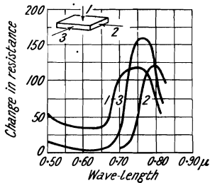
FIG. 24.—The Directive Effect of Light on the Light Sensitivity of Selenium Crystal.
