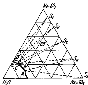
FIGS. 65 and 66.—The Ternary System: \text{Na}_2\text{SO}_3-\text{Na}_2\text{SO}_4-\text{H}_2\text{O} .
