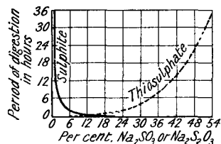
FIG. 108.—Progress of the Conversion of Sulphite to Thiosulphate.
