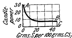
FIG. 26. — Equilibrium Curve of Amorphous Sulphur, Solution, and Vapour.
