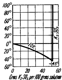
FIG. 67.—Solubility Curves of Potassium Sulphite.
