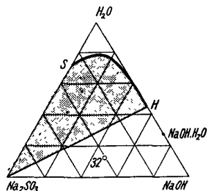
FIG. 63.—Equilibrium in the Ternary System: Na 2 SO 3 -NaOH-H 2 O at 32^\circ .
