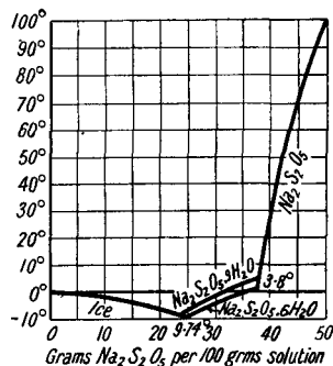
FIG. 68.—Solubility of Sodium Pyrosulphite.
