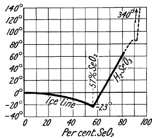
FIG. 47.—Solubility Curve of Selenium Dioxide in Water.
