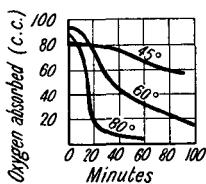
FIG. 42.—The Effect of Temperature on the Decomposition of Neutral Aqueous Solutions of Sodium Hyposulphite.
