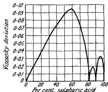
FIG. 85.—Viscosity-Deviations of Sulphuric Acid from Mixture Rule.
