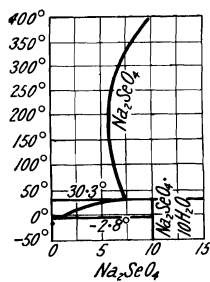
FIG. 54.—High Temperature Solubility of Sodium Selenate.
