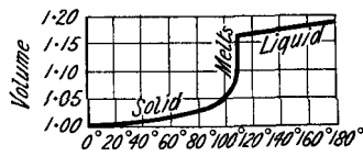
FIG. 15.—Volume Changes on Heating from 0° to 180°.
