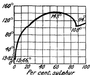
FIG. 33.—Freezing-point Curve of Sulphur and \beta\beta' -dichlorodiethylsulphide.
