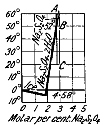
FIG. 43.—Solubility of Sodium Hyposulphite.
