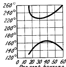
Fig. 34.—Reciprocal Solubility of Sulphur and Benzene.
