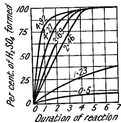
FIG. 79.—The Effect of Nitrogen Peroxide on the Rate of Oxidation of Sulphur Dioxide.
