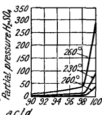
FIG. 93.—Partial Pressure of Acid over Sulphuric Acid.
