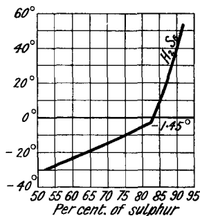
FIG. 41.—Solubility of Sulphur in Hydrogen Persulphide.
