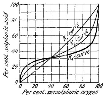
FIG. 102.—Relations between the Concentrations of Sulphuric Acid and the Persulphuric Acids.
