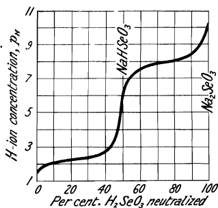
FIG. 48.—The H-ion Concentration during the Neutralization of Selenious Acid with Sodium Hydroxide.
