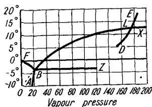
FIG. 47.—The Binary System: \text{SO}_2\text{-H}_2\text{O} (Diagrammatic).
