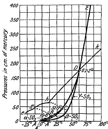
FIG. 76.—The Vapour Pressure Curves of Sulphur Trioxide.
