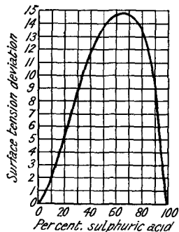
FIG. 88.—Surface Tension Deviations of Sulphuric Acid from the Mixture Rule.
