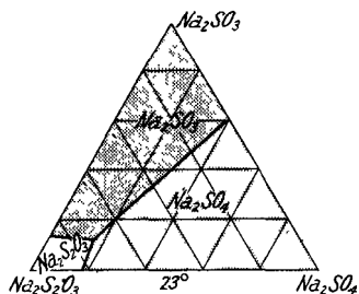
FIG. 119.—The Ternary System : \text{Na}_2\text{SO}_3 - \text{Na}_2\text{SO}_4 - \text{Na}_2\text{S}_2\text{O}_3 in Aqueous Solution at 23°.
