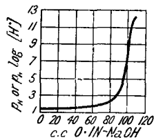
FIG. 99.—Electrometric Titration Curve of Sulphuric Acid.
