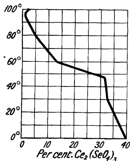
FIG. 61.—Solubility of Cerous Selenate in Water.
