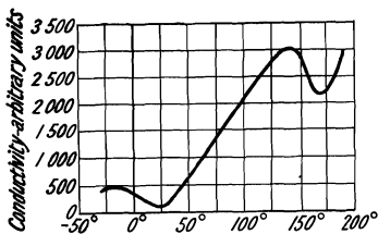
FIG. 13.—Temperature-Conductivity Curve.
