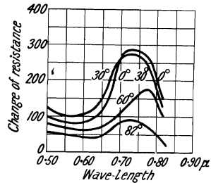
FIG. 25.—The Effect of Polarized Light at Different Angles on the Light Sensitivity of Selenium.
