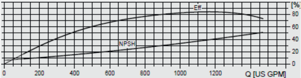
Efficiency curves for the Grundfos submersible pump type 1100S. The pump's nameplate typically notes the pump's flow at best efficiency. Another number typically refers to the number of bowls and thereby how much pressure the pump can produce.
