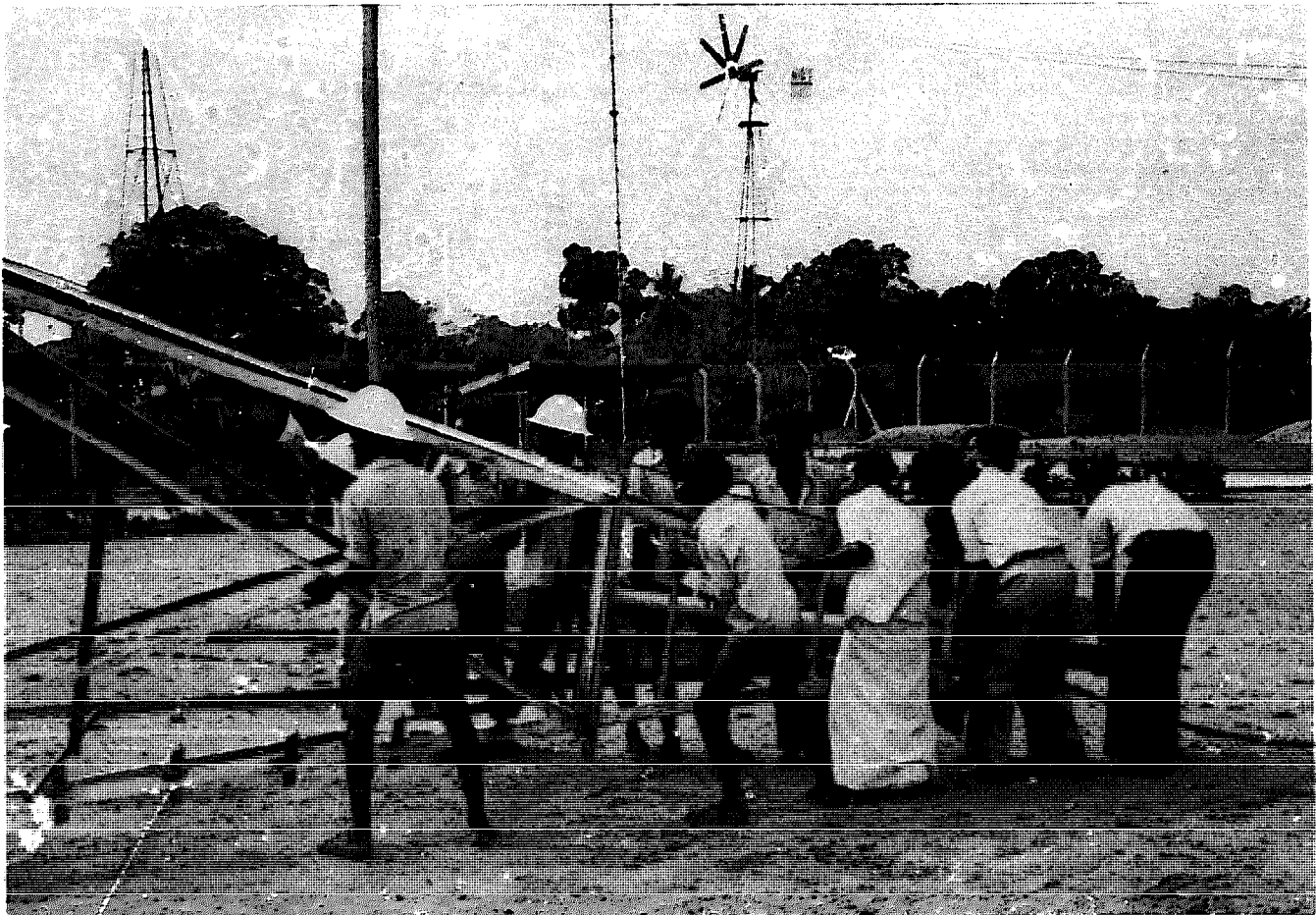
The installation of a 2.5 m windmill in Colombo, Sri Lanka, in the background the 2.2 m WEU windmill.
