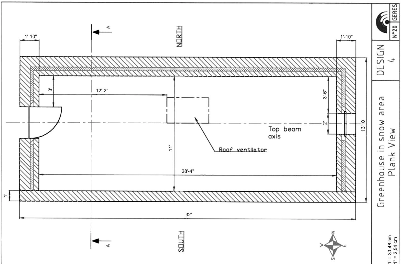
Figure 16 - Design 4 - Greenhouse in snowy areas
