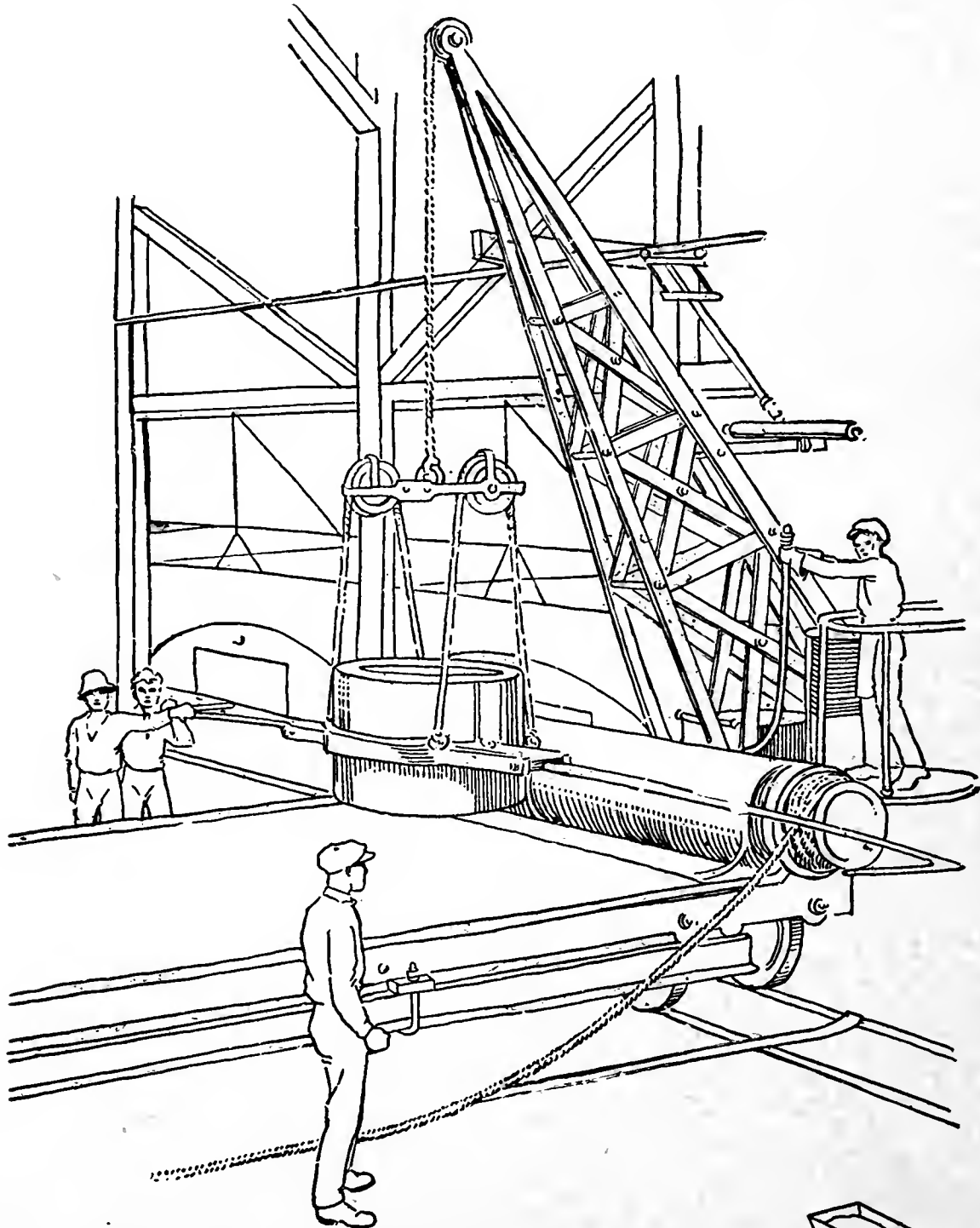
FIG. 24 ROLLING PLATE GLASS
