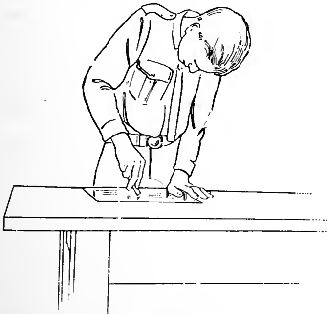
FIG. 87 BORING A HOLE IN GLASS
